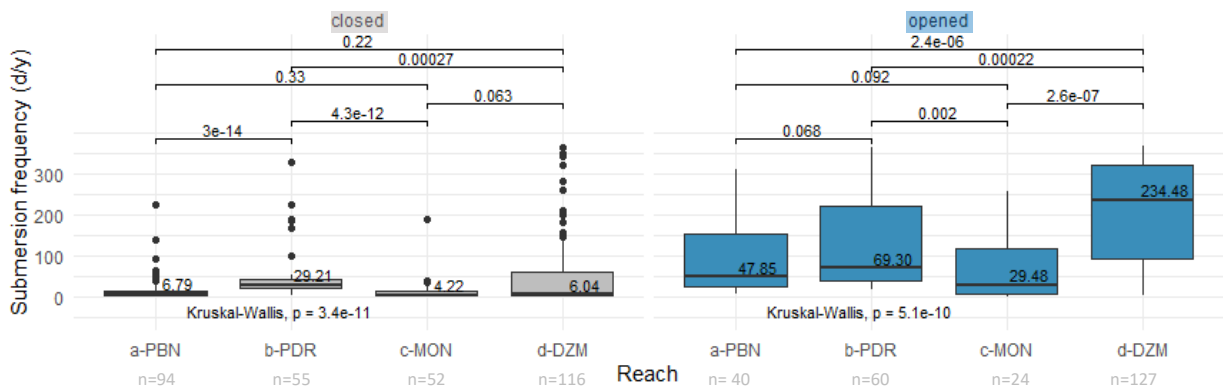
Figure 98 : Submersion frequency of dike structures according to the reach
