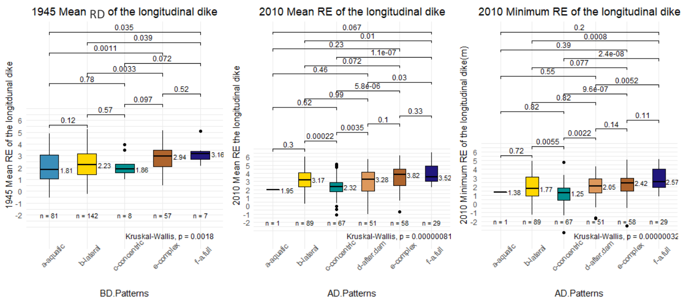
Figure 92: Before/after diversion longitudinal dike parameters (closed fields)
