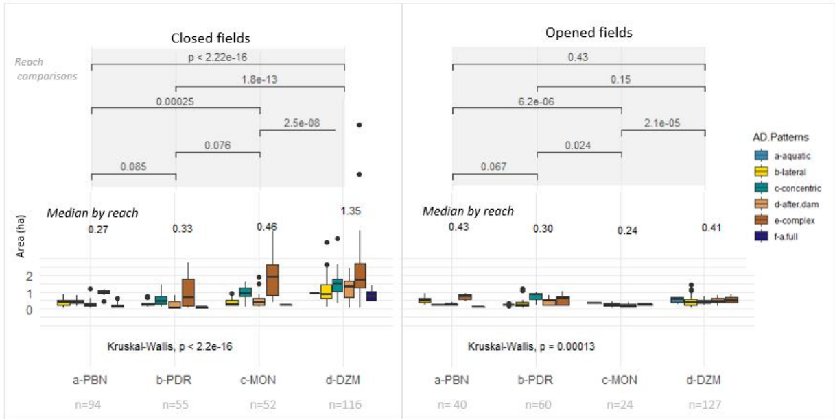
Figure 97: Dike field extent according to reach and structure types
