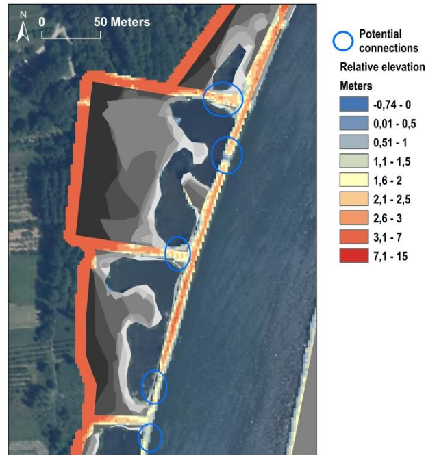
Figure 108 : Low spots, breaches in the dykes like hydrological connection points (Lidar DEM data)
