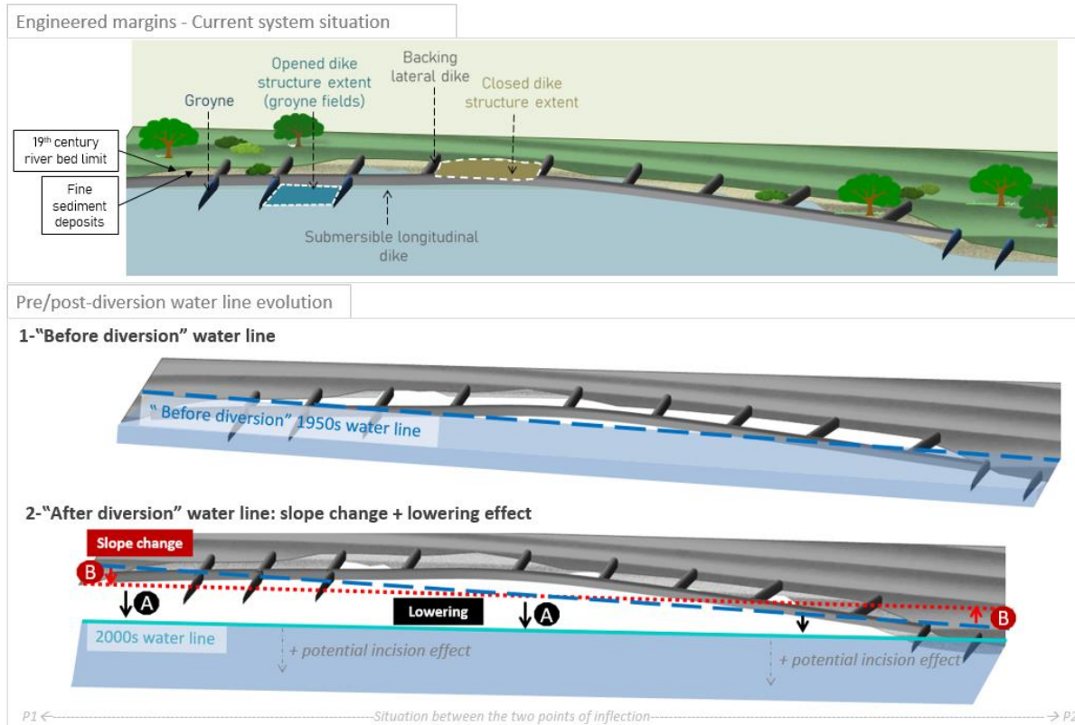
Figure 107 : Water line changes occurred by diversion
