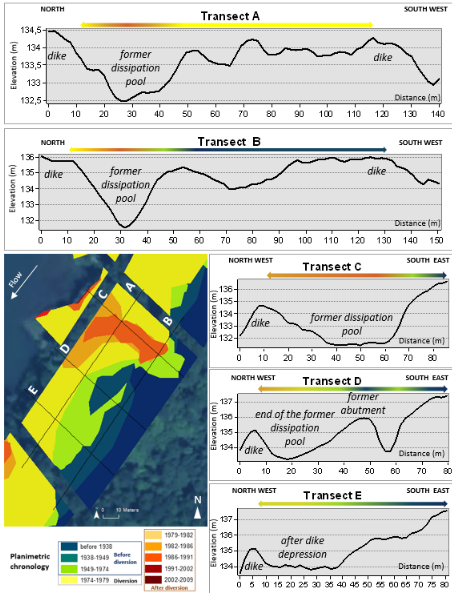
Figure 81 : Correspondence between planimetric patterns and topography of structures (coloured arrows correspond to the planimetric transect)
