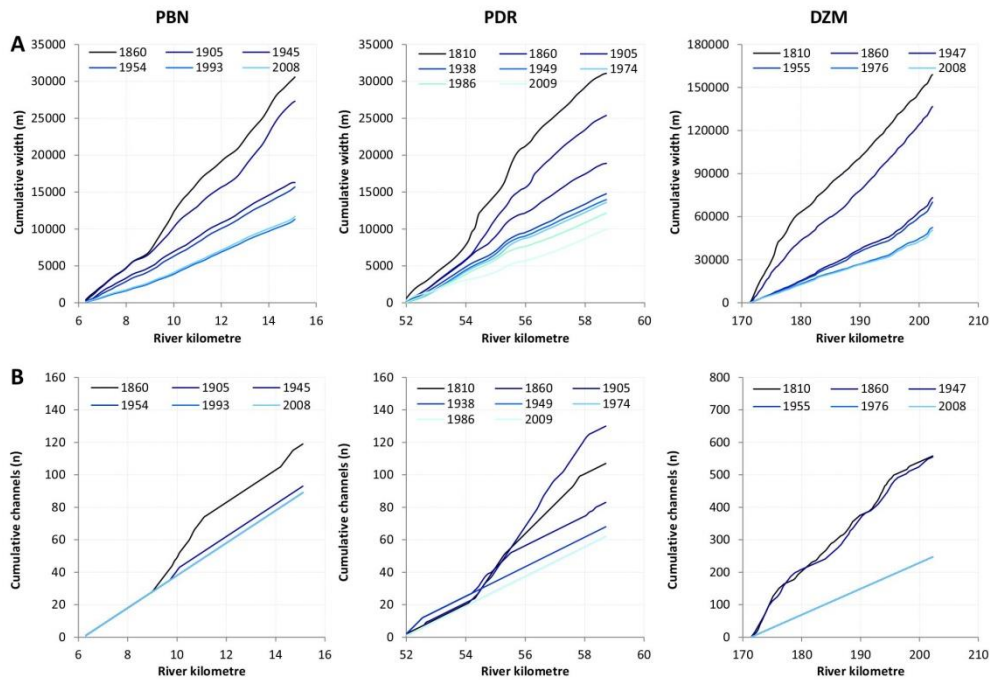
Fig. 7. A. Cumulative average active channel width and B, cumulative number of flowing channels per 100-m-long segment for the different periods for PBN, PDR and, DZM. It should be noted that the size of DZM reach is much larger than PBN and PDR (28, 11.2 and 15.7 km, respectively).
