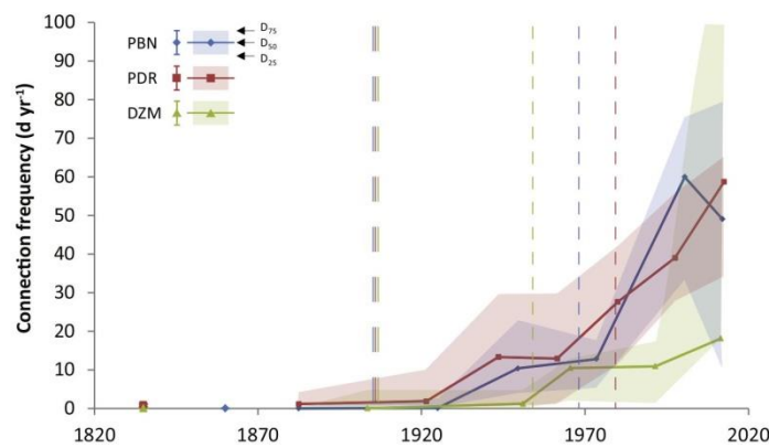
Fig. 11. Median present connection frequency by floodplain terrestrialisation period. Long dashed lines correspond to Girardon structures, and short dashed lines denote channel bypassing trends of each of the sections.
