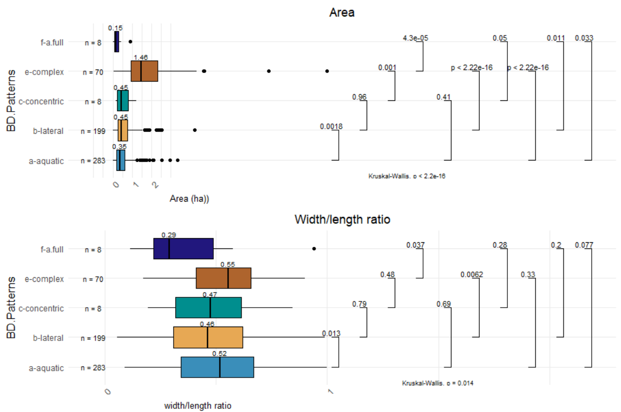
Appendix 5: Dike fields areas and width/length ratio comparisons according to the pattern (before diversion situation)
