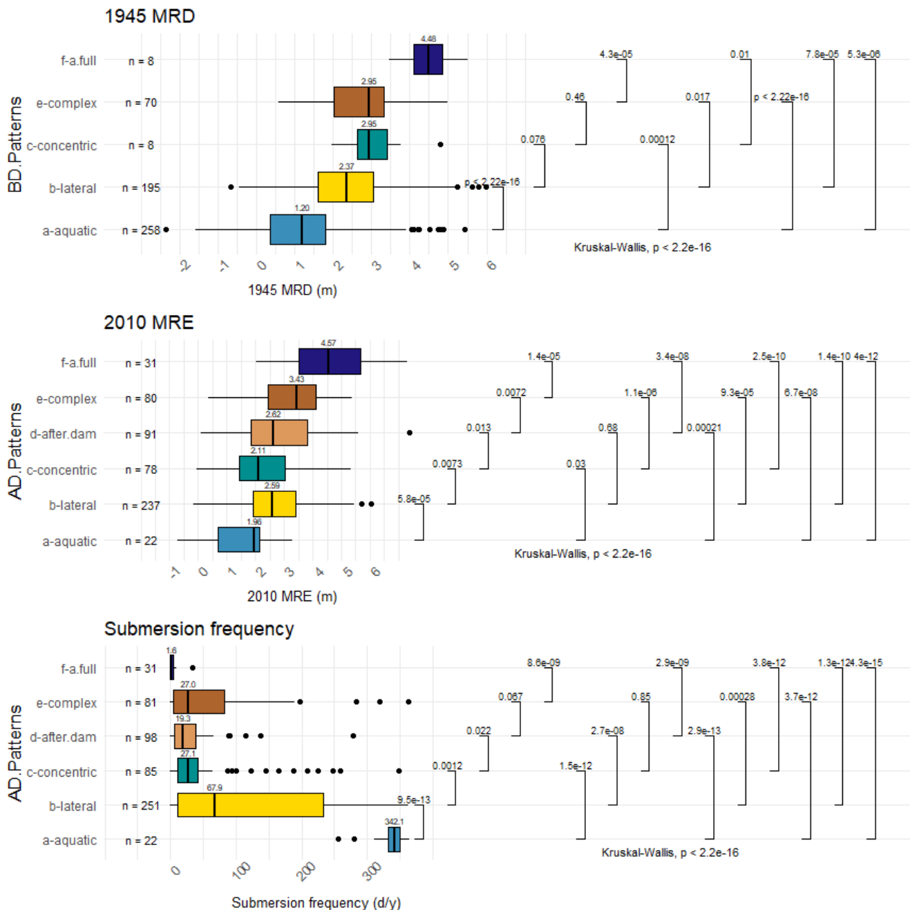
Figure 90 : 1945 MRD, 2010 MRE and submersion frequency according to patterns
