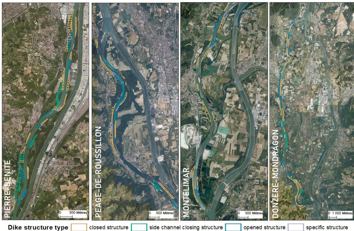
Figure 77 : Distribution of the dike fields on each reach
