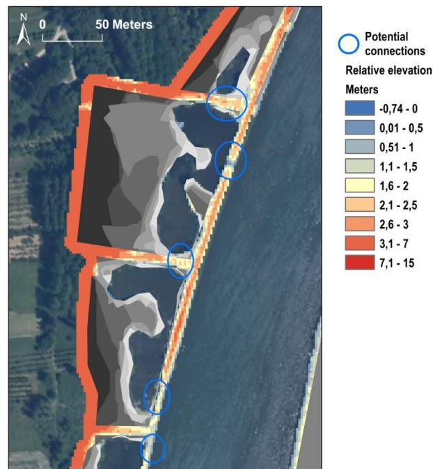
Figure 108 : Low spots, breaches in the dykes like hydrological connection points (Lidar DEM data)
