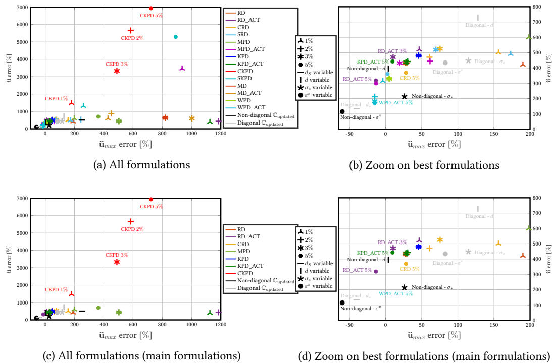
Figure 3.45: Comparison of classical and locally updated damping matrix performances to characterise the experimental accelerations
