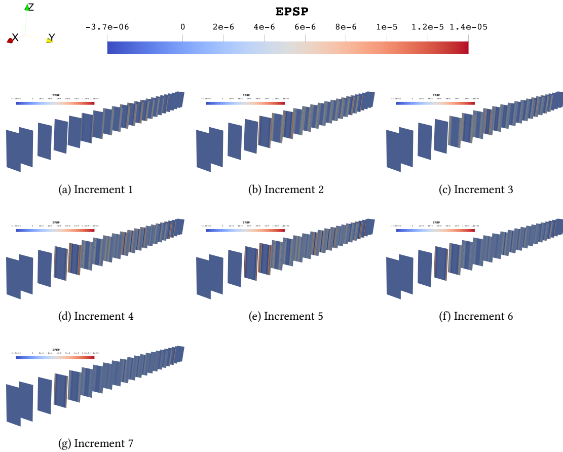
Figure D.5: DSS2 test - Friction deformation variable evolution along the beam - RICBET - RD 2%
