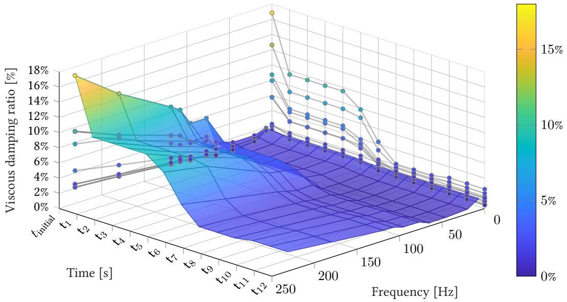
Figure 3.1: Equivalent viscous damping ratios (eq. 3.8) for ten modes over time
