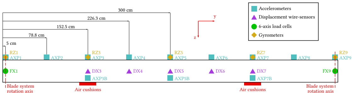
Figure 1.18: Sensor positions (Heitz, 2017)
