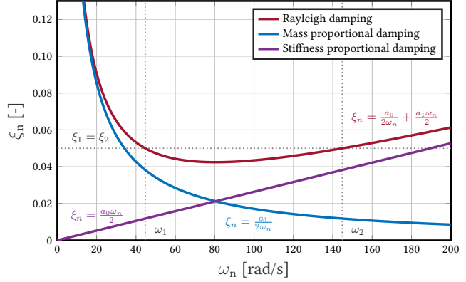
Figure 1.13: Rayleigh equivalent damping for \xi_1 = \xi_2
