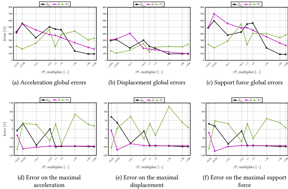
Figure 3.39: Parametric study of function parameters - non-diagonal damping matrix formulation - \mathcal{P}_1 evolution - global responses
