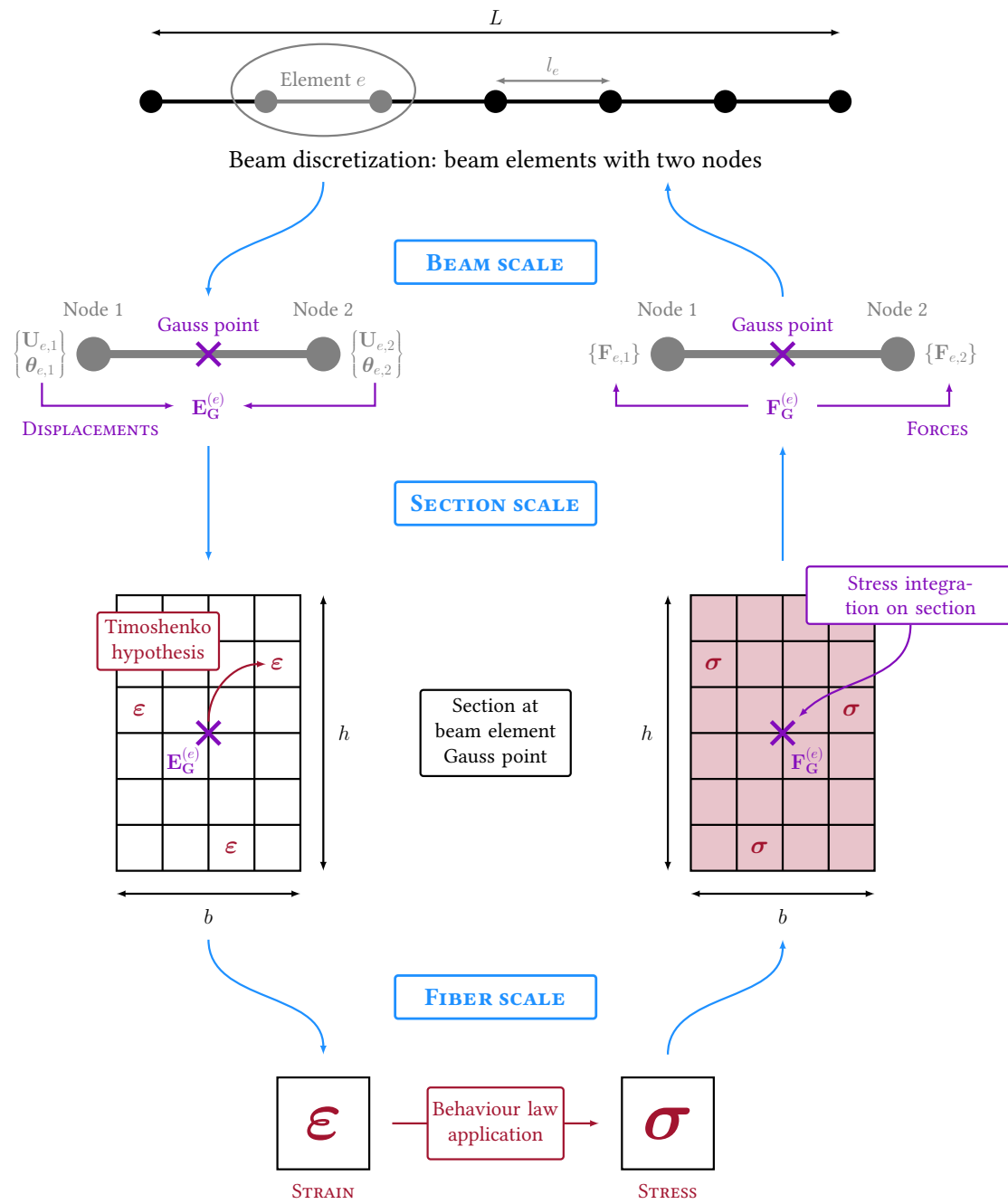
Figure 2.3: Multi-fibre approach algorithm
