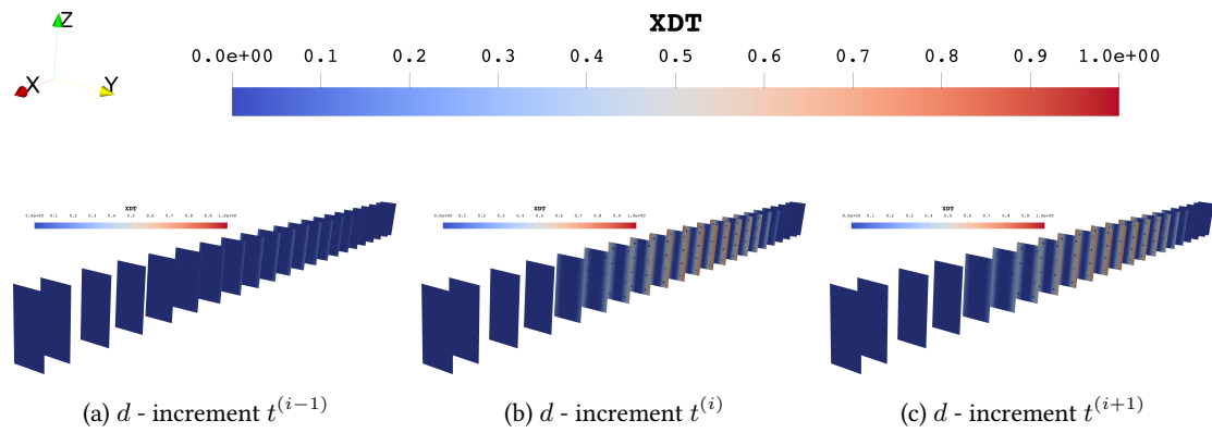
Figure 2.42: DSS2 test - Damage variable evolution along the beam - RICBET - RD 2%
