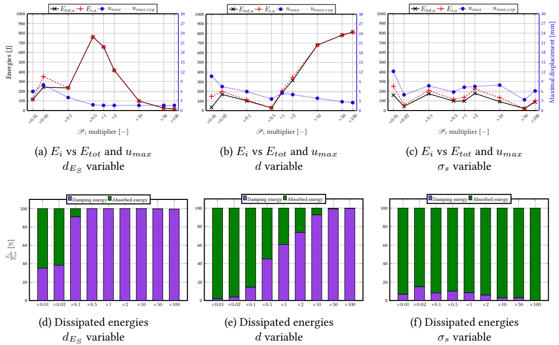
Figure G.6: Parametric study of function parameters - diagonal damping matrix formulation - \mathcal{P}_1 evolution - energy analyses
