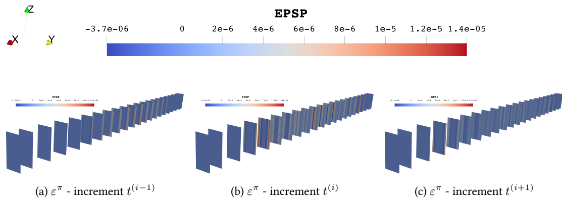
Figure 2.43: DSS2 test - Friction deformation variable evolution along the beam - RICBET - RD 2%
