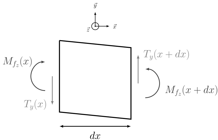
Figure E.1: Equilibrium of a beam section
