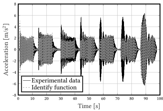
(a) DSS2 test - acceleration
