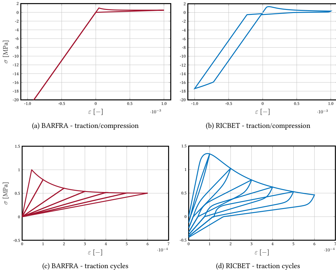
Figure 2.5: Constitutive laws for one concrete element
