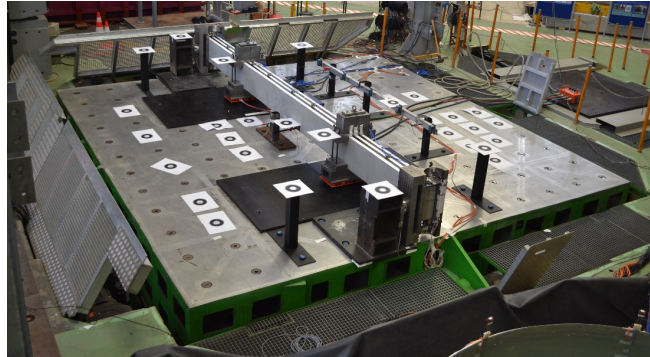
Figure 3: Dynamic experimental setup (Heitz, Le Maout, et al., 2018)
