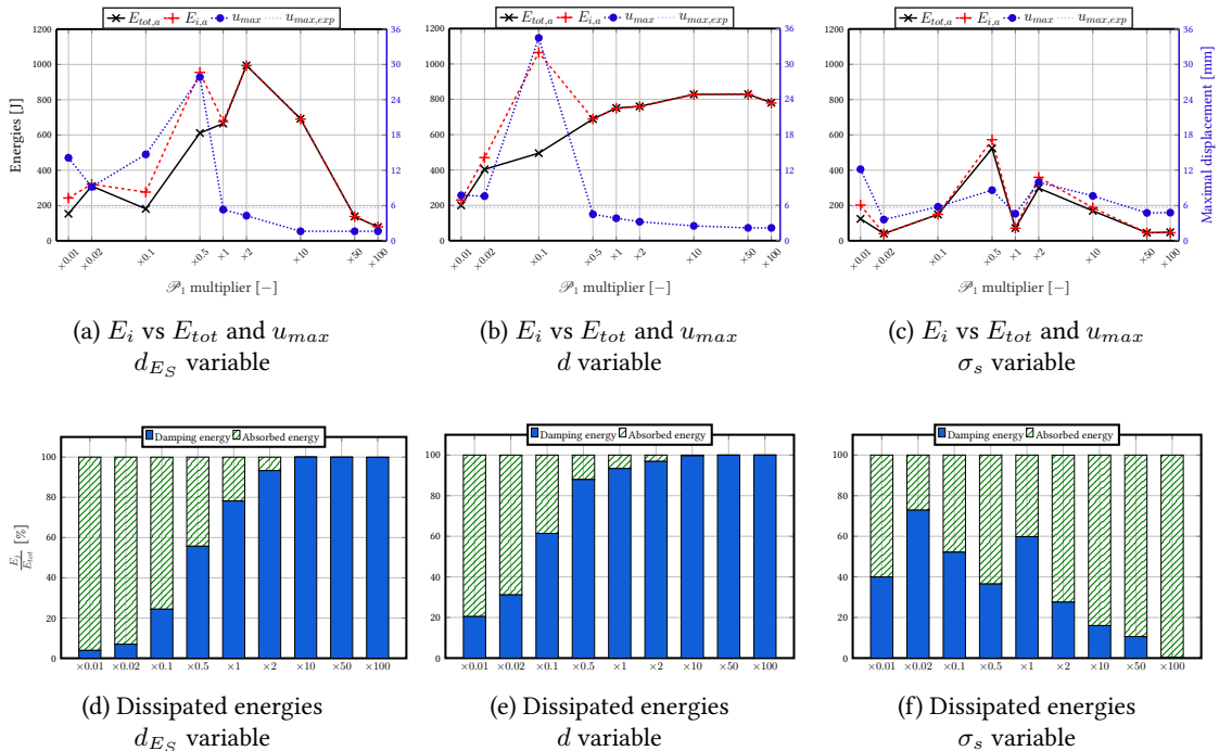
Figure 3.41: Parametric study of function parameters - non-diagonal damping matrix formulation - \mathcal{P}_1 evolution - energy analyses
