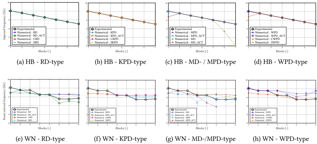
Figure 2.16: DSS2 test - Frequency responses (white-noise signals - WN - and harmonic block signals - HB -) - RICBET 2%
