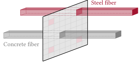
Figure 2.1: One section of the multi-fibre model with one fibre of concrete and one of steel
