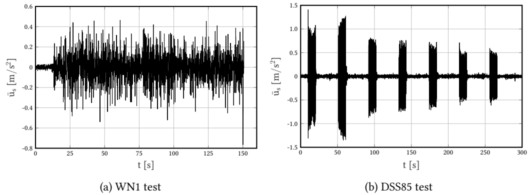
Figure 1.23: Input signals of the two first dynamic tests carried out on HA16-C1A-2 beam
