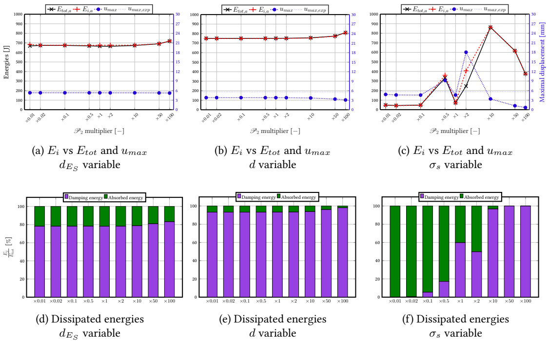
Figure G.3: Parametric study of function parameters - non-diagonal damping matrix formulation - \mathcal{P}_2 evolution - energy analyses
