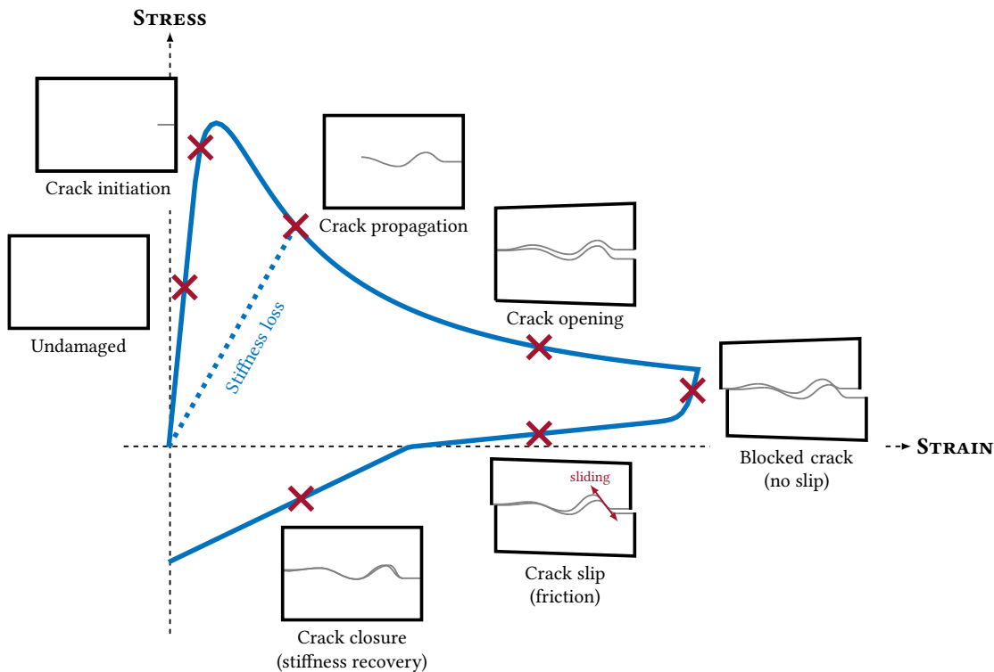
Figure 2.6: Scheme of concrete dissipative phenomena
