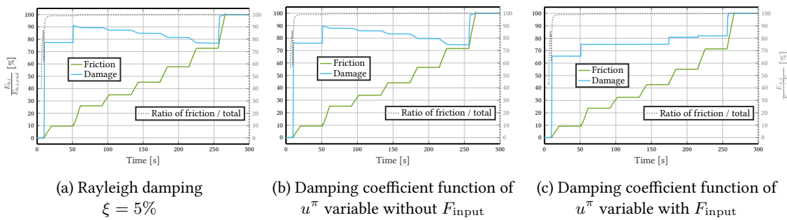
Figure 3.34: DSS2 test with IDEFIX model - Dissipation proportions at the material level - proposed damping models depending on internal variables
