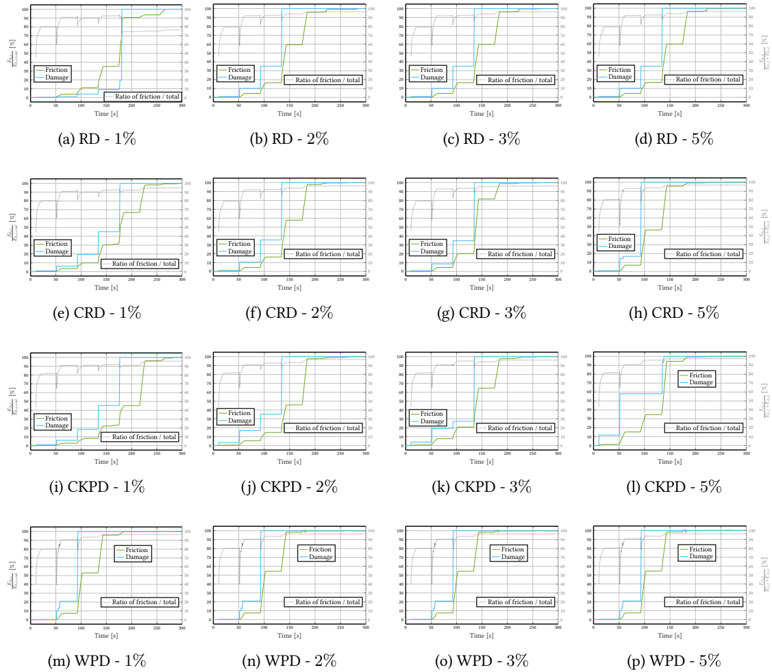
Figure C.2: DSS2 test - Dissipation proportions at material level - RICBET - damping ratio influence
