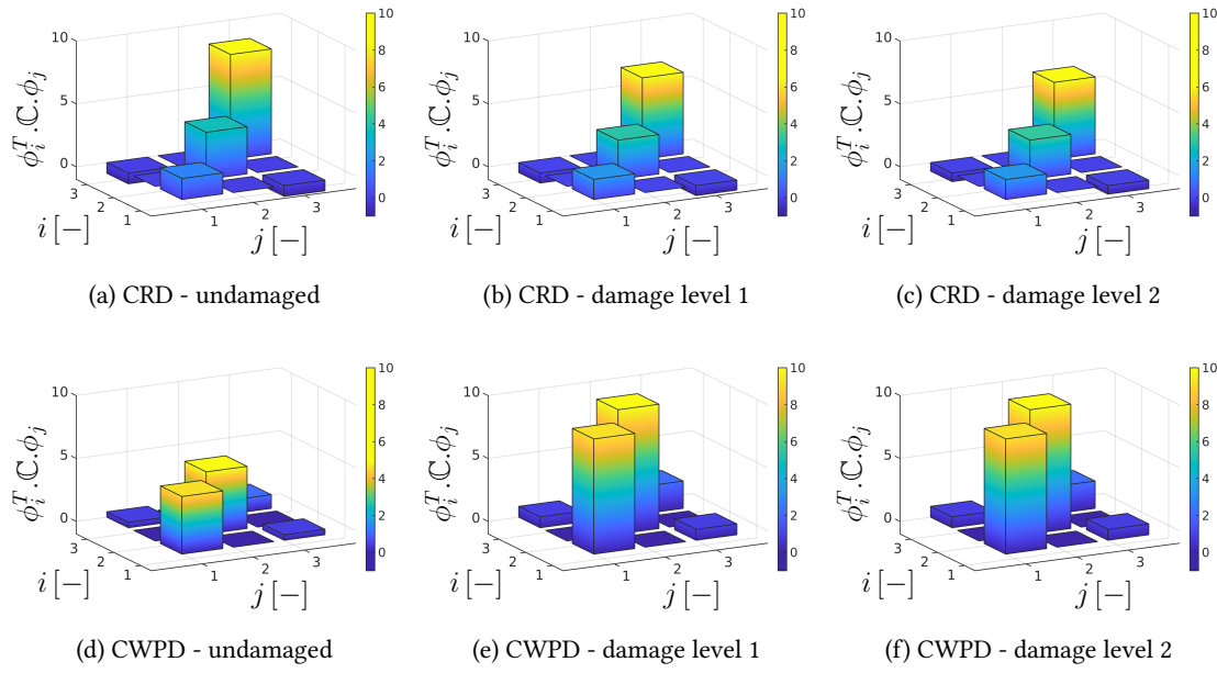
Figure 3.3: Projection of the damping matrix on the undamaged eigenbasis - DSS2 test - RICBET - 2%
