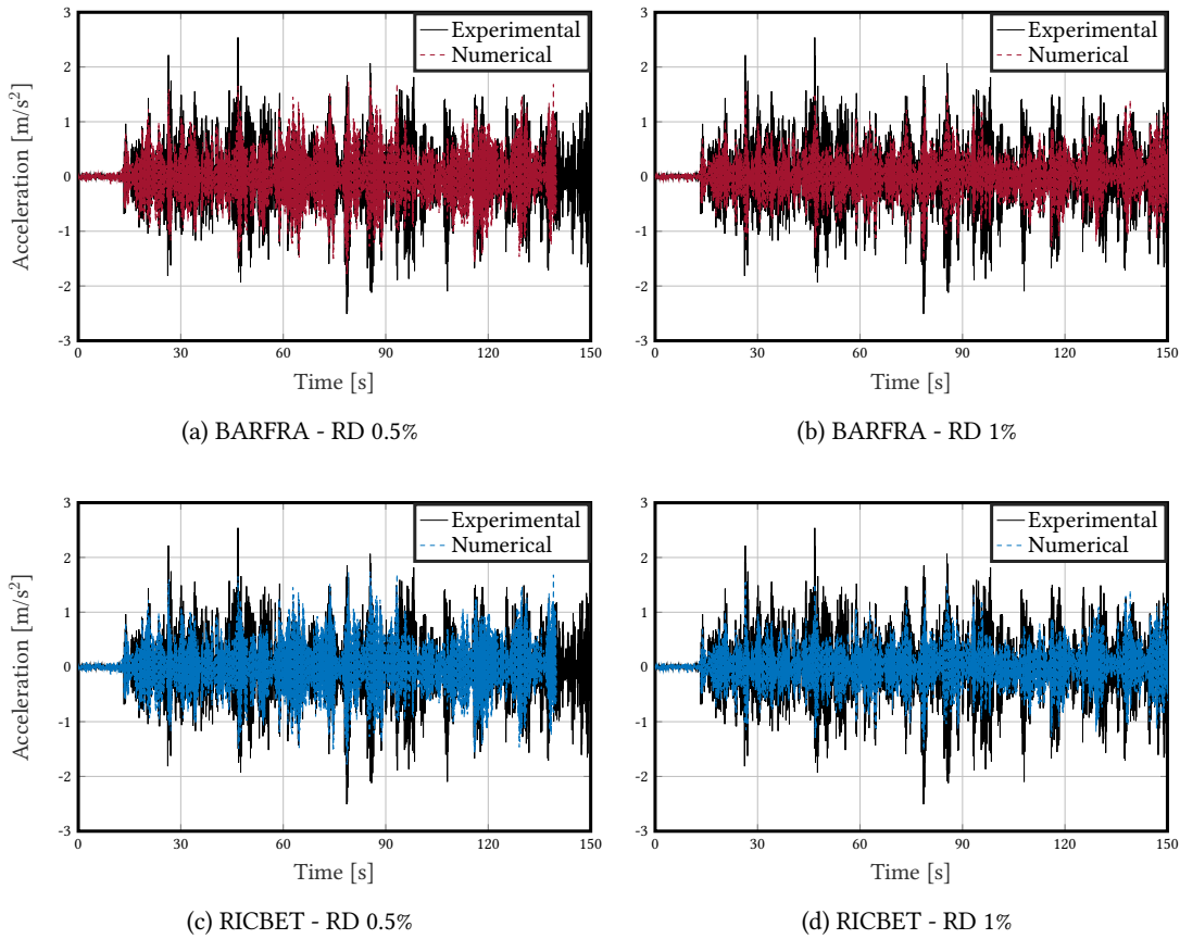
Figure 2.11: WN1 test - Acceleration responses
