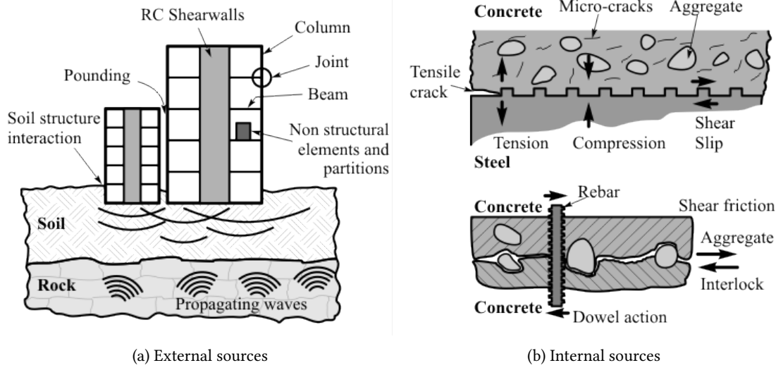
Figure 1.5: Schemes summarising the damping sources (Jehel, 2009)
