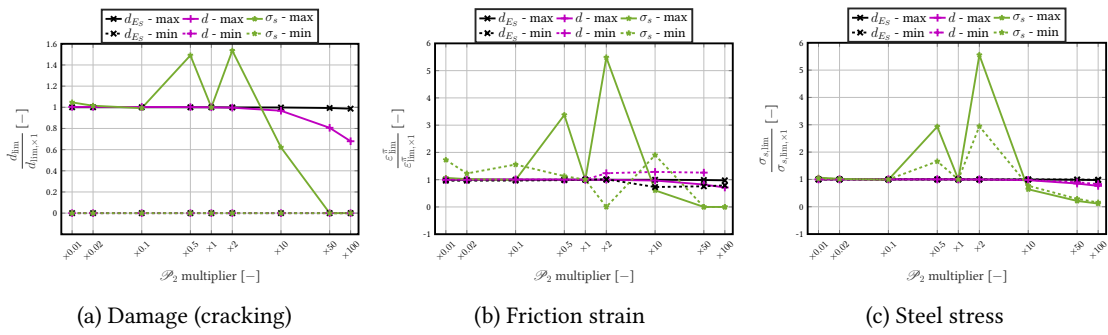
Figure G.2: Parametric study of function parameters - non-diagonal damping matrix formulation - \mathcal{P}_2 evolution - normalized maximal and minimal values of some variables
