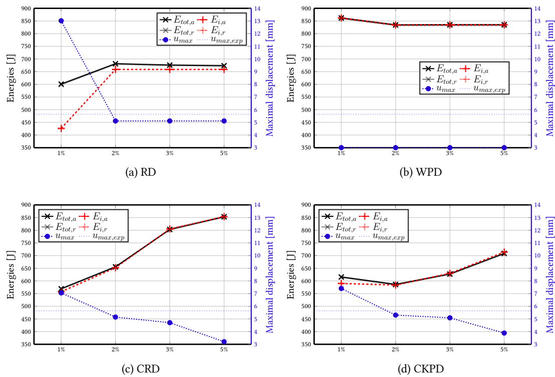
Figure 2.33: DSS2 test - Imparted and total energies in parallel to the maximal displacement - RICBET - \xi influence
