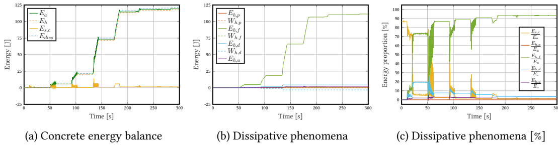
Figure 2.38: DSS2 test - Concrete energy analysis - RICBET - RD 2%
