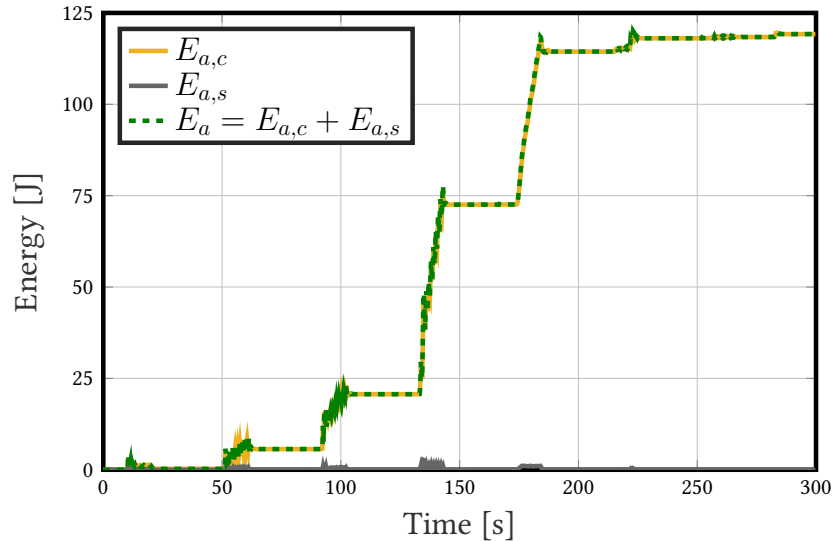
Figure 2.24: DSS2 test - Total absorbed energy decomposition between steel and concrete
