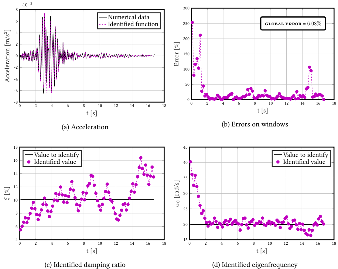
Figure 3.14: Validation of the damping identification method on a three simple DOFs system
