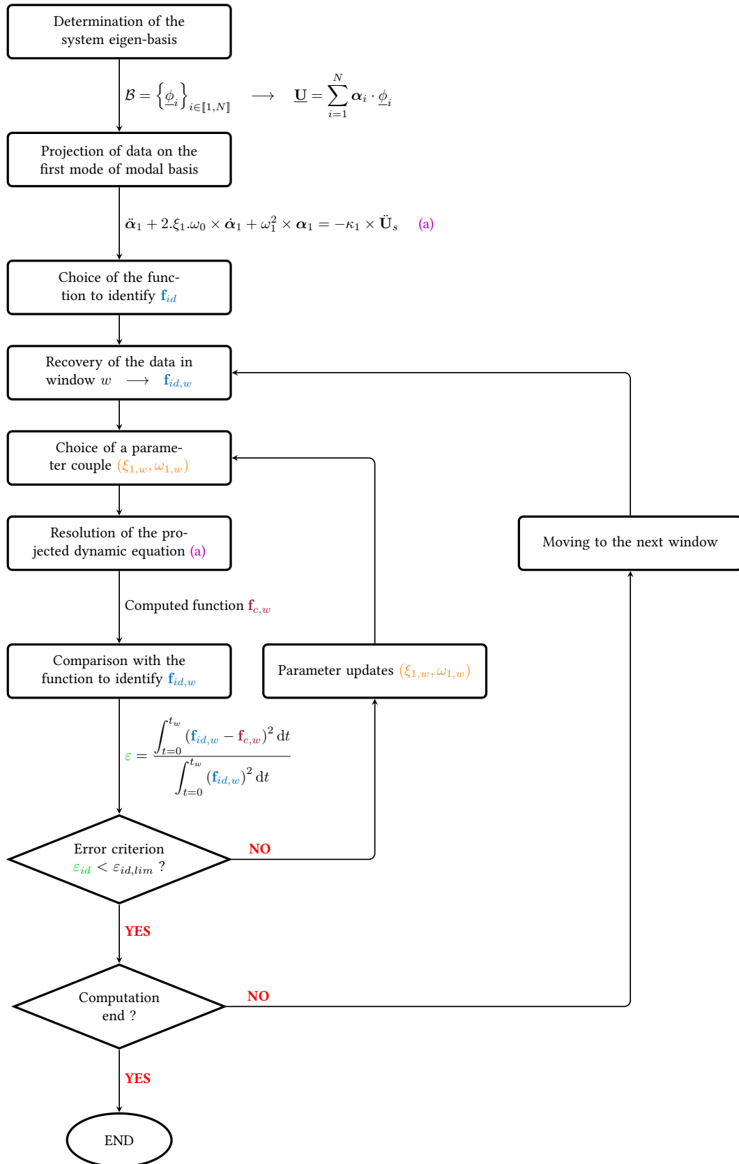
Figure 3.10: Algorithm of the damping identification method
