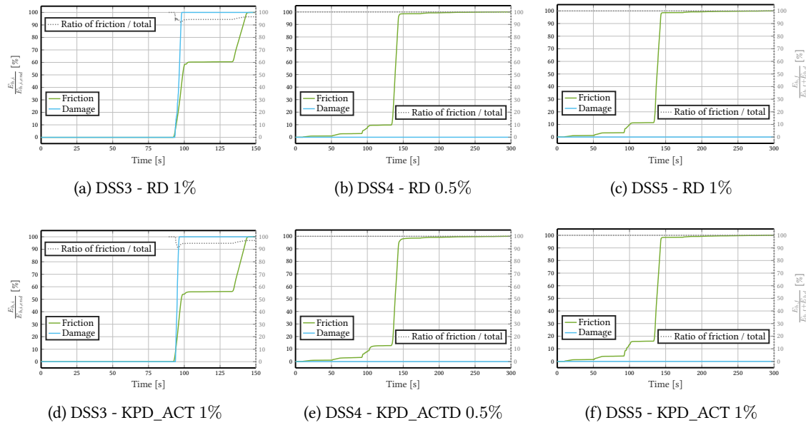
Figure 2.41: DSS3 to DSS5 tests - Dissipation proportions at the material level - RICBET
