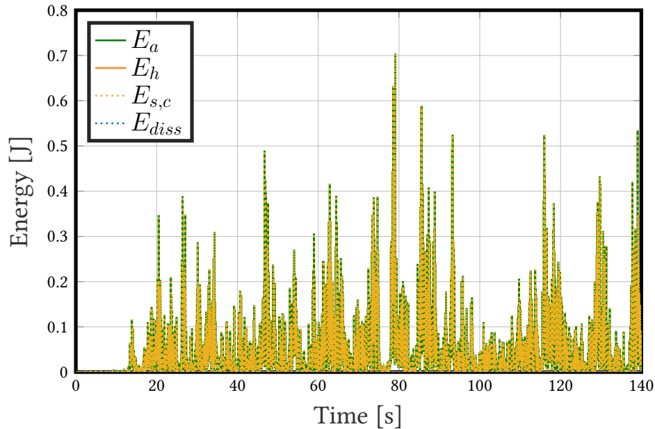
Figure 2.37: WN1 test - Concrete energy balance - RICBET - RD 0.5%
