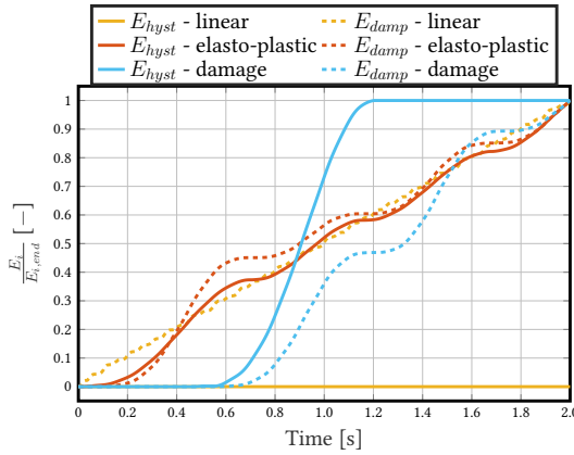
Figure 1.9: Different types of damping - one DOF system - dissipative energies
