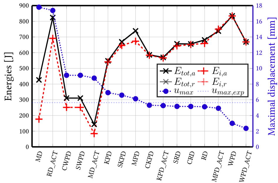
Figure 2.31: DSS2 test - Imparted and total energies in parallel to the maximal displacement - RICBET - 2%
