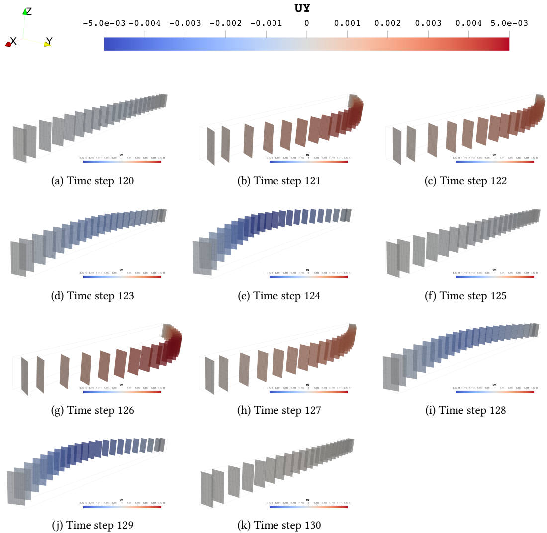
Figure D.1: DSS2 test - increment 4 - Beam displacement [m] - RICBET - RD 2%
