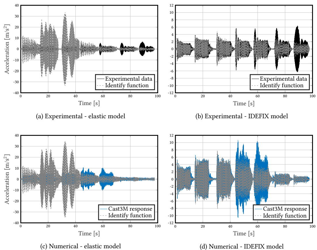
Figure 3.26: DSS2 test (harmonic parts) - Identified accelerations with IDEFIX model
