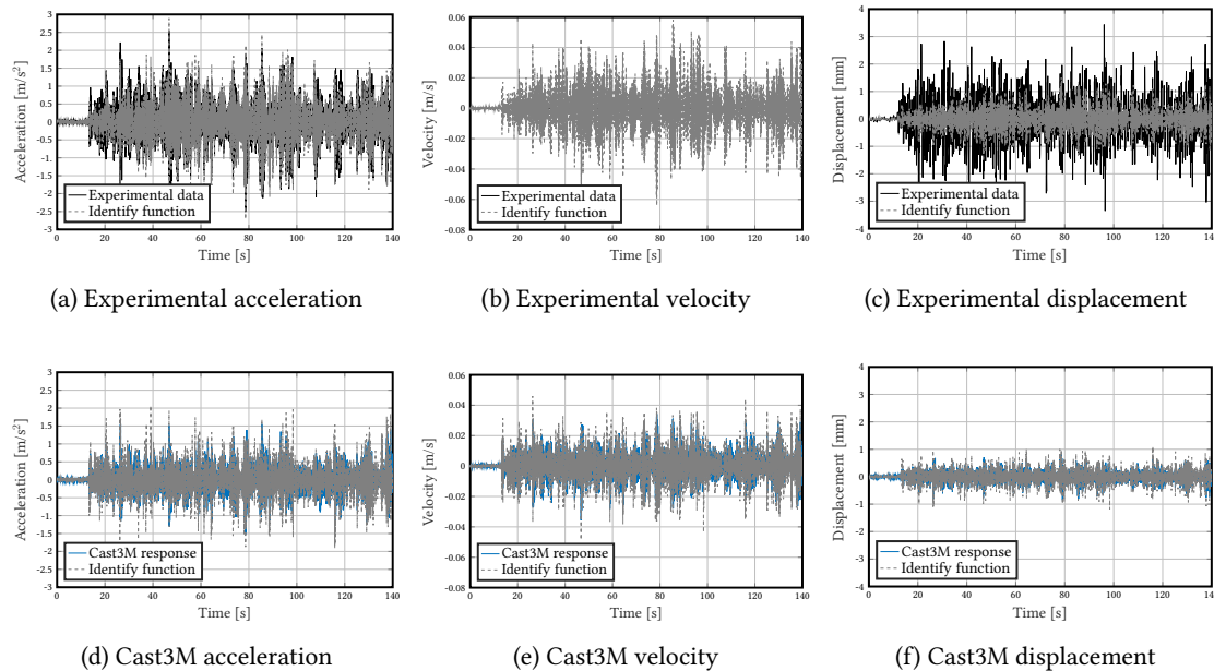
Figure 3.15: WN1 test - Application of the damping identification method on beam responses - global responses
