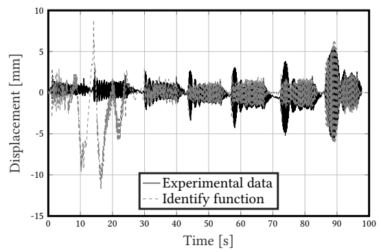
(b) DSS2 test - displacement
