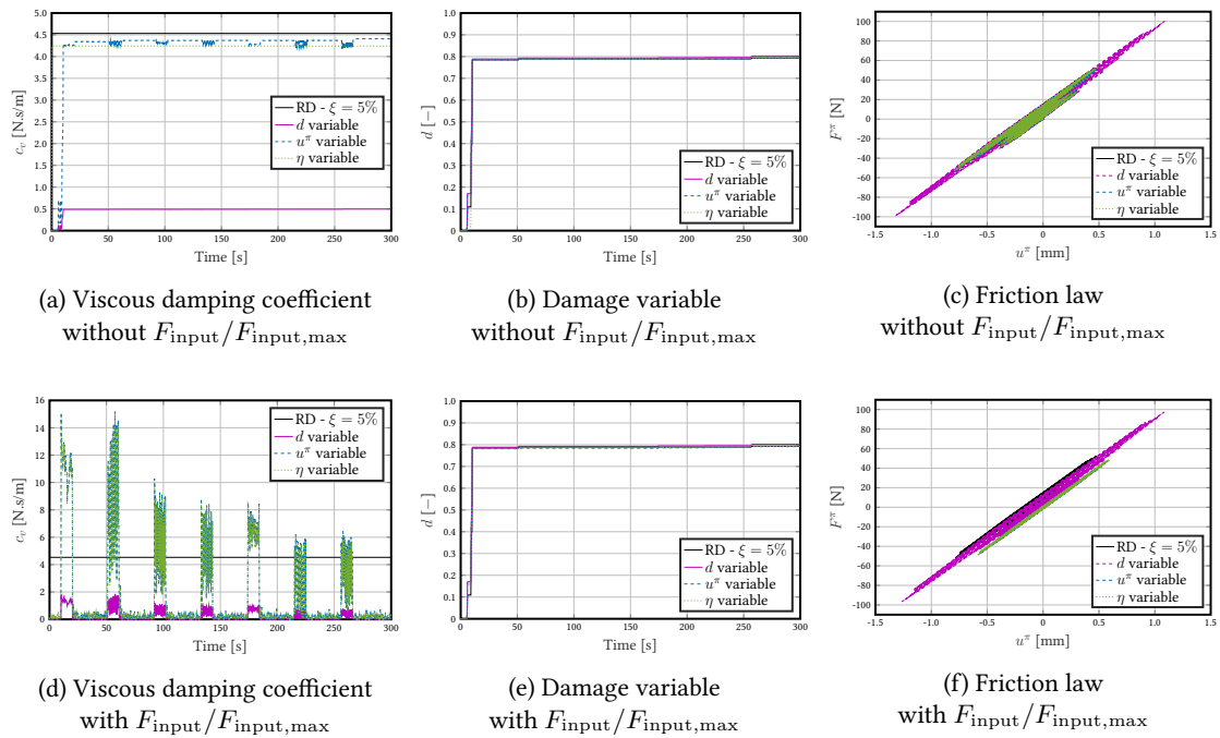
Figure 3.31: DSS2 test with IDEFIX constitutive model - Nonlinear parameters with proposed damping models depending on internal variables
