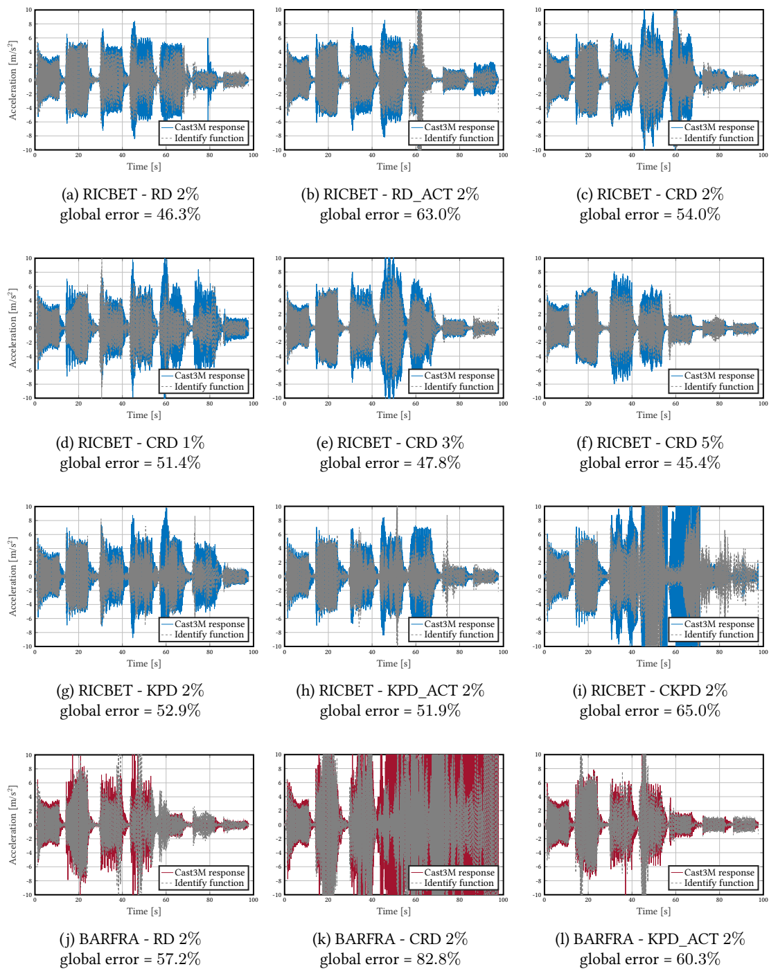
Figure 3.20: DSS2 test (harmonic parts) - Identified accelerations
