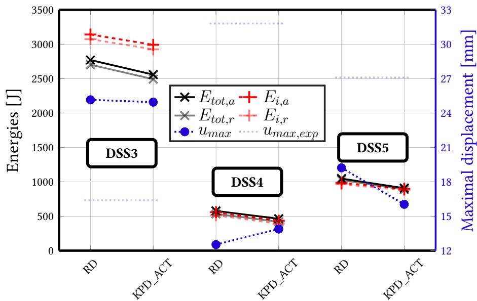
Figure 2.35: DSS3 to DSS5 tests - Imparted and total energies in parallel to the maximal displacement - RICBET
