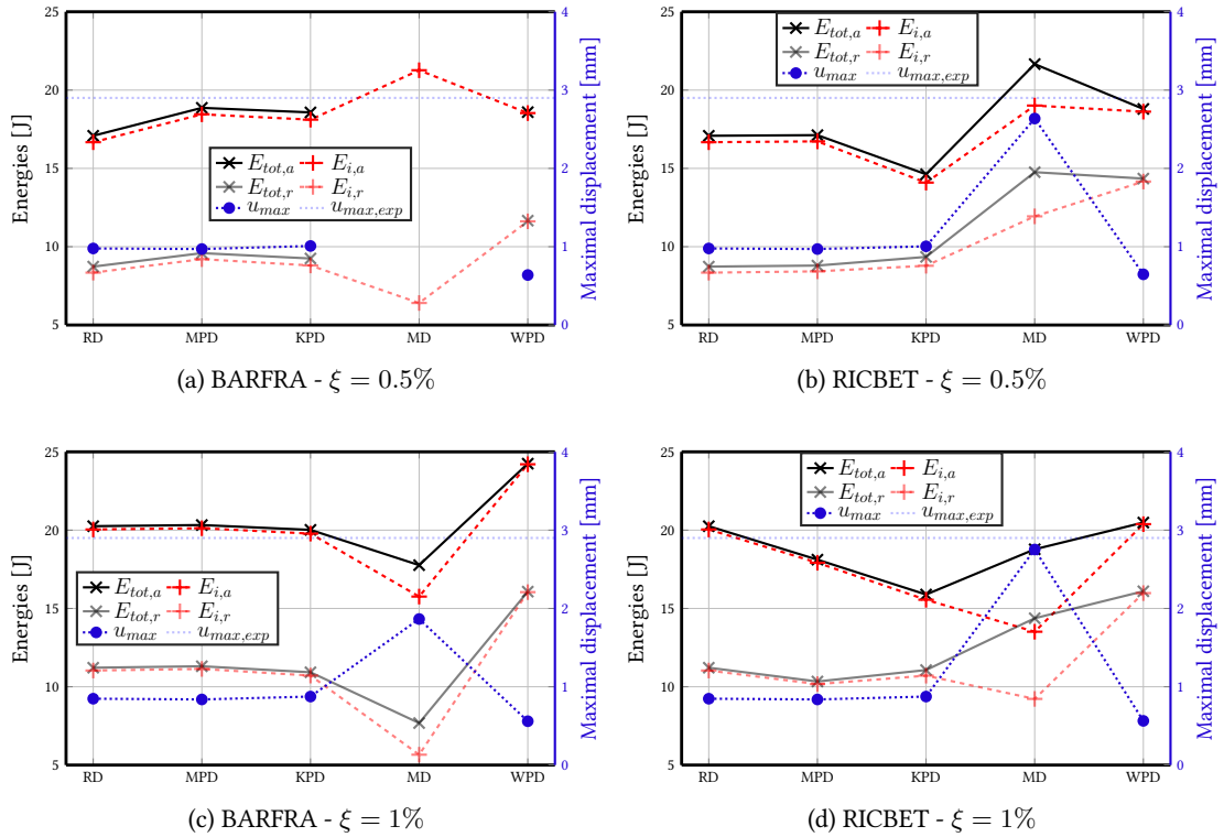
Figure 2.26: WN1 test - Imparted and total energies in parallel to the maximal displacement - absolute energy balance
