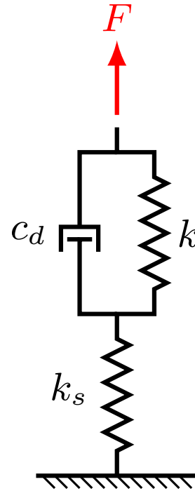
Figure 1.14: Modified hysteretic model (Muravskii, 2004)
