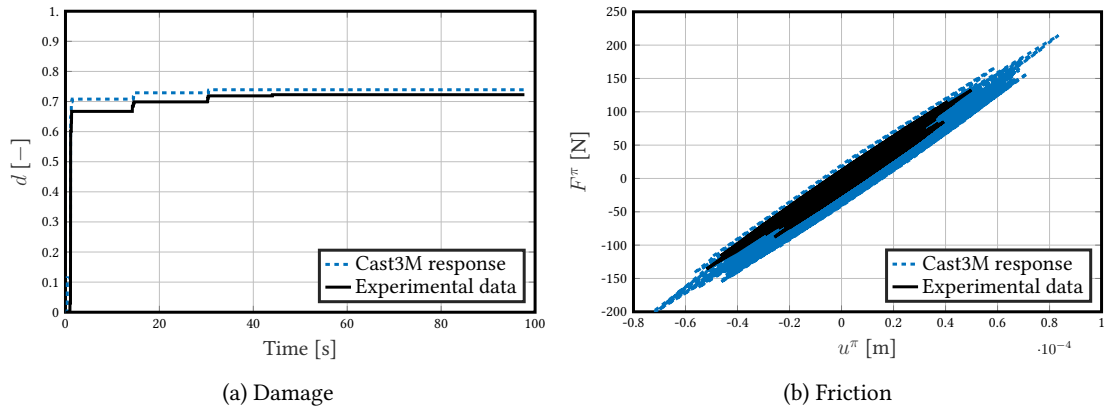
Figure 3.28: DSS2 test (harmonic parts) - Nonlinear parameter evolutions - IDEFIX model
