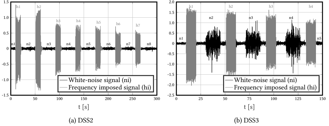
Figure 2.10: Decomposed input signals between harmonic and white-noise parts
