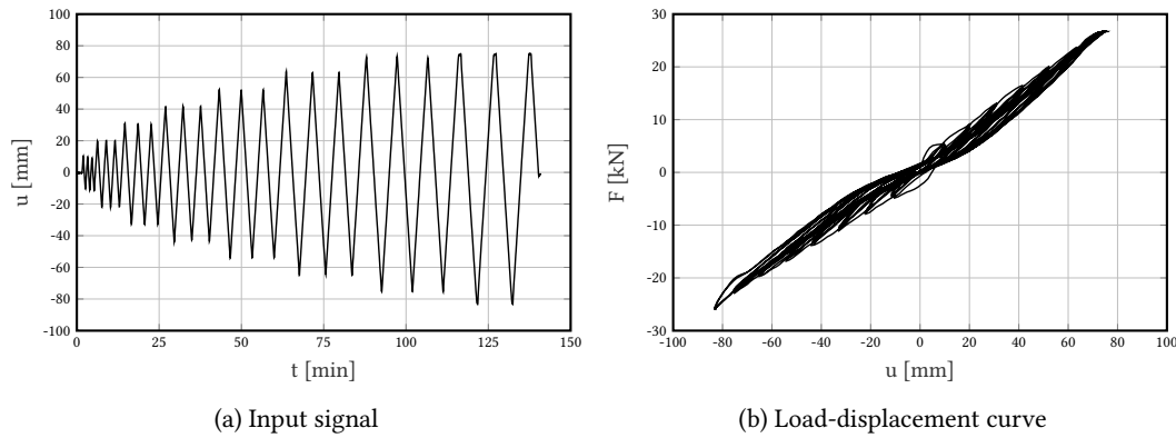
Figure 1.21: QSC1 test on the beam HA16-C1A-1
