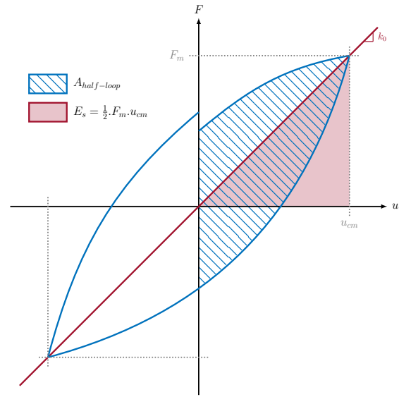
Figure 1.16: Determination of the equivalent viscous damping for a half-cycle (Jacobsen, 1960)
