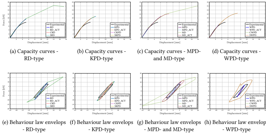
Figure 2.15: DSS2 test - Envelopes of the behaviour responses - (RICBET 2%)
