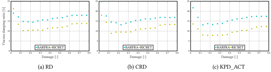
Figure 3.23: DSS2 test (harmonic parts) - Numerical identified evolutions \xi_1(d) - constitutive model influence - 2%
