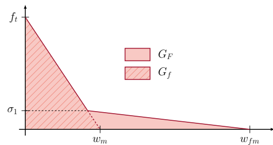
Figure 1.4: Definition of fracture energies
