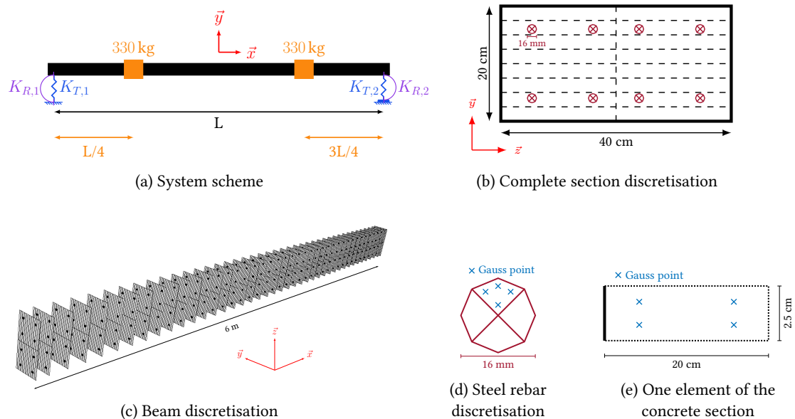
Figure 2.4: Model scheme and discretisation
