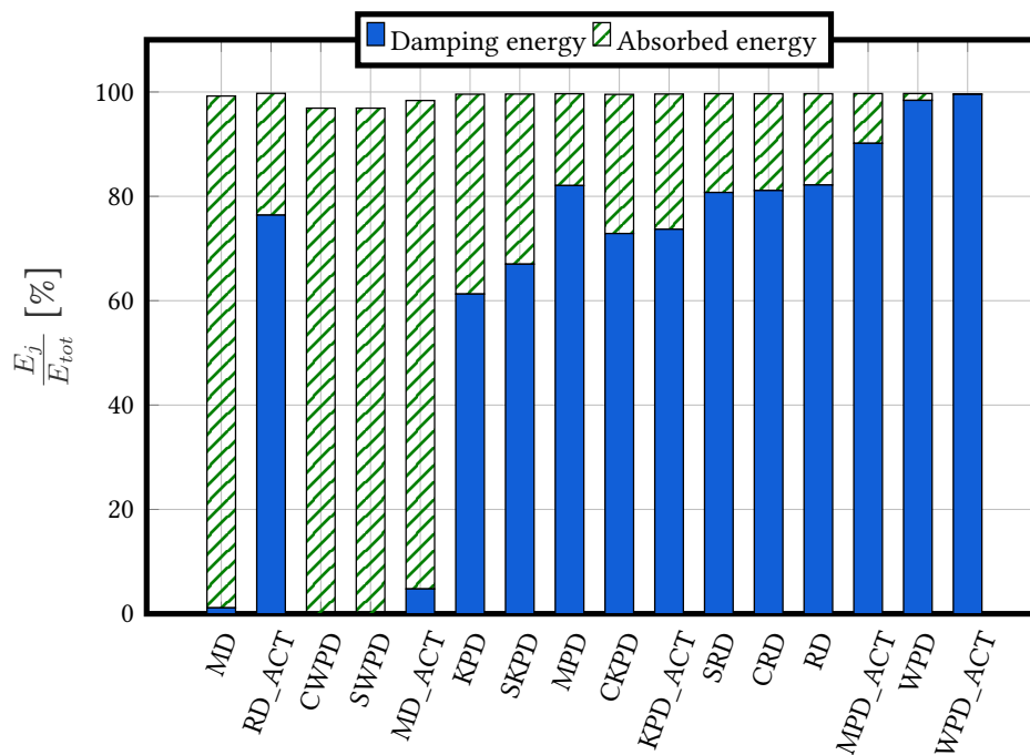
Figure 2.32: DSS2 test - Distribution of dissipative energies at the structural level - RICBET - 2%
