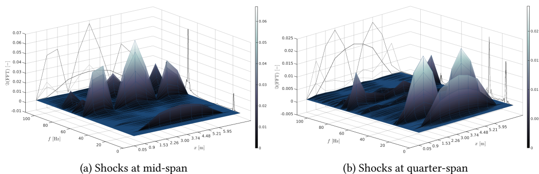
Figure 1.19: Imaginary part of acceleration FFT response - beam HA16-C1A-1
