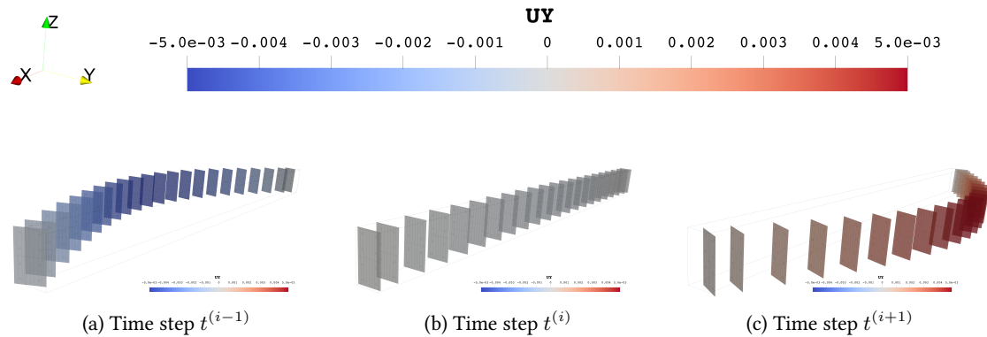
Figure 2.13: DSS2 test - Beam displacement [m] - damping formulation comparisons RICBET - RD 2%
