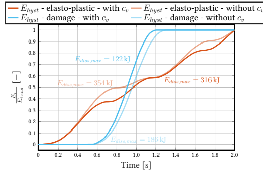
Figure 1.10: Different types of damping - one DOF system - dissipative energies - influence of viscous damping
