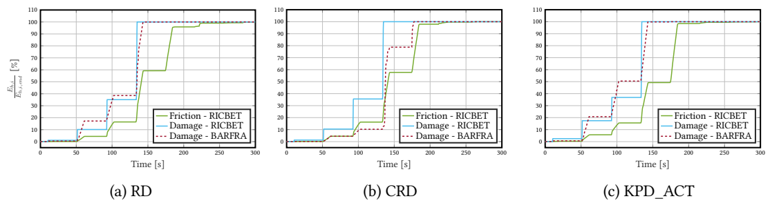
Figure 2.40: DSS2 test - Dissipation proportions at the material level - RICBET and BARFRA - 2%
