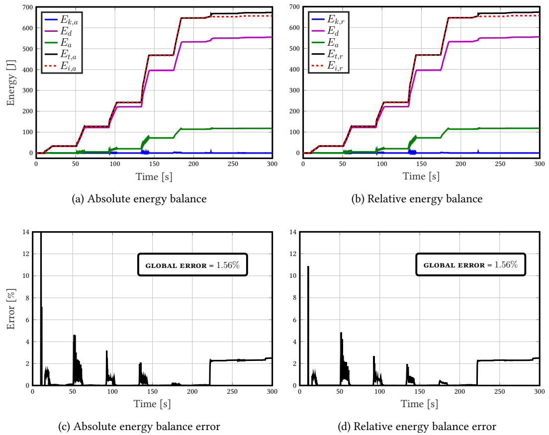
Figure 2.28: DSS2 test - Structural energy balances - RICBET - RD 2%
