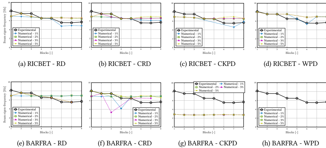
Figure 2.18: DSS2 test - Frequency responses of the white-noise signals - damping ratio comparisons
