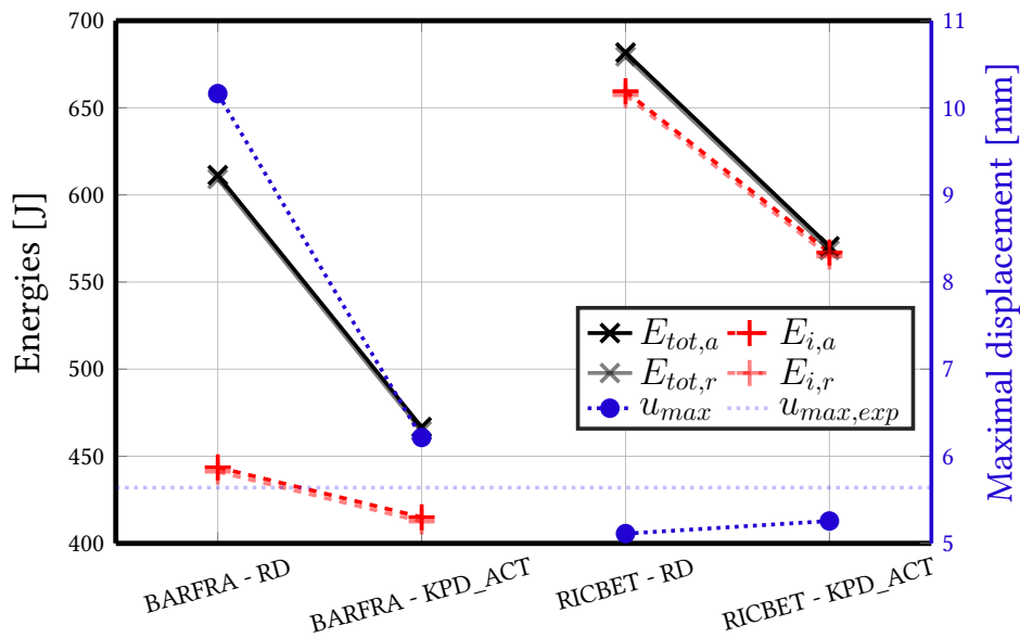
Figure 2.30: DSS2 test - Imparted and total energies in parallel to the maximal displacement - 2%
