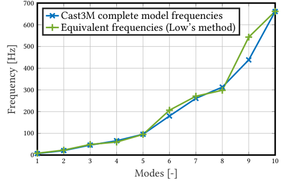
Figure 3.7: Validation of eigenfrequency combinations
