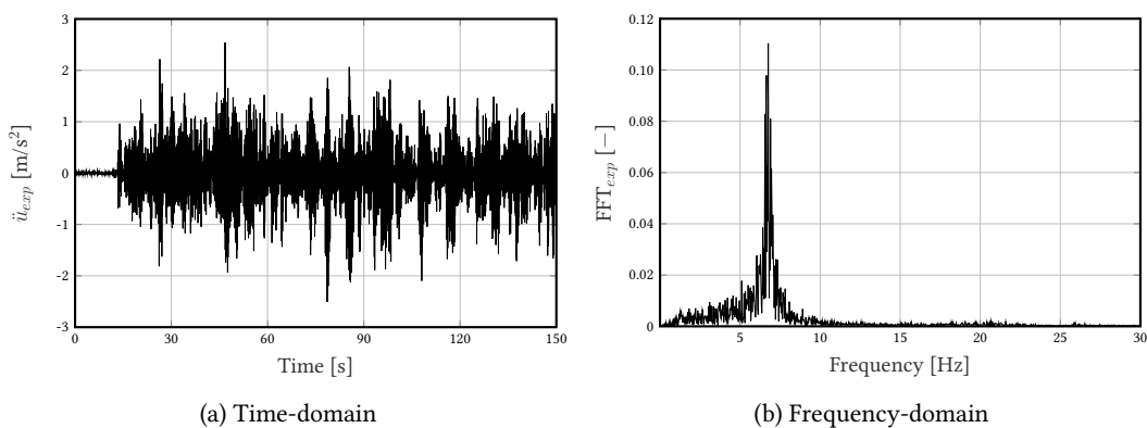
Figure 1.24: Mid-span acceleration response of the beam HA16-C1A-2 submitted to the WN1 input signal in figure 1.23a
