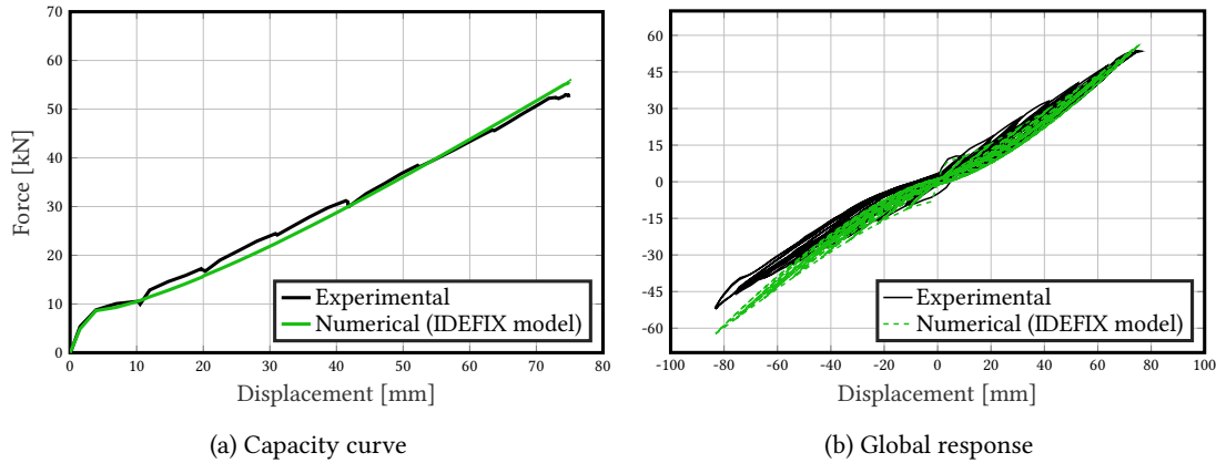
Figure 3.24: Quasi-static responses of calibrated IDEFIX numerical model
