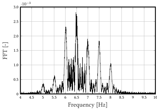
Figure 2.9: Frequency response between 4 Hz and 10 Hz of a complete DSS2 test
