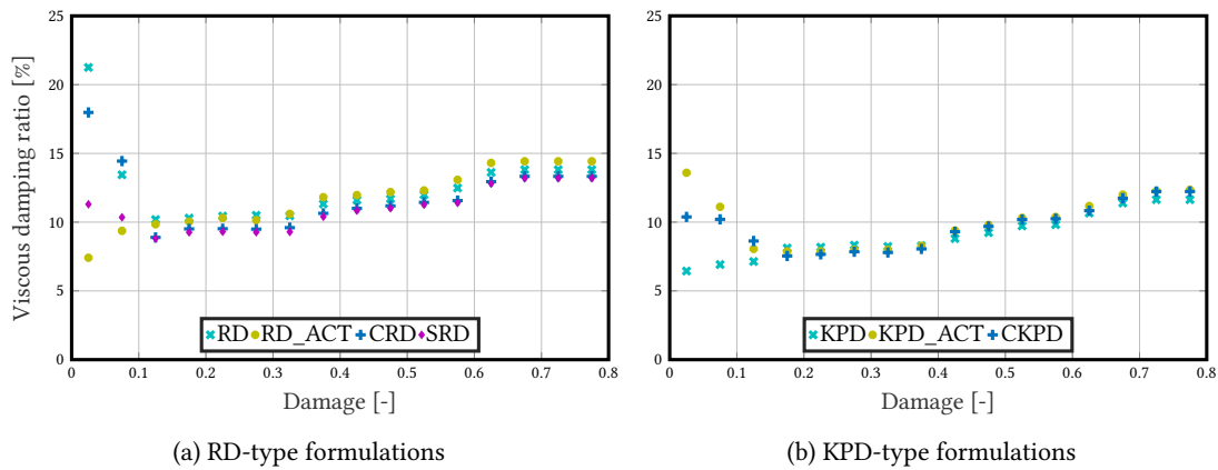
Figure 3.21: DSS2 test (harmonic parts) - Numerical identified evolutions \xi_1(d) - RICBET 2%
