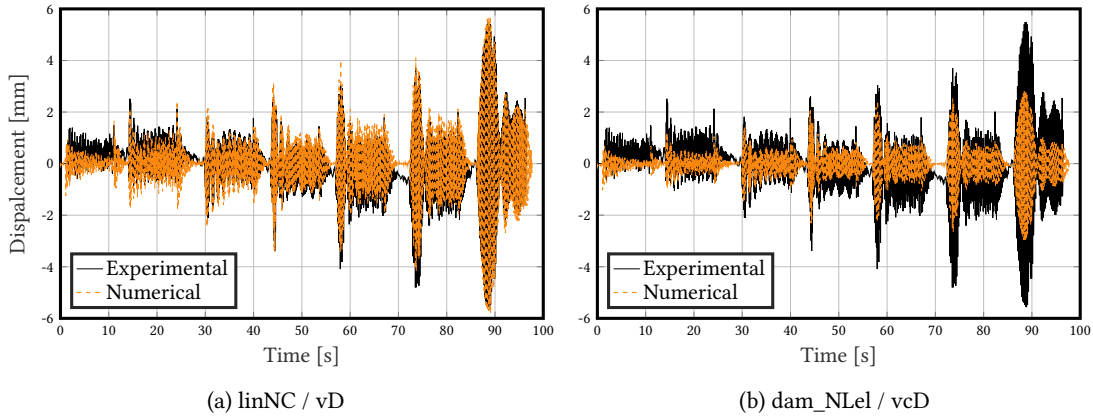
Figure 3.29: Displacement identifications
