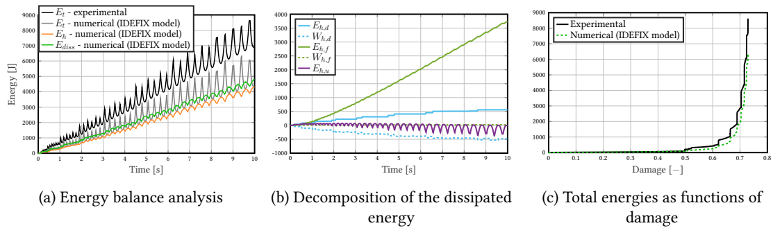
Figure 3.25: Quasi-static energy balance with IDEFIX model
