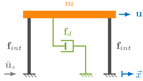
Figure 1.6: SDOF system
