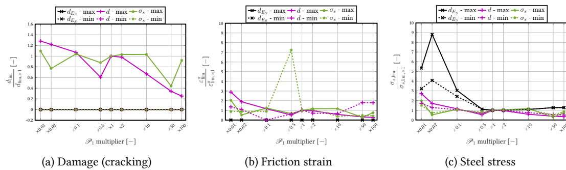
Figure G.5: Parametric study of function parameters - diagonal damping matrix formulation - \mathcal{P}_1 evolution - normalized maximal and minimal values of some variables
