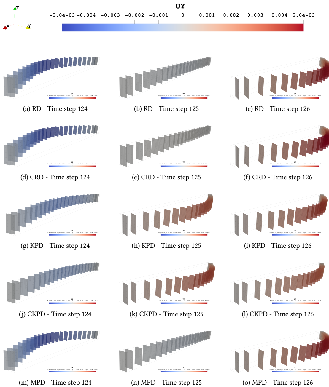
Figure D.2: DSS2 test - increment 4 - Beam displacement [ m ] - damping formulation comparisons - RICBET 2%
