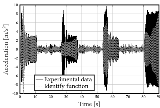
(c) DSS3 test - acceleration
