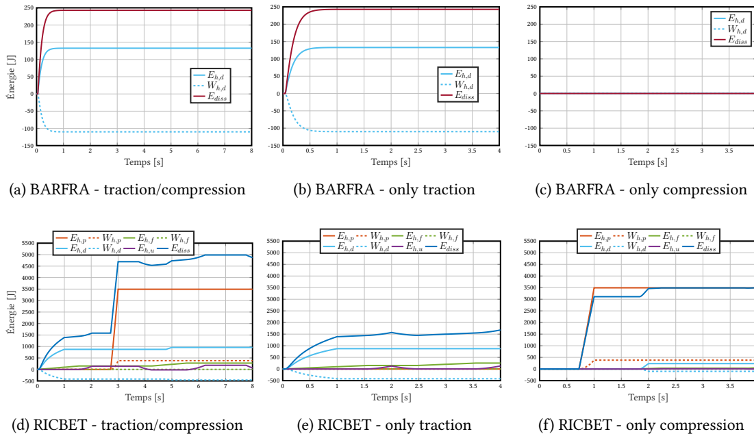
Figure 2.23: Energy distribution of dissipative phenomena for one fibre element - two cycles
