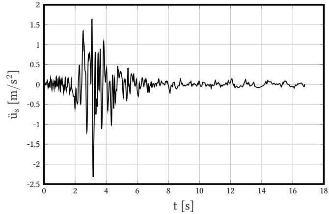
Figure 3.12: Seismic acceleration
