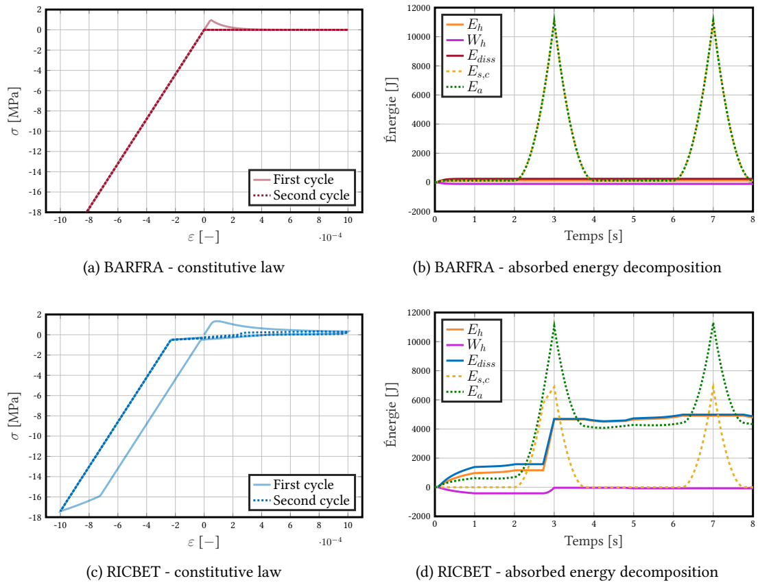
Figure 2.22: Energy analysis of one fibre element of concrete - two traction/compression cycles
