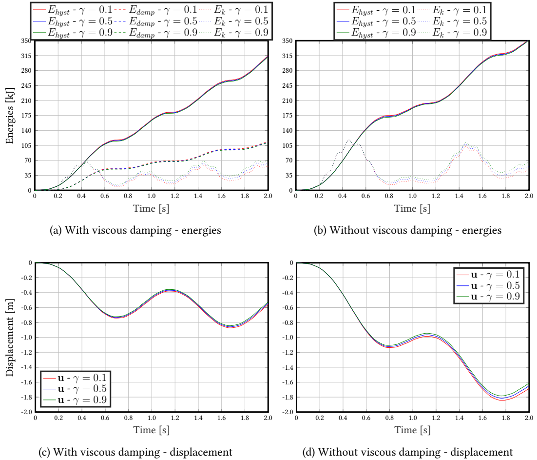
Figure 1.12: Different types of damping - one DOF system - numerical damping - elasto-plastic model
