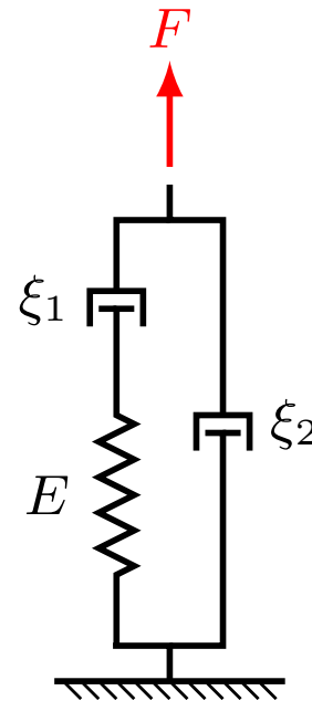
Figure 1.15: Generalised Maxwell model
