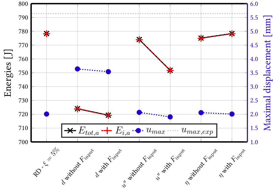
Figure 3.32: DSS2 test with IDEFIX model - Imparted and total energies (absolute energy balance) in parallel to the maximal displacement - proposed damping models depending on internal variables
