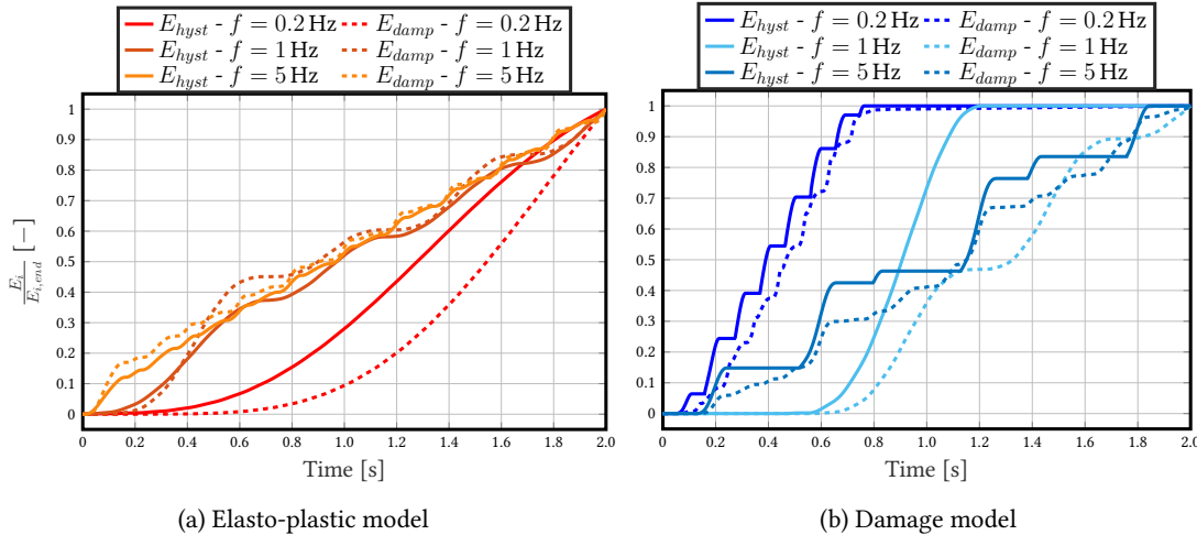
Figure 1.11: Different types of damping - one DOF system - influence of the input signal frequency
