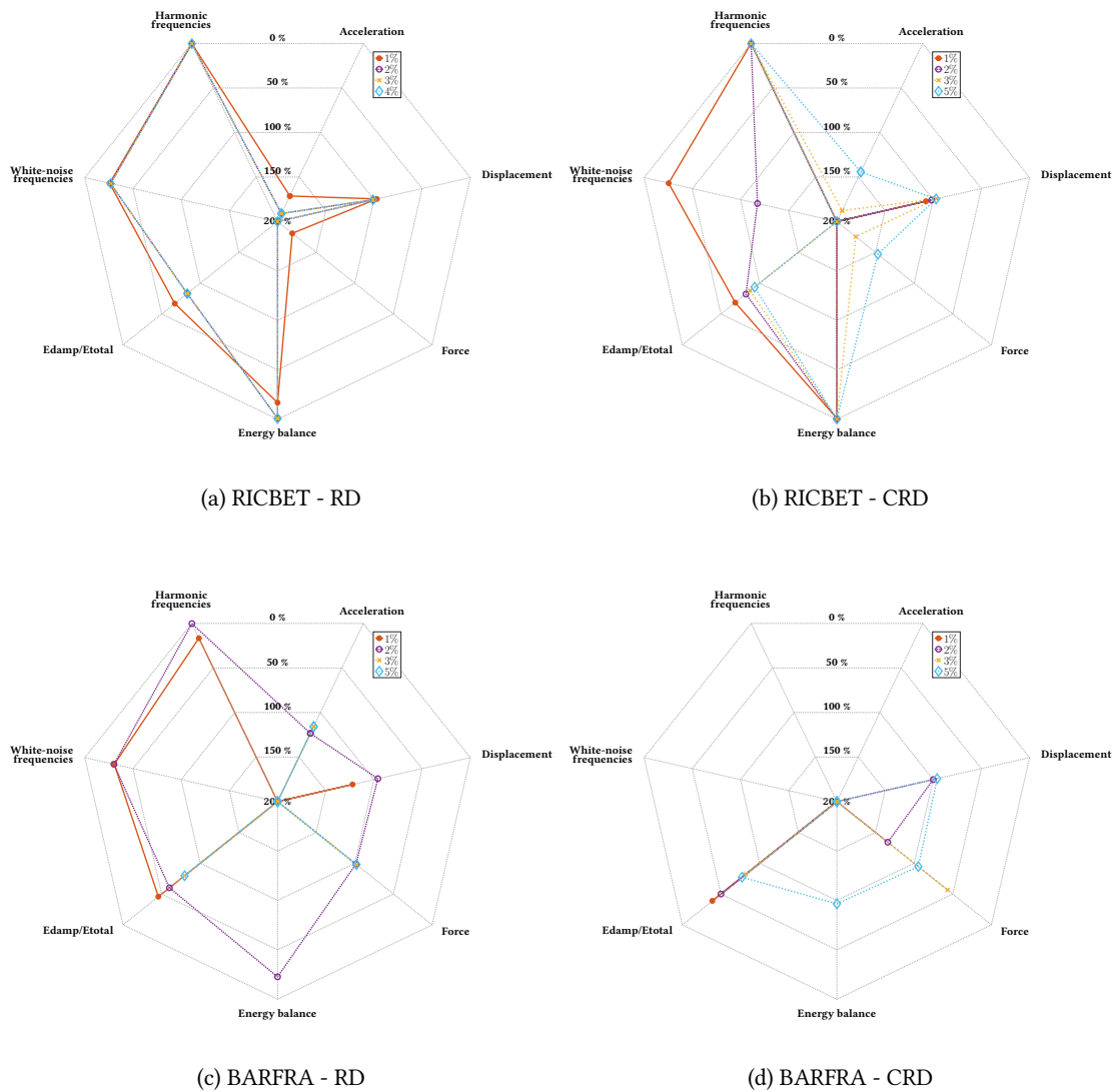
Figure 2.45: DSS2 test - Synthesis of damping ratio and constitutive model comparisons
