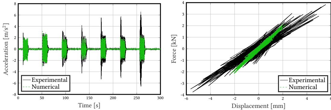
(a) Acceleration response - without F_{input}/F_{input,max}
