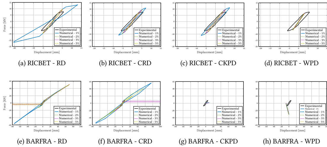
Figure 2.17: DSS2 test - Behaviour law envelopes - damping ratio comparisons
