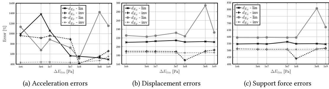
Figure 3.38: Parametric study for the update limit with d_{E_S} and d_{E_T} variables - non-diagonal damping matrix formulation
