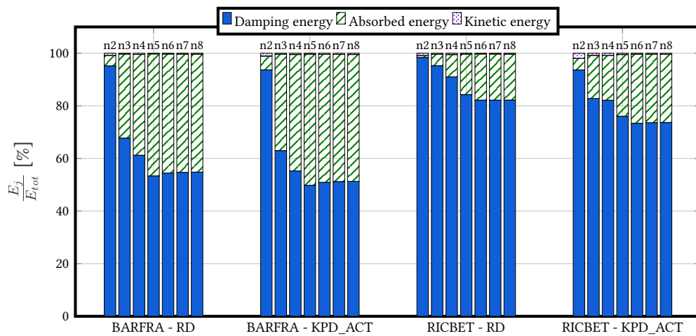
Figure 2.29: DSS2 test - Distribution of dissipative energies at the structural level along the computation - 2%
