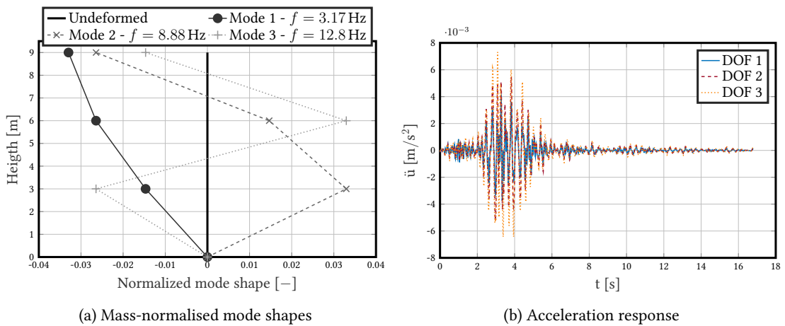
Figure 3.13: "Reference solution" of the three DOFs system
