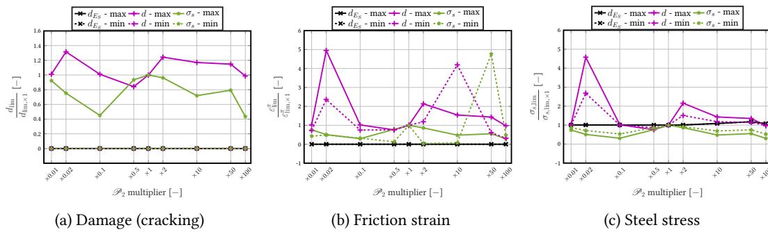
Figure G.8: Parametric study of function parameters - diagonal damping matrix formulation - \mathcal{P}_2 evolution - normalized maximal and minimal values of some variables
