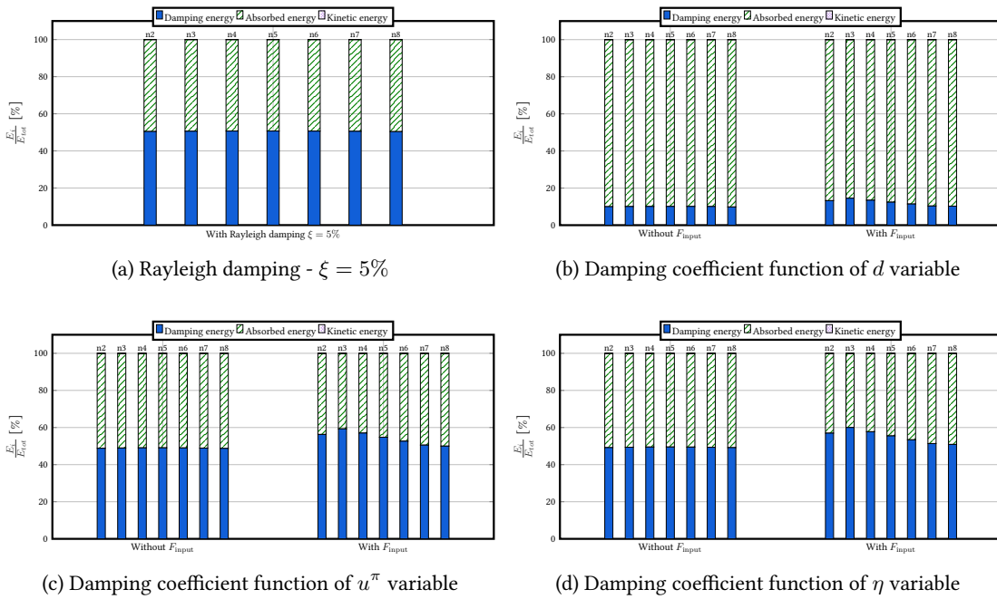
Figure 3.33: DSS2 test with IDEFIX model - Distribution of dissipative energies at the structural level along computation - proposed damping models depending on internal variables
