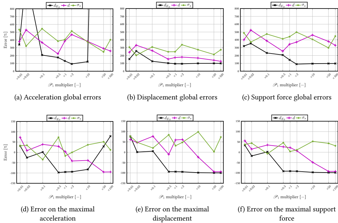
Figure G.4: Parametric study of function parameters - diagonal damping matrix formulation - \mathcal{P}_1 evolution - global responses
