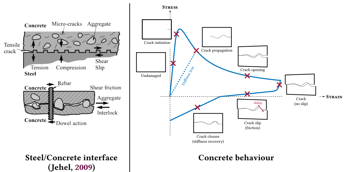
Figure 2: Dissipative phenomena mechanisms of reinforced concrete
