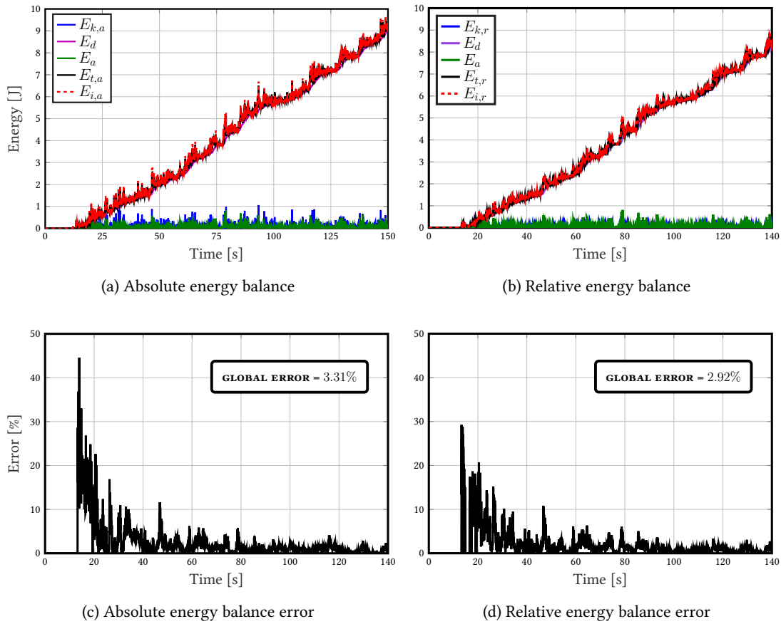
Figure 2.25: WN1 test - Structural energy balances - RICBET - RD 0.5%
