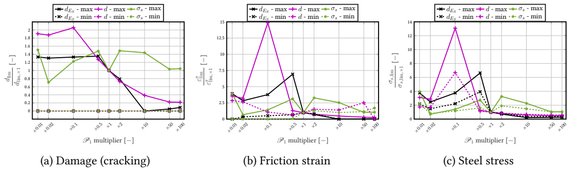
Figure 3.40: Parametric study of function parameters - non-diagonal damping matrix formulation - \mathcal{P}_1 evolution - normalised maximal and minimal values of some variables
