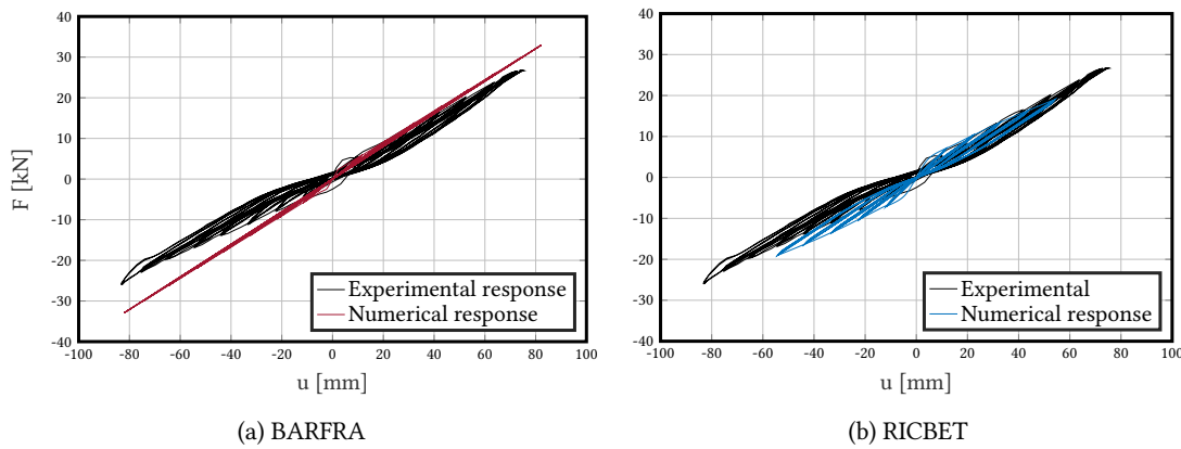
Figure 2.7: Responses of the calibrated concrete models in comparison with the experimental quasi-static data
