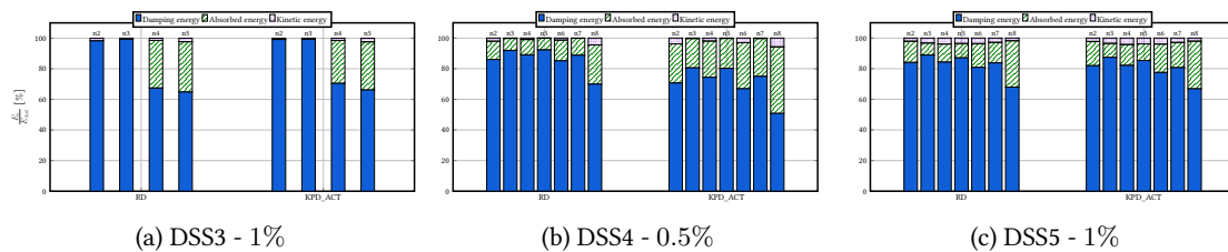
Figure 2.36: DSS3 to DSS5 tests - Distribution of dissipative energies at the structural level along the computation - RICBET
