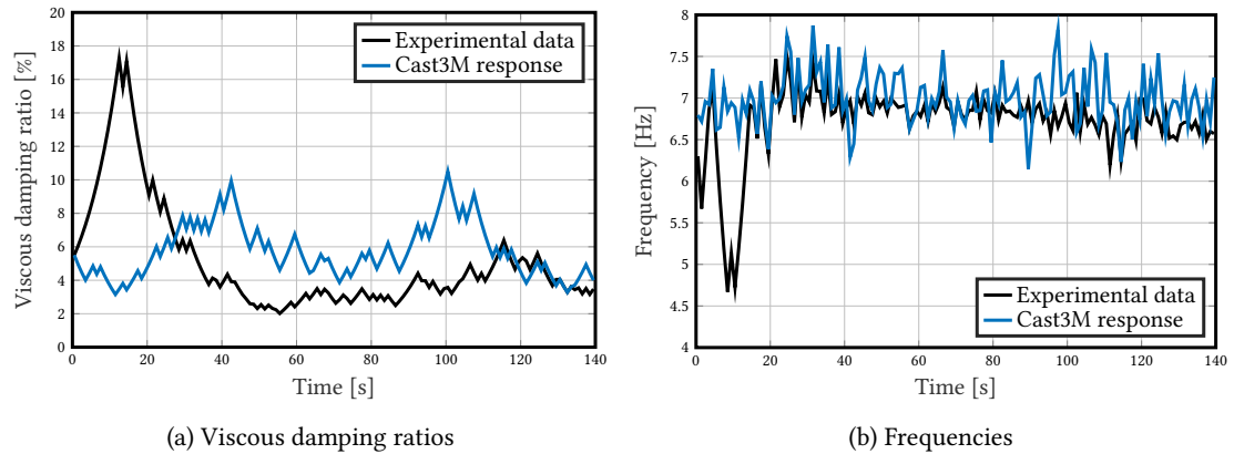
Figure 3.16: WN1 test - Application of the damping identification method on beam responses - identified parameters
