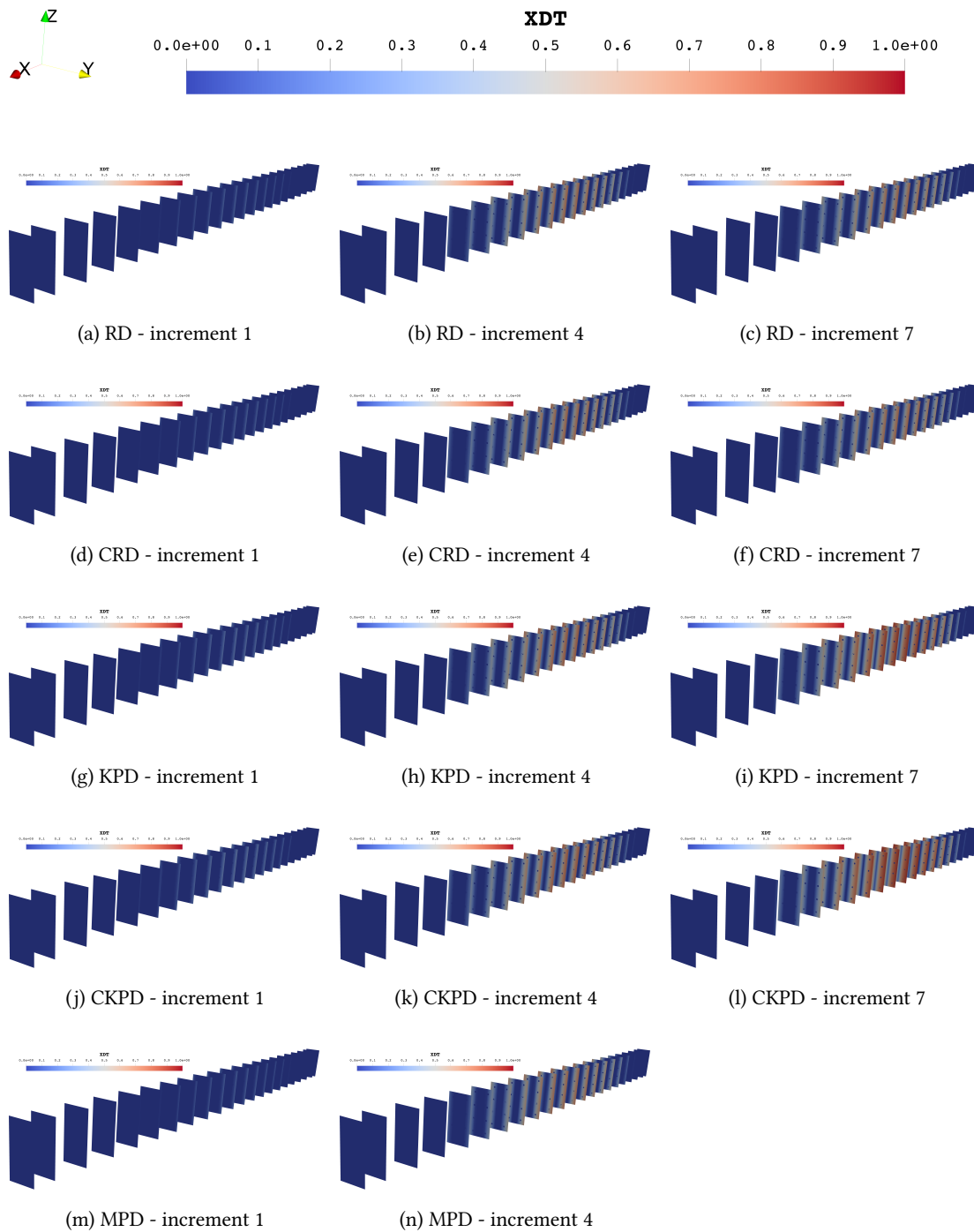
Figure D.4: DSS2 test - Damage variable evolution along the beam - damping formulation comparisons - RICBET 2%
