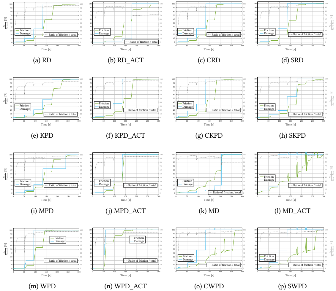
Figure C.1: DSS2 test - Dissipation proportions at material level - RICBET 2% - damping formulation influence
