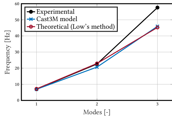
Figure 3.8: Comparison of the three first eigenfrequencies
