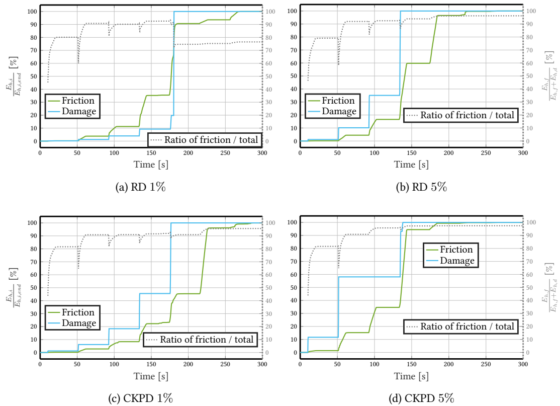
Figure 2.39: DSS2 test - Dissipation proportions at the material level - RICBET - some results
