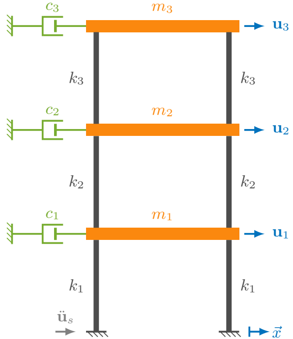
Figure 3.11: Three DOFs discrete system
