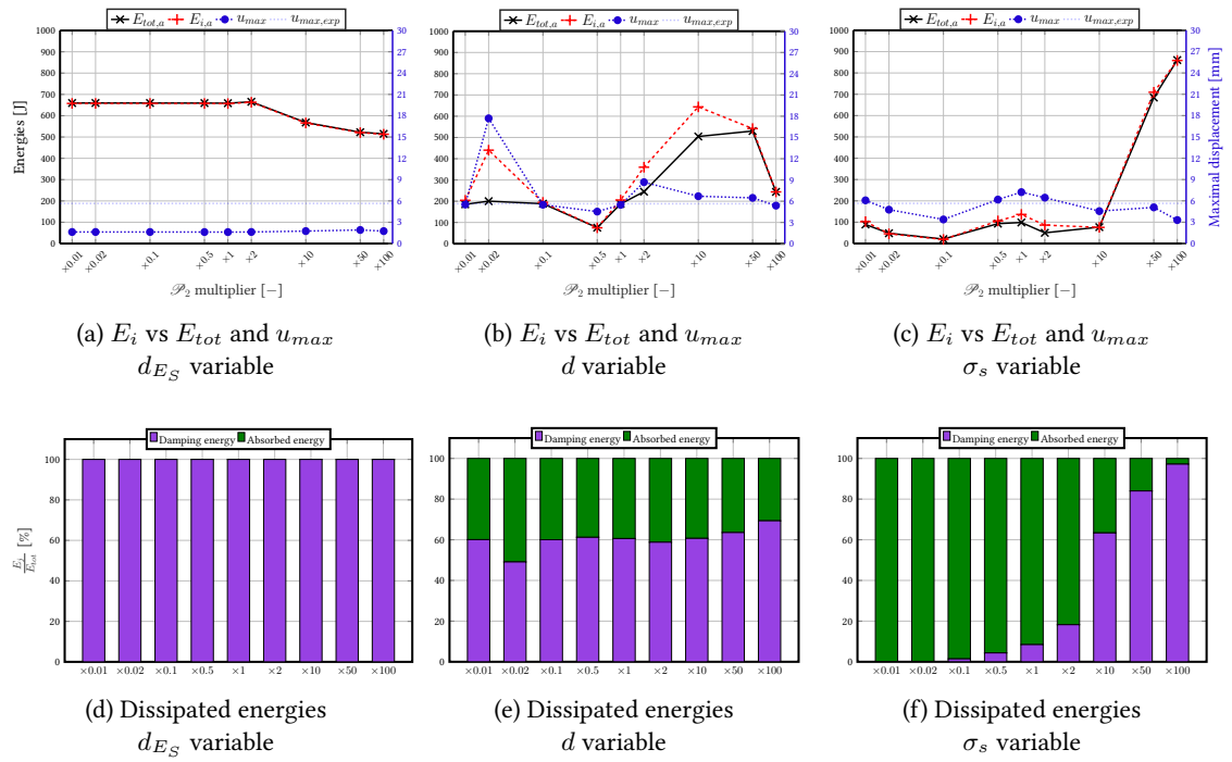
Figure G.9: Parametric study of function parameters - diagonal damping matrix formulation - \mathcal{P}_2 evolution - energy analyses
