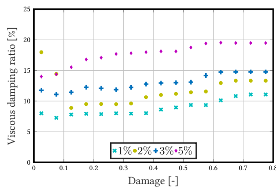
Figure 3.22: DSS2 test (harmonic parts) - Numerical identified evolutions \xi_1(d) - RICBET CRD - viscous damping ratio influence
