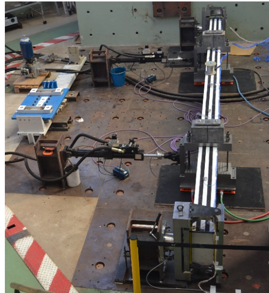
Figure 1.20: Quasi-static experimental setup (Heitz, 2017)
