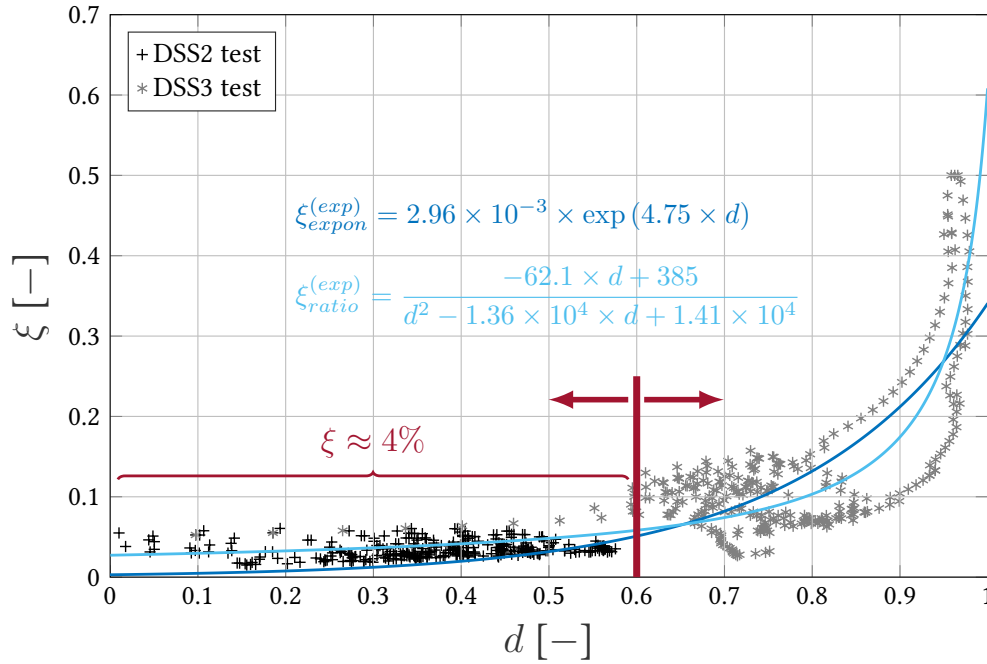
Figure 3.19: DSS2 and DSS3 tests - \xi_1(d) identified on experimental data - harmonic signal parts
