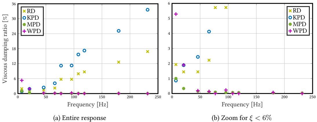
Figure 3.2: Equivalent viscous damping ratio for ten modes - initial matrices
