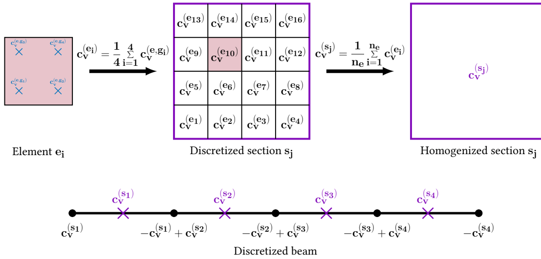
Figure 3.36: c_v from Gauss point to beam nodes
