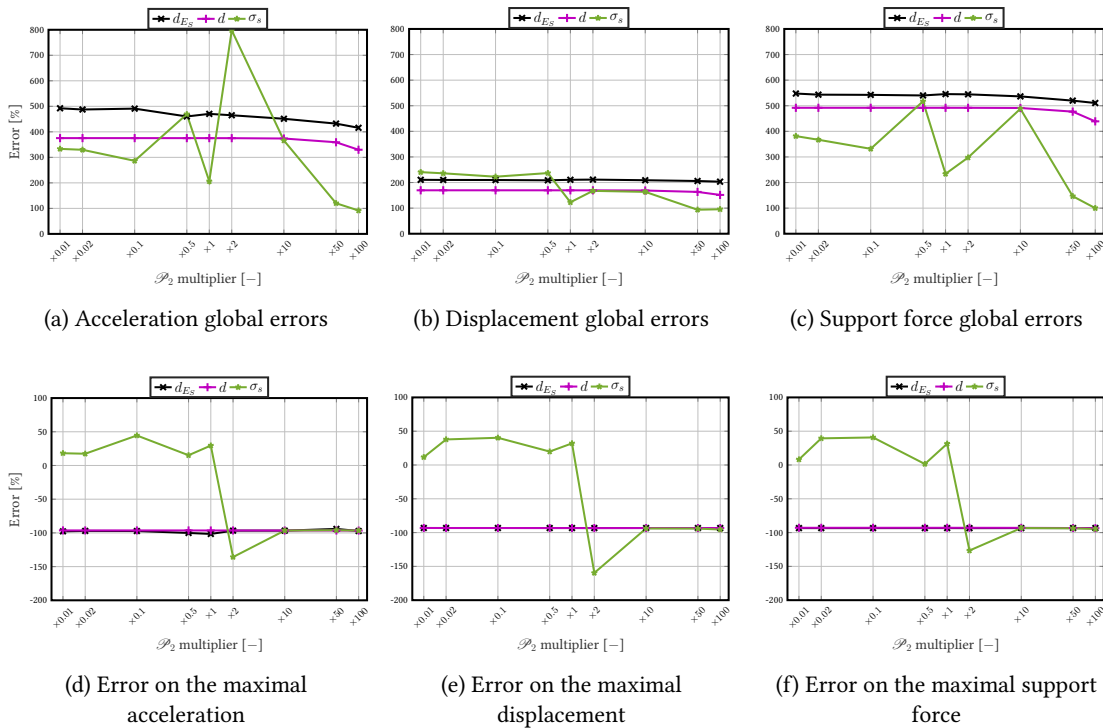
Figure G.1: Parametric study of function parameters - non-diagonal damping matrix formulation - \mathcal{P}_2 evolution - global responses
