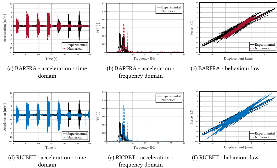
Figure 2.14: DSS2 test - Dynamic responses - KPD_ACT 2%
