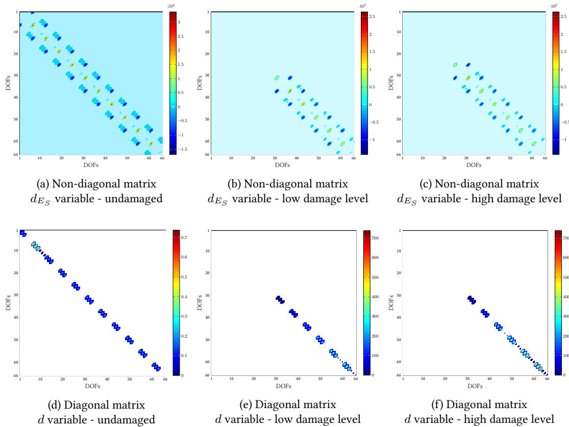
Figure 3.42: Updated damping matrices at different damage levels
