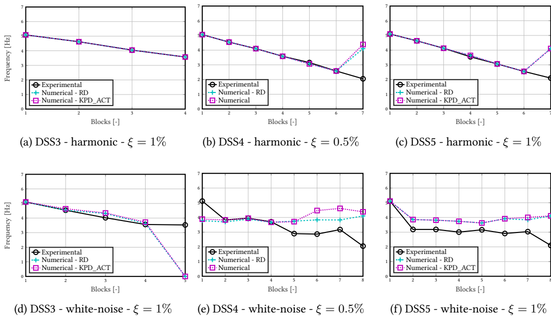
Figure 2.21: DSS3 to DSS5 tests - Frequency evolutions - RICBET
