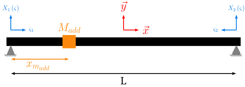
Figure 3.6: Scheme of the beam with one additional mass
