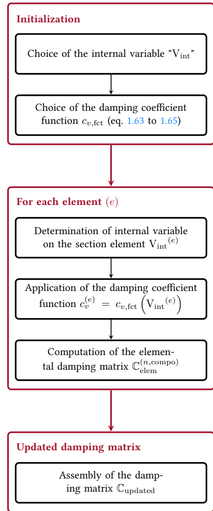
Figure 3.35: Algorithm of updated damping matrix computations
