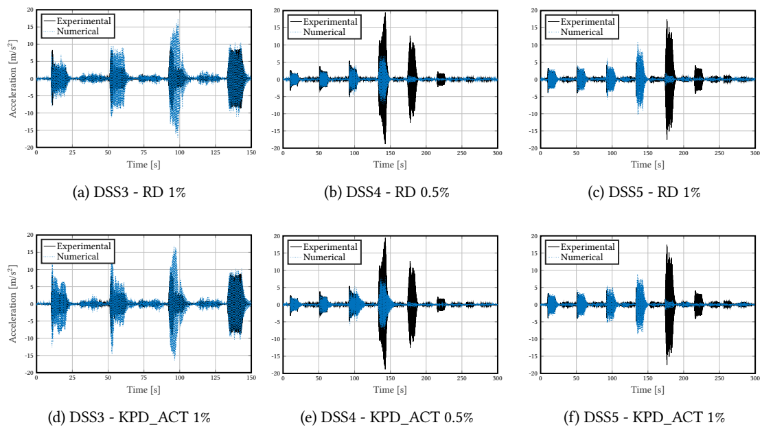
Figure 2.19: DSS3 to DSS5 tests - Acceleration responses - RICBET
