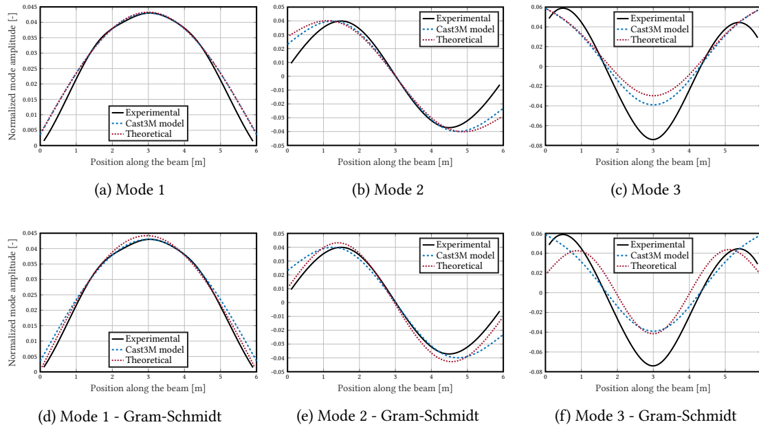
Figure 3.9: Combination of mode shapes - Rayleigh's quotient method
