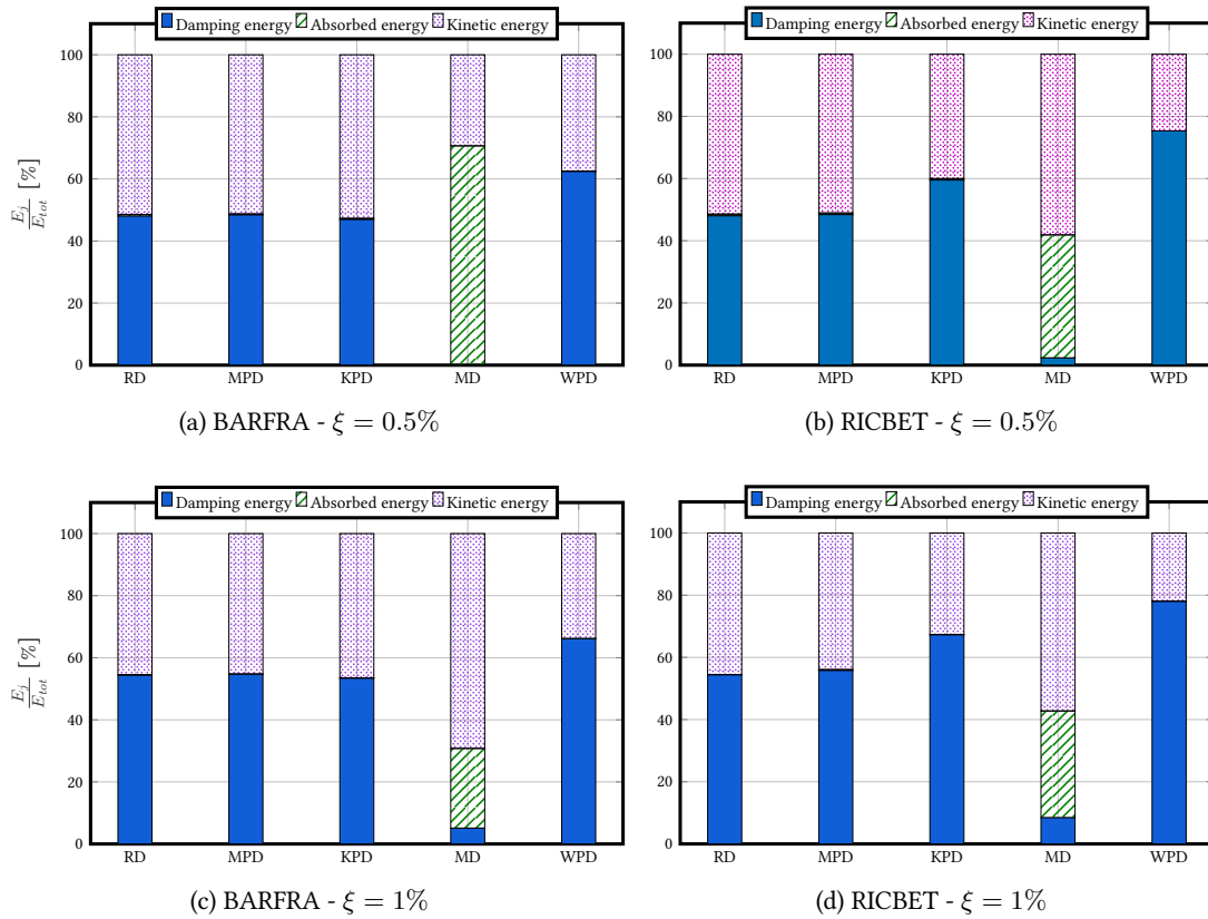
Figure 2.27: WN1 test - Distribution of dissipative energies at the structural level - absolute energy balance
