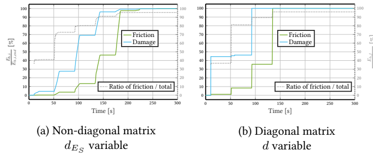
Figure 3.44: Updated damping matrix - Dissipation proportions at the material level - comparisons of updated damping matrix formulations
