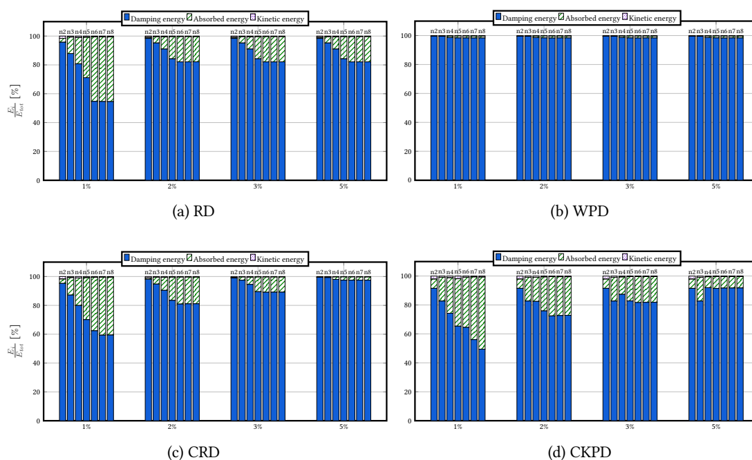
Figure 2.34: DSS2 test - Distribution of dissipative energies at the structural level along the computation - RICBET - \xi influence
