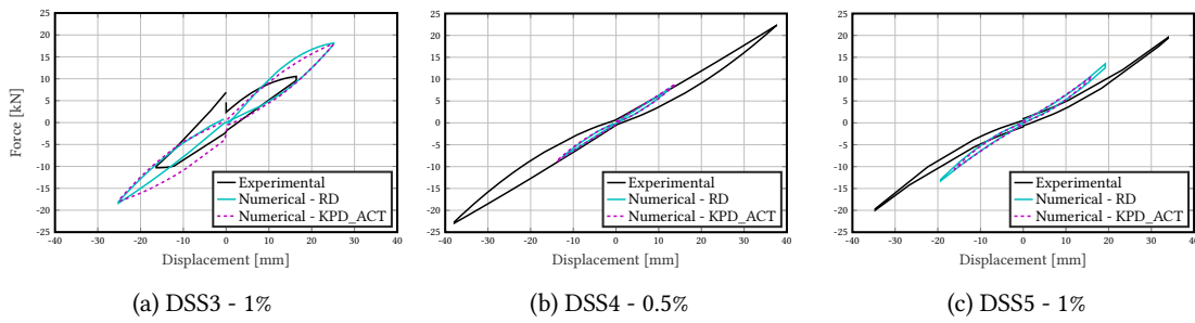
Figure 2.20: DSS3 to DSS5 tests - Behaviour law envelopes - RICBET
