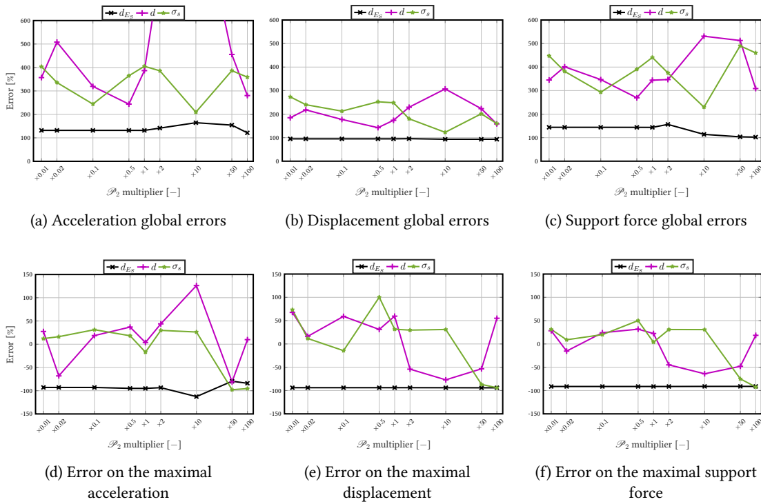
Figure G.7: Parametric study of function parameters - diagonal damping matrix formulation - \mathcal{P}_2 evolution - global responses
