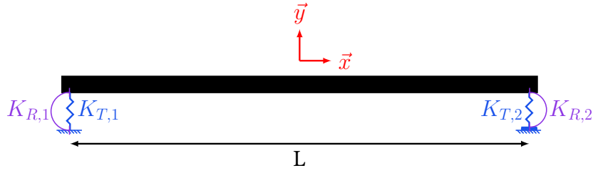
Figure 3.5: Scheme of the beam on elastic supports
