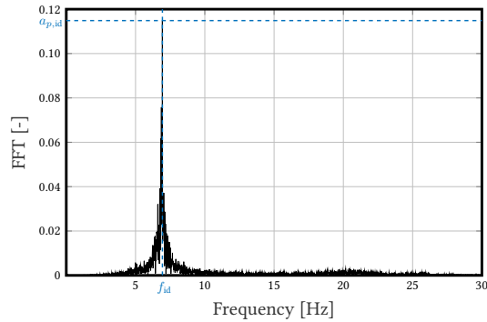
Figure 2.8: Eigenfrequency and peak amplitude determination on a white-noise response
