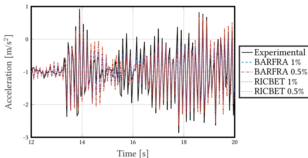
Figure 2.12: WN1 test - Damping formulation comparisons
