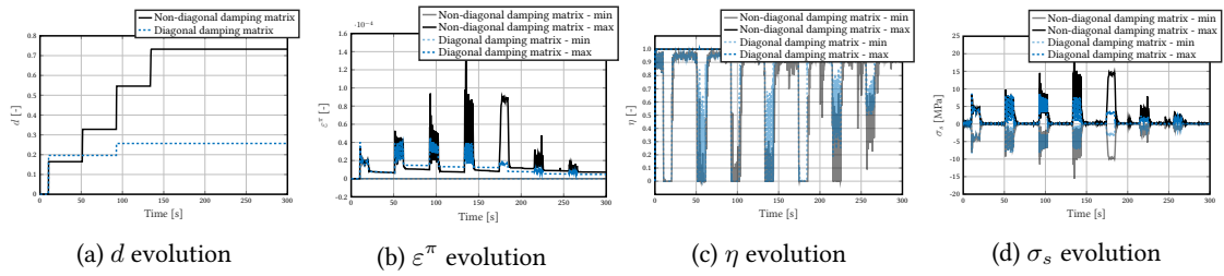
Figure 3.43: Updated damping matrix - Evolution of nonlinear variables and steel stresses - comparison of updated damping matrix formulations
