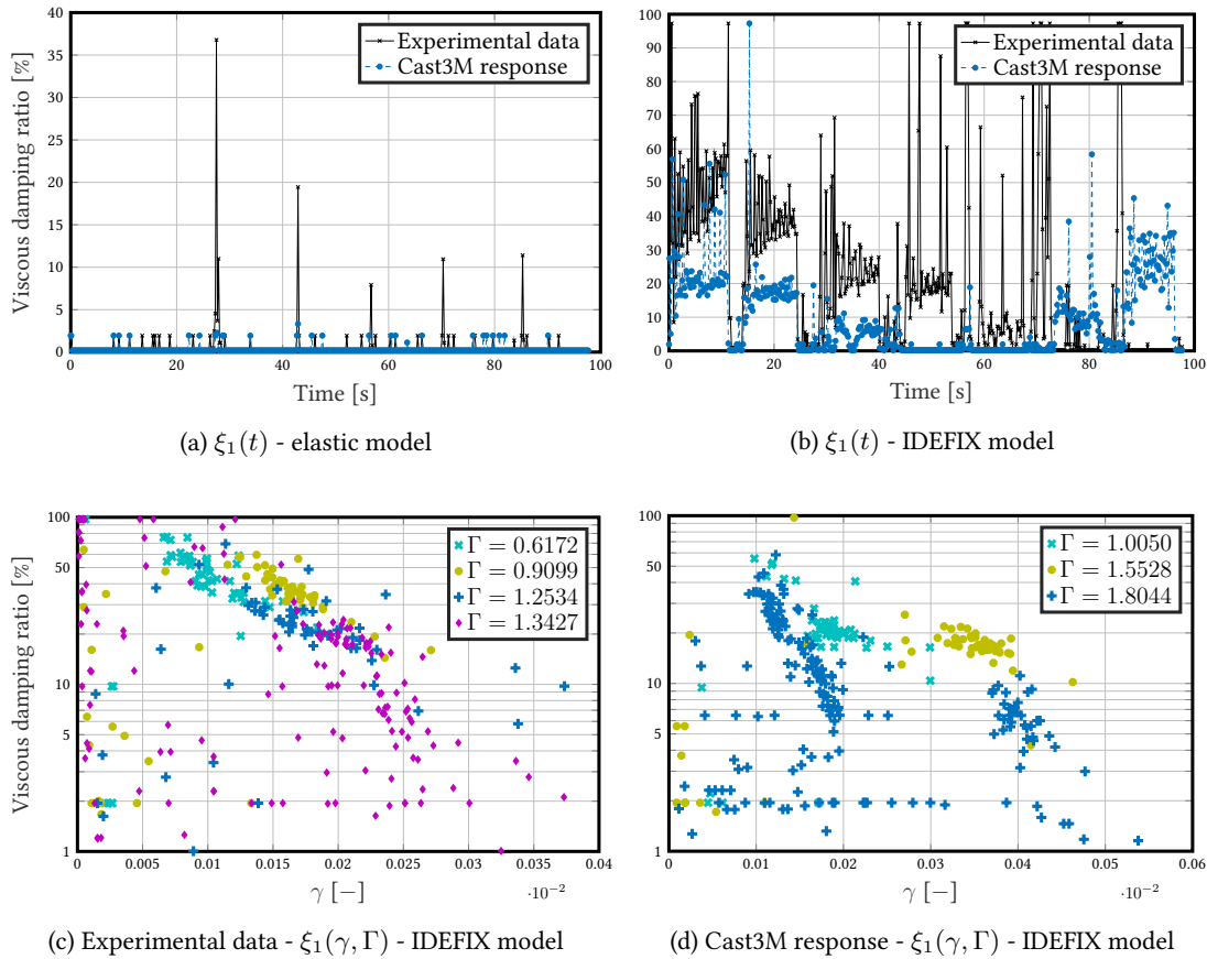
Figure 3.27: DSS2 test (harmonic parts) - Identified viscous damping ratios with IDEFIX model - dependence on the damage indices \gamma and \Gamma
