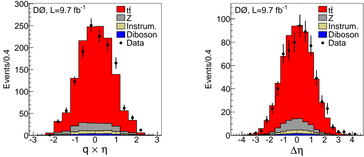
Figure 2.18: Distributions in q \times \eta and \Delta\eta = \eta_{\ell^+} - \eta_{\ell^-} for the sum of ee , e\mu and \mu\mu events, 9.7 \text{ fb}^{-1} , [43].
