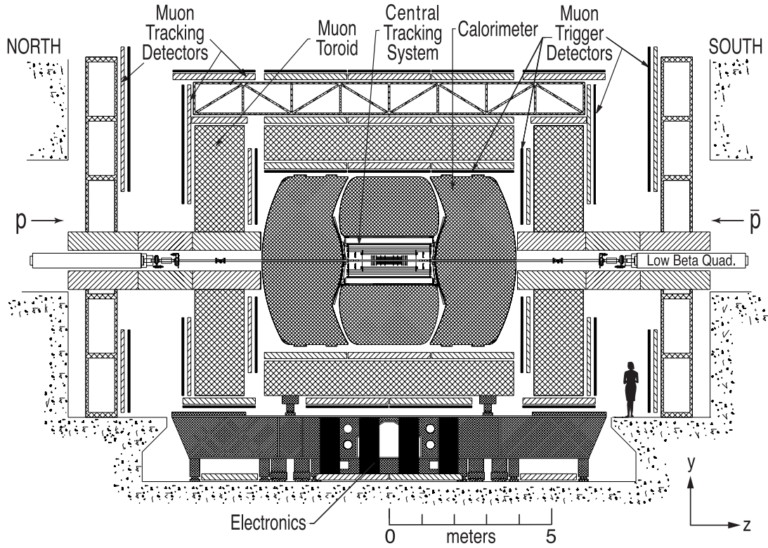
Figure 1.2: D0 detector.
