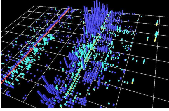
Figure 1.10: A typical “ring of fire” event. The x and y axes are \eta and \phi axes of calorimeter. Z axis is an absolute value of the calorimeter EM towers signal in ADC counts. Positive cell signals are indicated in red and negative in blue.
