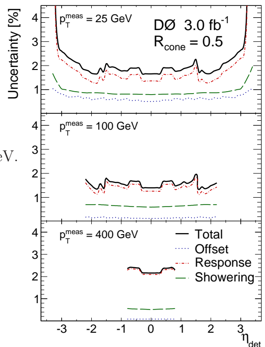
Figure 2.16: D0 JES uncertainty for jets in data as a function of the detector pseudorapidity \eta_{det} for different uncorrected p_T , [30].
