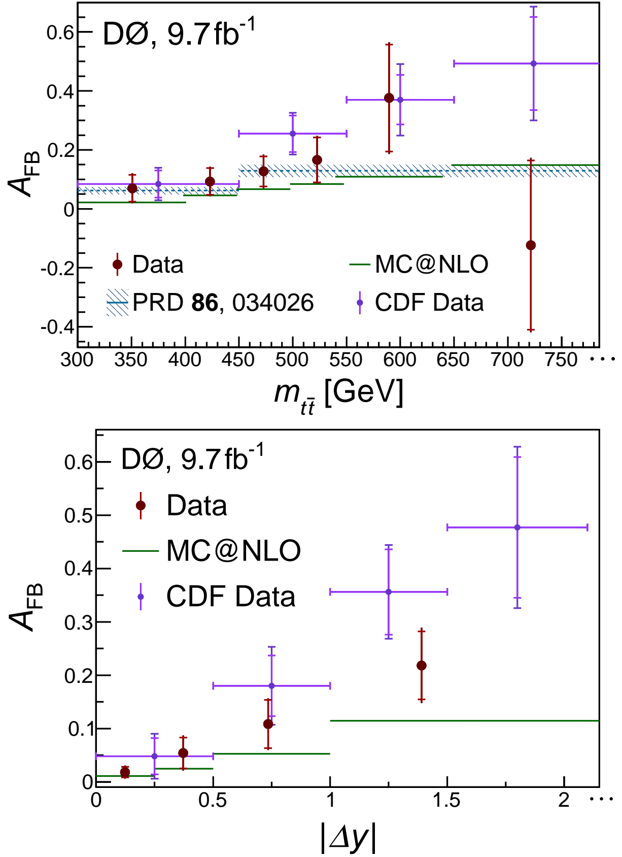
Figure 2.26: A_{t\bar{t}} asymmetry distribution as a function of m_{t\bar{t}} and |\Delta y| as measured by the DØ and CDF experiments in the \ell + \text{jets} final state [160, 161].
