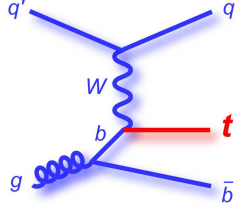
Figure 2.3: Feynman diagrams for the single top quark production.
