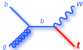
Figure 2.3: Feynman diagrams for the single top quark production.
