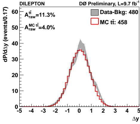
Figure 2.23: Distributions of the \Delta y and A_i variables after background subtraction, 9.7 \text{ fb}^{-1} , [80].
