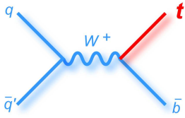
Figure 2.3: Feynman diagrams for the single top quark production.
