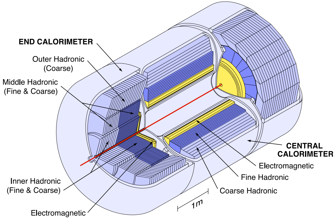
Figure 1.3: D0 calorimeters.
