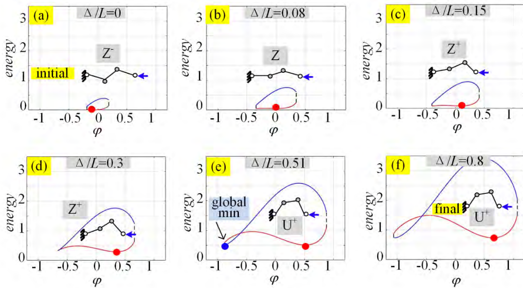
Fig. 1. 31: Evolution of energy- \phi curves for stable configuration for the initial "Z-configuration".
