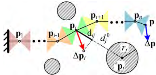
Fig. 5. 17: Computing the distances d_{ij} between the robot joints and obstacles
