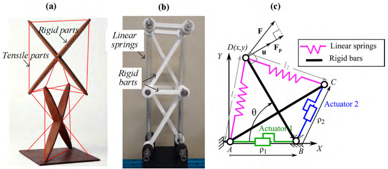
Fig. 1. 3: Typical stable tensegrity structures composed of rigid bodies connected by tensile parts: (a) Snelson's 3DOF X-piece, 1948 (Skelton and Oliveira, 2009). (b): 2-segment serial tensegrity mechanism (Furet and Wenger, 2019a). (c): 2DOF planar tensegrity mechanism (Boehler et al., 2015).
