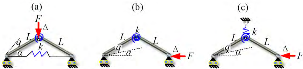
Fig. 1. 18: Examples of two-bar mechanisms where the buckling phenomenon is observed.
