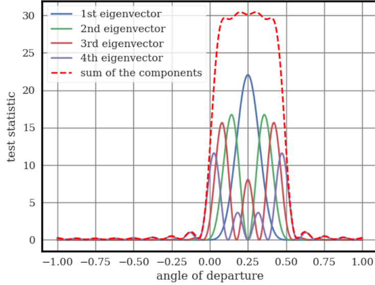
Figure 6.7 – Angular response of each individual weighted correlators of Equation (6.8) for the third interval detector out of four for any direction of departure t \in [-1, 1] . System with N_t = 16 antennas ( OS = 0.25 or US = 4 ).
