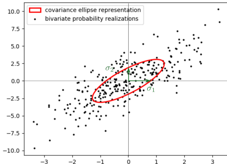
Figure C.1 – Ellipse representation of the covariance matrix of a distribution.
