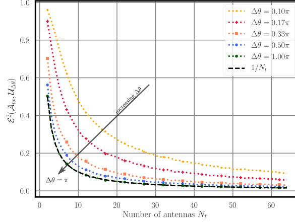
Figure 2.4 – Numerical evaluation of \mathcal{E}(\mathcal{A}_{tx}, \mathcal{U}_{\Delta\theta}) for increasing \Delta\theta with fixed half-wavelength antenna spacing. The lower, the better.
