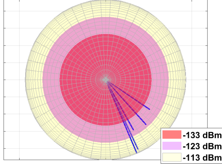
3-D AOD Power Spectrum - 60 GHz, UMi NLOS, 109.9 m T-R Separation
