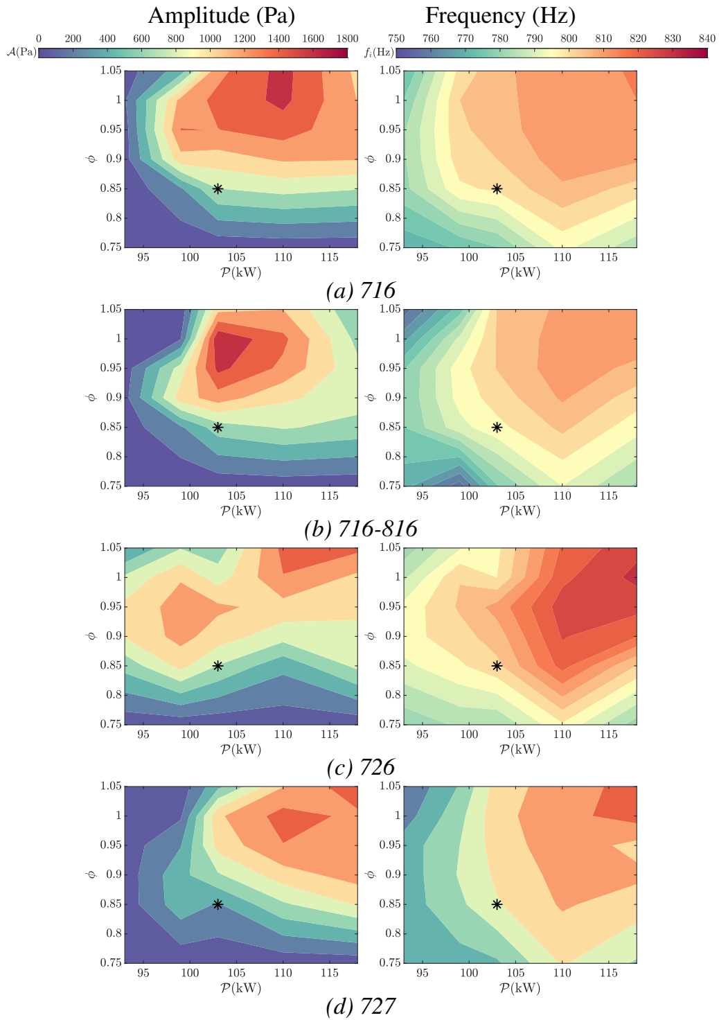
Figure 7.2. Amplitude (left) and frequency (right) stability map of MICCA-Spray for the different swirlers in the higher-swirl category. The swirlers in the lower-swirl category (707 and 712) are always stable in the assessed operating zone and hence are not shown here. The black star on the stability map refers to the operating conditions of the complementary single-injector combustor described in Section 7.5.
