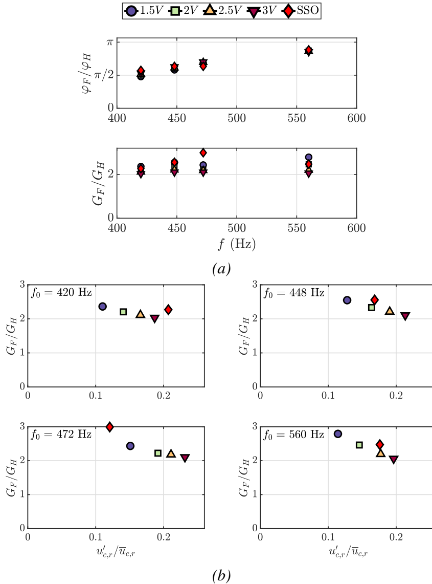
Figure 3.3. Comparison between the stable flame describing function \mathcal{F} and the combustion response under SSO, \mathcal{H} . (a) Phases \varphi_F and \varphi_H and gains G_F and G_H plotted at the four resonance frequencies and at different amplitude levels for SFM. The relative velocity fluctuation for obtaining \mathcal{F} and \mathcal{H} is measured in the chamber. The red diamonds represent phases and gains of \mathcal{H} during SSOs for different chamber lengths. The other colors and symbols correspond to the measured \mathcal{F} during SFM obtained while modulating the flame at the SSO frequencies and at four different levels of amplifier voltages (1.5, 2, 2.5, and 3 V). (b) Gain of \mathcal{F} and modulus of \mathcal{H} plotted as a function of the relative velocity fluctuation in the chamber. The velocity is measured at the reference position (r, z) = (4.0, 2.5) mm. The representation in terms of amplifier voltages shown in (a) is expressed in terms of velocity fluctuation levels in (b).
