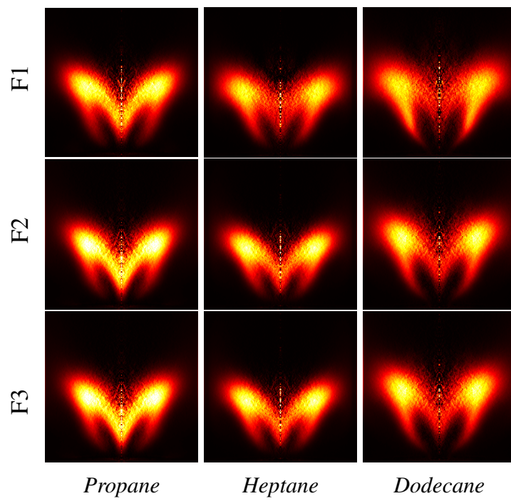
Figure C.8. Swirler 727
