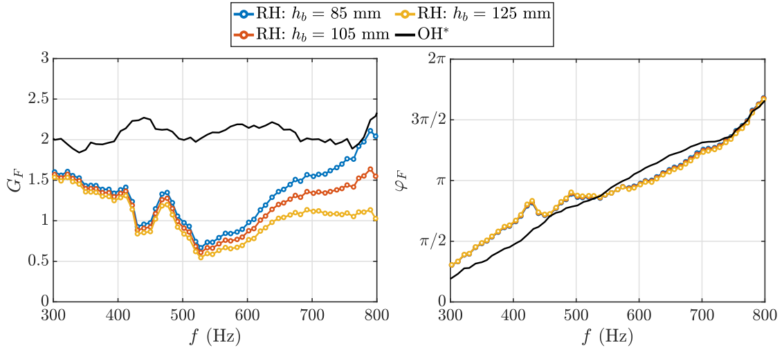
Figure A.4. Sensitivity of flame describing function determined using an acoustic method to the distance h_b between flame section and microphone measurement section. Swirler: 716, h_r = 6.75 mm, operating point: F1, V_0 = 3 V.
