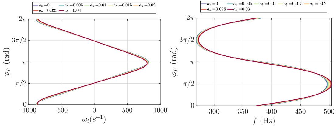
Figure 5.5. Sensitivity of the growth rate \omega_i and frequency f to the flame barycenter location a_b .
