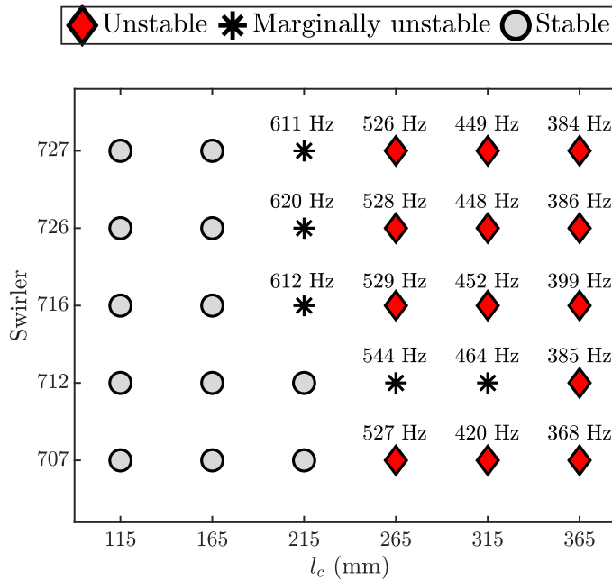
Figure D.2. Stability map of SICCA-Spray with five different swirlers at F1.
