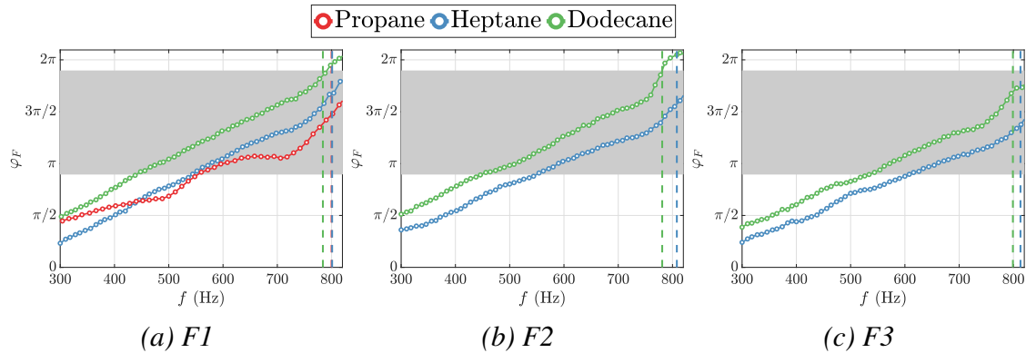
Figure 9.13. FTF phase for the three fuels at V_0 = 3 V and at the three operating points F1 ( \mathcal{P} = 6.4 kW, \phi = 0.85 ), F2 ( \mathcal{P} = 6.4 kW, \phi = 0.95 ) and F3 ( \mathcal{P} = 7.4 kW, \phi = 0.95 ). Unstable bands are obtained using a linear extrapolation of impedance gain (case B) and shown in gray. The dashed vertical lines correspond to the instability frequency of MICCA-Spray. In (a), the dashed lines corresponding to heptane and propane coincide. The instability analysis of propane is only carried out at F1 as a reference case.
