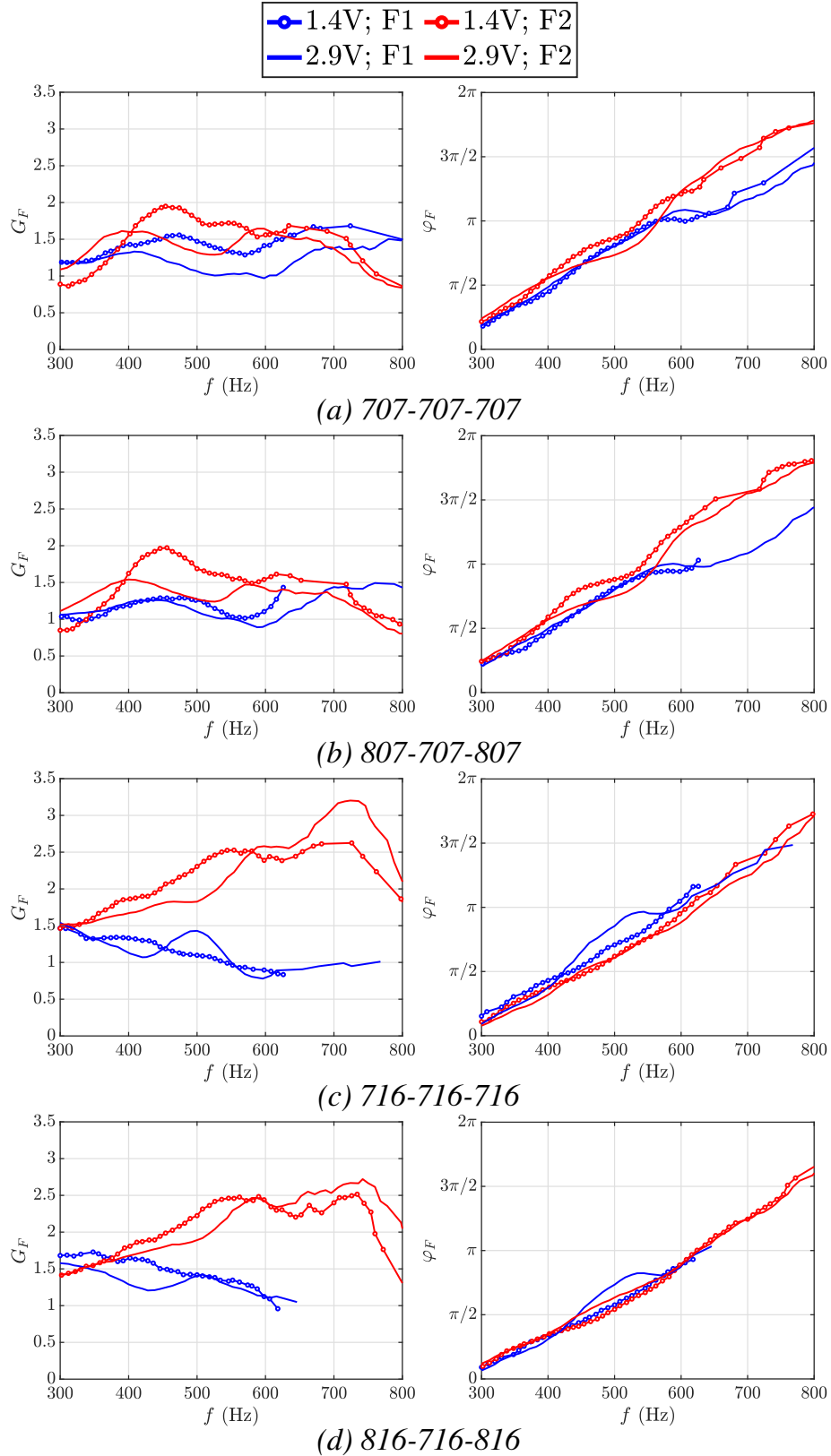
Figure 10.6. Comparison between operating points: gain G_F and phase \varphi_F of the FDFs measured in TICCA-Spray showing the comparison between the two operating points for the different swirler combinations (F1: blue, F2: red). Results are only plotted at two amplifier voltages V_0 = 1.4\text{ V} (solid line with marker) and 2.9\text{ V} (solid line without marker), to illustrate the differences.
