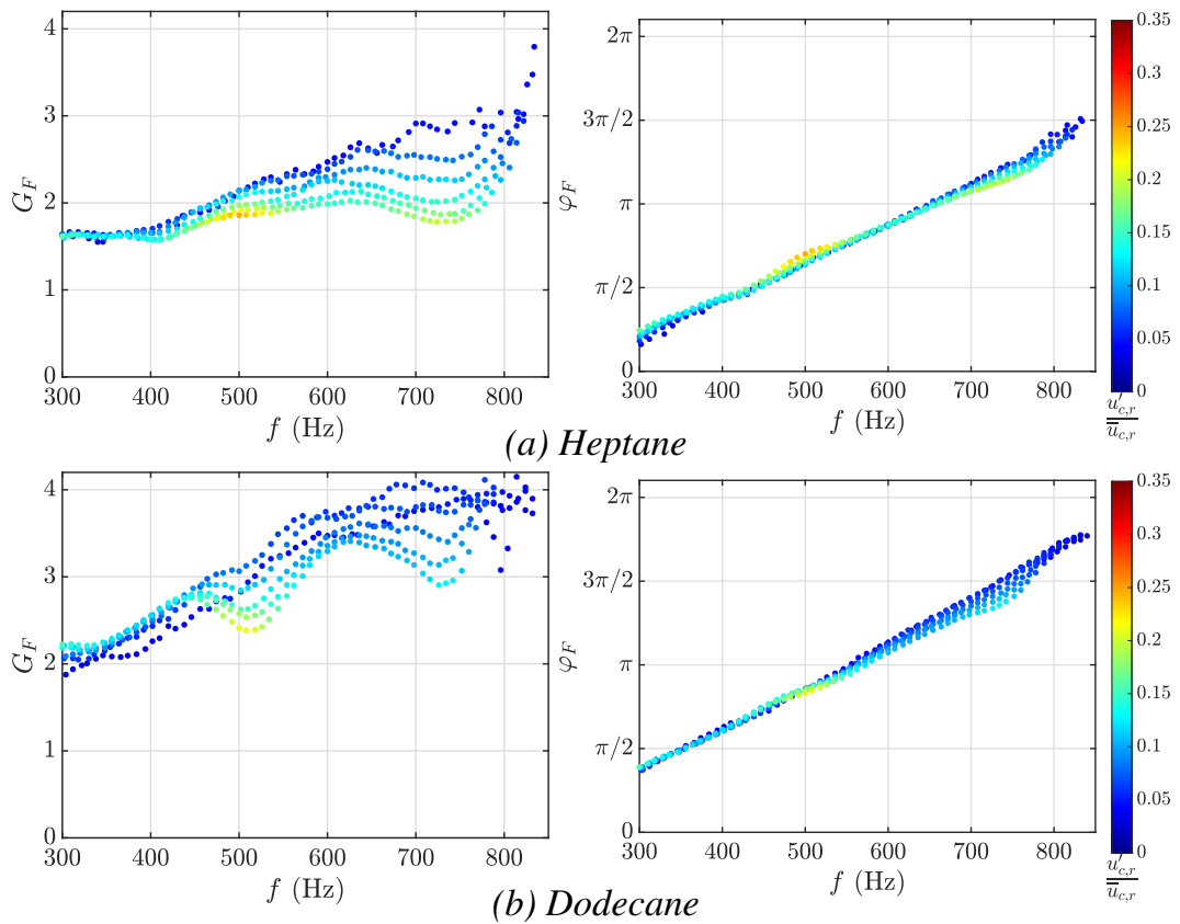
Figure 9.15. FDF (gain G_F and phase \varphi_F ) of the direct flame describing function in SICCA-Spray for the liquid fuels at F3 ( \mathcal{P} = 7.4 \text{ kW} & \phi = 0.95 ) with color axis representing the level of velocity fluctuations u'_{c,r}/\bar{u}_{c,r} at the injector outlet.
