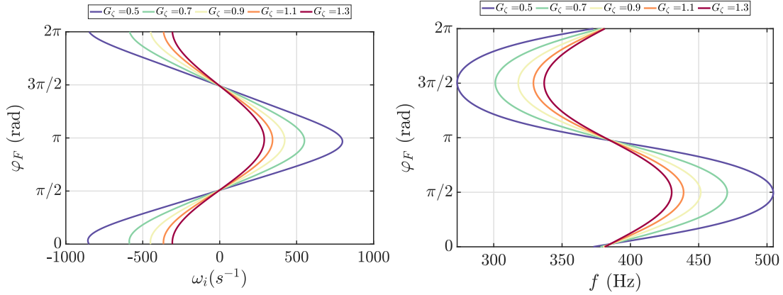
Figure 5.4. Sensitivity of the growth rate \omega_i and frequency f to the magnitude G_\zeta of injector impedance.
