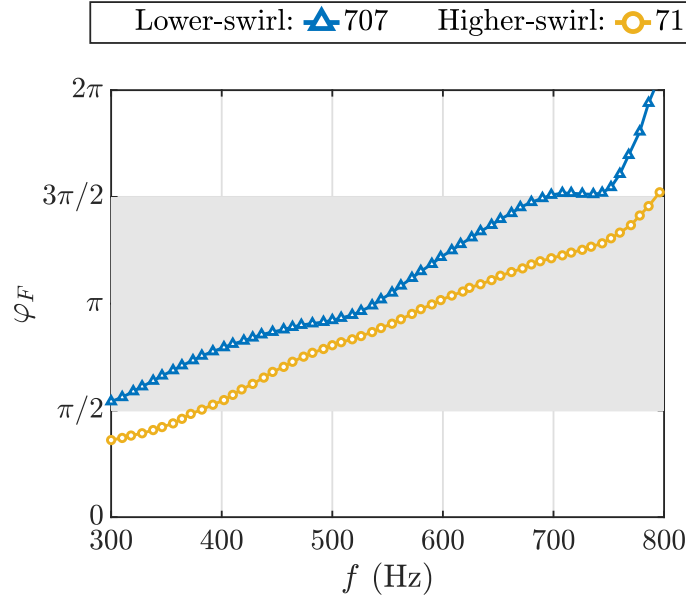
Figure 7.8. FDF phase \varphi_F for swirlers 707 and 716 at \phi = 0.95 and \mathcal{P}_{sicca} = 6.4 kW (operating point F2) in SICCA-Spray. Only the phase evolution with the maximum attainable relative velocity fluctuations at all frequencies are shown.
