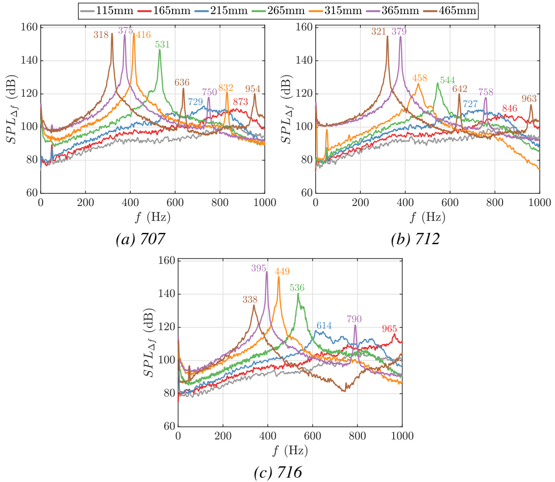
Figure 6.3. Frequency spectra showing the sound pressure level ( SPL_{\Delta f} ) measured by microphone MCI near the combustor backplane for the three swirlers at different combustion chamber lengths l_c .
