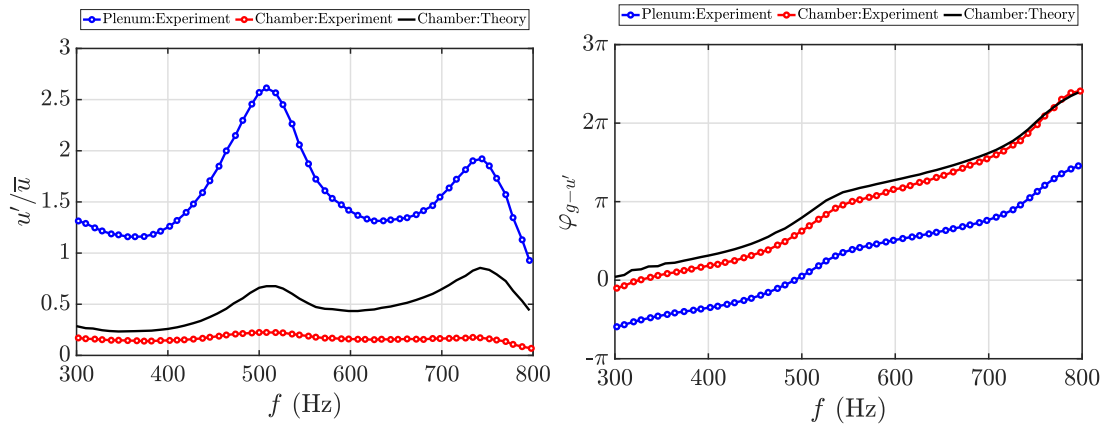
Figure 4.2. Left: The evolution of relative velocity fluctuations measured in the plenum and chamber close to the injector exit along with a comparison of the theoretically deduced chamber relative velocity fluctuations at different frequencies. Right: Phase between velocity and reference generator signal for velocity measured in the plenum, chamber and theoretically deduced chamber velocity at different frequencies. Swirler: 716
