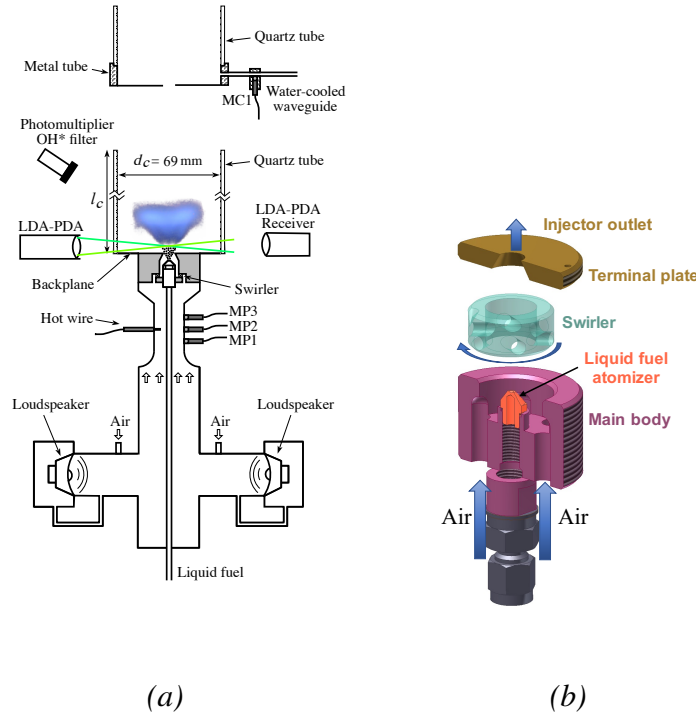
Figure 8.1. (a) Experimental setup of the SICCA-Spray test rig. (b) Exploded view of the injector unit. Reproduced from Chapter 1.
