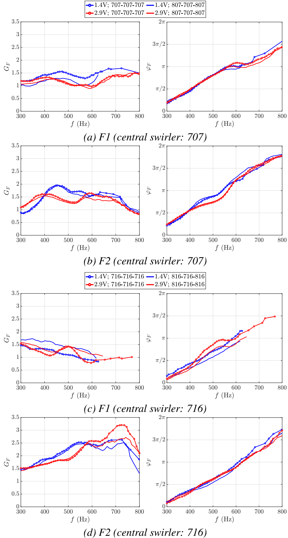
Figure 10.7. Influence of neighboring swirlers: gain G_F and phase \varphi_F of the FDF measured in TICCA-Spray with co- (solid lines with marker) and counter-swirl (solid lines without marker) swirler combinations at the two operating points F1 and F2. Results are presented for two amplifier voltage V_0 = 1.4\text{V} and 2.9\text{V} of the driver units.
