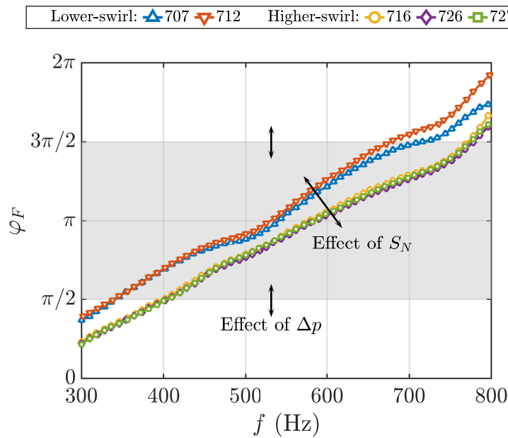
Figure 7.7. FDF phase \varphi_F for the different swirlers considered in this study. Only the phase evolution of Fig. 7.6 corresponding to the maximum attainable relative velocity fluctuations are shown. The swirlers 707 and 712 belong to the lower-swirl category while the swirlers 716, 726, and 727 belong to the higher-swirl category.
