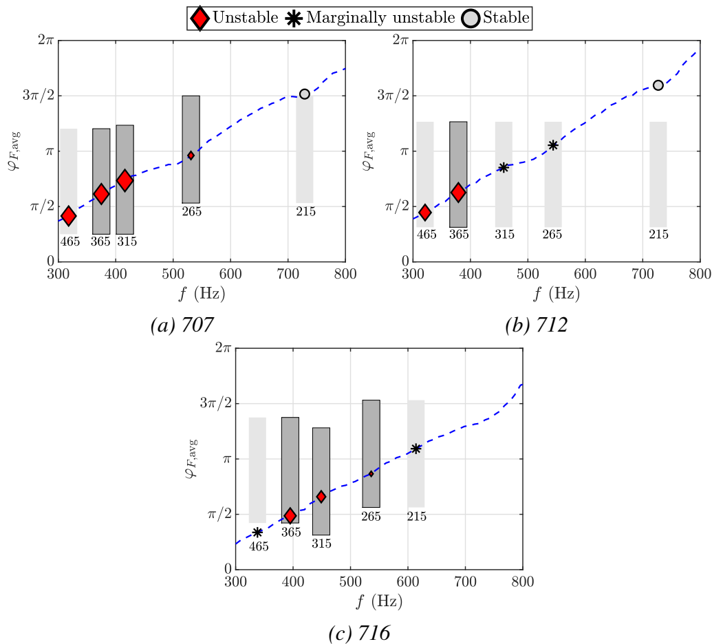
Figure 6.9. Instability bands (marked in gray) predicted by the model are shown at self-sustained oscillation (SSO) frequency for the three swirlers. The combustion chamber length l_c is quoted under each band in mm. The dark gray bands with black outlines correspond to a definite prediction and the light gray bands refer to an approximate prediction. For the unstable points (black diamonds with red shading), the size of the marker is proportional to the RMS chamber pressure p_{rms} . The blue dotted line represents the phase of the FDF averaged over the fluctuation level \varphi_{F,avg} . The theoretical model provides unstable bands while the FDF phase and the stability of the system are obtained from experiments (also shown in Fig. 6.4).
