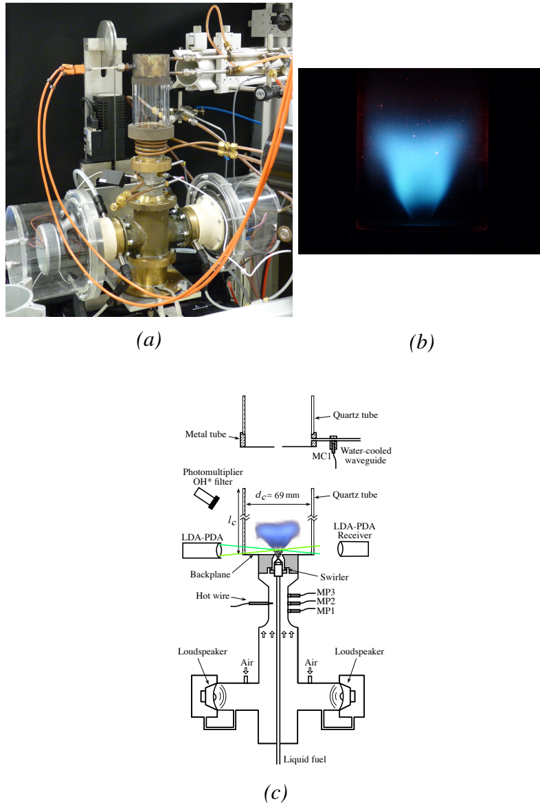
Figure 1.2. (a) A photograph of SICCA-Spray comprising a single sector of the annular configuration. A single flame of the annular combustor is placed in an isolated environment surrounded by a cylindrical combustion chamber. The setup shown here is equipped with different diagnostic tools such as microphones, hot wire, and thermocouple. (b) A photograph of the flame in SICCA-Spray during operation. (c) Schematic of the experimental setup of SICCA-Spray. The figure shows the position of the microphones marked as MP x and the hot wire in the plenum. For the LDA/PDA measurements, a full transparent quartz chamber is used. When measuring the chamber pressure, a metal ring or metal cap is mounted on the chamber to hold the microphone fixed on a waveguide, as shown (a).
