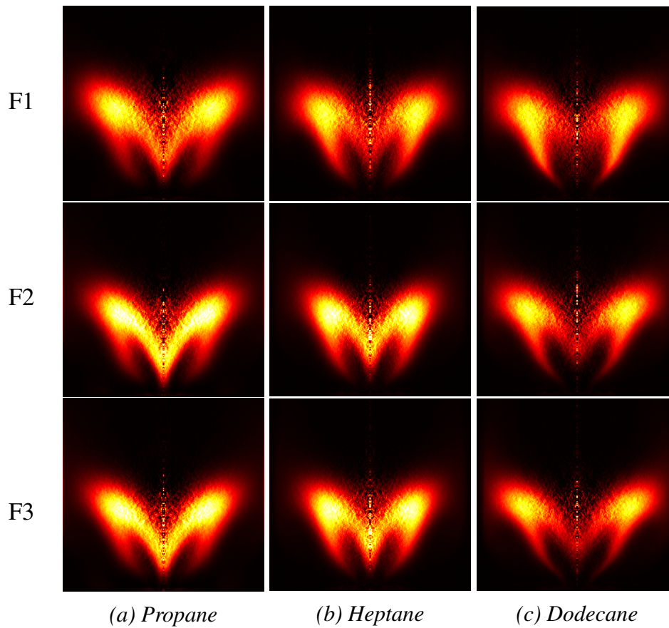
Figure 9.6. SICCA-Spray flame images showing the chemiluminescence of \text{OH}^* captured using an ICCD camera with the different fuels at all three operating points. A single image is obtained by time accumulation of 30 frames and an Abel transform is applied to these images.
