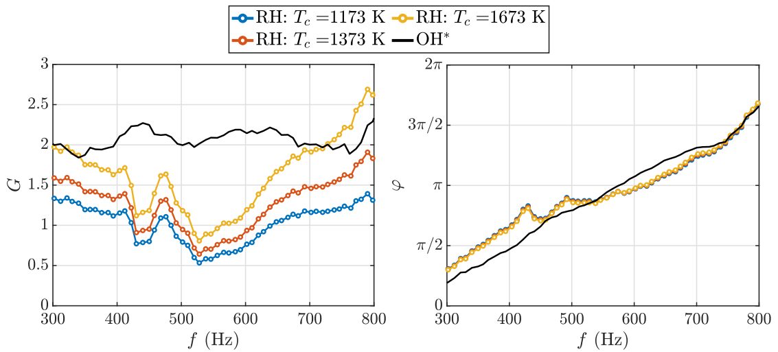
Figure A.5. Sensitivity of flame describing function determined using an acoustic method to the temperature in the chamber T_c . Swirler: 716, h_r = 6.75 mm, operating point: F1, V_0 = 3 V.
