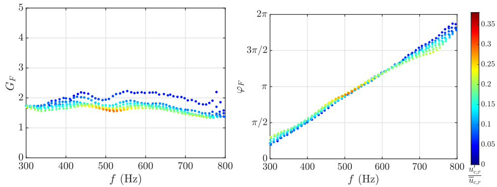
Figure B.3. Flame describing function gain G_F (left) and phase \varphi_F (right) for swirler 713. Relative velocity fluctuations are measured at a radius r = 3.5 mm from the injector center and a height of h = 2.5 mm from the backplane.
