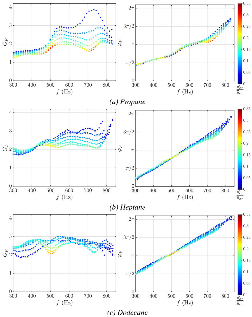
Figure 9.9. FDF (gain G_F and phase \varphi_F ) of the flame describing function in SICCA-Spray for the three fuels at FI ( \mathcal{P} = 6.4\text{ kW} & \phi = 0.85 ) with color axis representing the level of velocity fluctuations u'_{c,r}/\bar{u}_{c,r} at the injector outlet. For the liquid fuels direct FDF is shown, while for the case of premixed propane indirect FDF is displayed. The data are smoothed using a five-point moving average.
