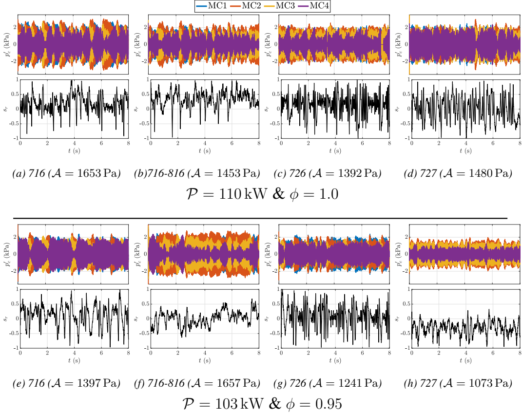
Figure 7.3. Time evolution of chamber pressure p'_c (MC1 to MC4) and spin ratio s_r for 716, the alternate arrangement of 716-816, 726, and 727. Two operating points are chosen from the instability map, where strong instability is exhibited by the four swirler configurations. The pressure-spin ratio set at the top corresponds to \{\mathcal{P} = 110 kW & \phi = 1.0\} , and the bottom set corresponds to \{\mathcal{P} = 103 kW & \phi = 0.95\} .
