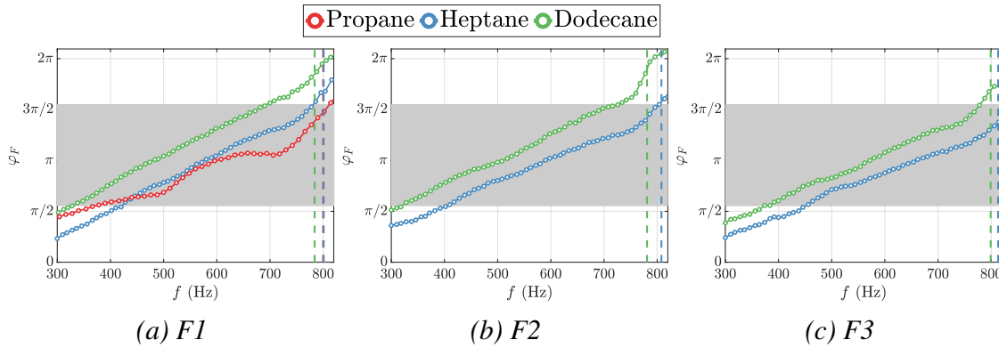
Figure 9.12. FTF phase for the three fuels at V_0 = 3\text{ V} and at the three operating points F1 ( \mathcal{P} = 6.4\text{ kW} , \phi = 0.85 ), F2 ( \mathcal{P} = 6.4\text{ kW} , \phi = 0.95 ) and F3 ( \mathcal{P} = 7.4\text{ kW} , \phi = 0.95 ). Unstable bands are obtained by considering the nearest neighboring impedance (case A) and shown in gray. The dashed vertical lines correspond to the instability frequency of MICCA-Spray. In (a), the dashed lines corresponding to heptane and propane coincide. The instability analysis of propane is only carried out at F1 as a reference case.
