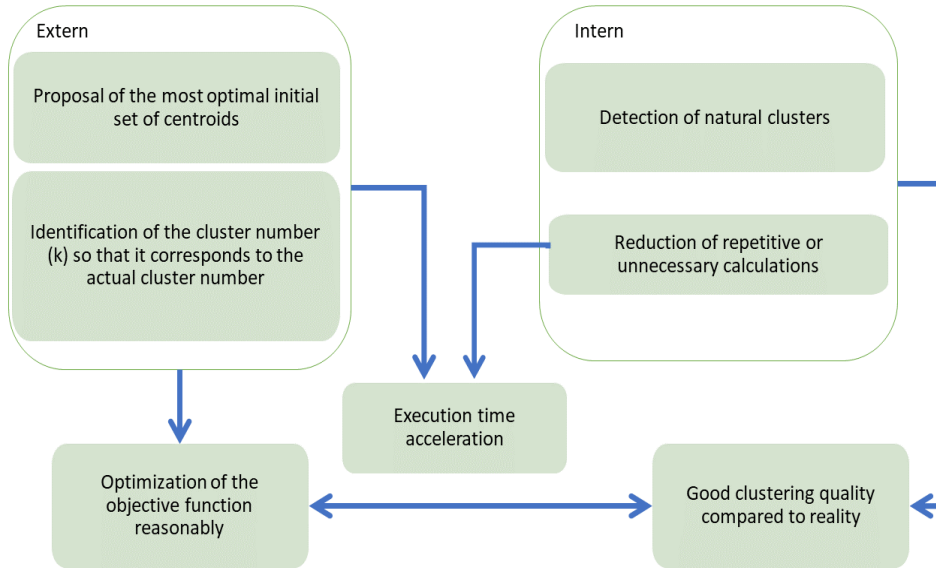
Figure II.2: K-means versatility
