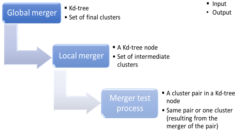
Figure III.14: Merger test process (MTP) is nested in the local merger algorithm, which in turn is nested in the global merger algorithm. MTP could be called multiple times during local merger execution in a node.
