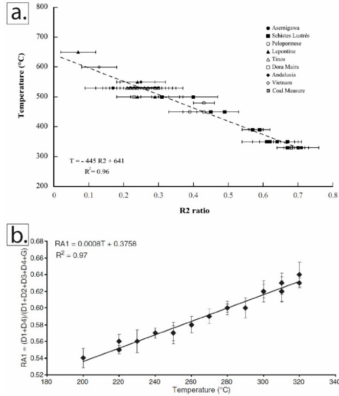
Figure II.4 – Correlation between area ratios and metamorphic temperatures from 200 to 650°C (Modified from (Beysnac et al., 2002; Lahfid et al., 2010)). a. R2 area ratio calibration used by (Beysnac et al., 2002) for the thermometer calibration in high grade metamorphism b. RA1 area ratio calibration used by (Lahfid et al., 2010) for the thermometer calibration in low grade metamorphism
