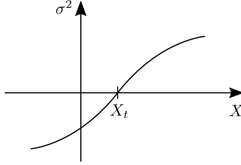
Figure 4.2: Sketch of the evolution of \sigma^2(X) in the inter-vane channels.
