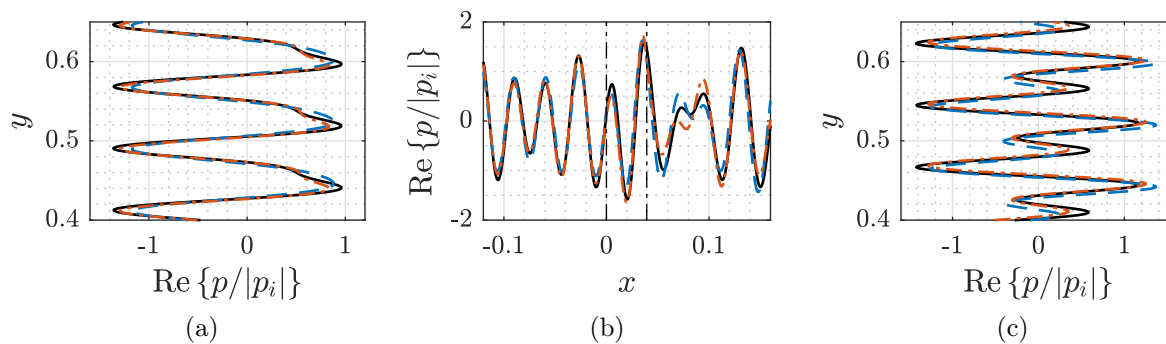
Figure 3.24: Instantaneous pressure profiles computed with FEM (—), MMBCW/Stagger (--) and MMBCW/Camber (-.-) for j = -18 and kb = 5.5 , extracted at x = -0.04 m (a), y = 0.013 m (b) and x = 0.08 m (c). The vertical dash-dotted lines in (b) represents the LE and TE interfaces.
