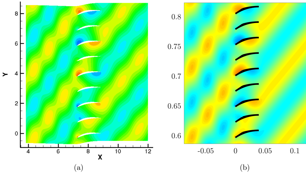
Figure 3.27: Instantaneous pressure maps computed with BASS (a) and MMBCW with a Kutta condition (b) for j = -12 at kb = 2.75 , M_\infty = 0.4 . Color scales are not equal.
