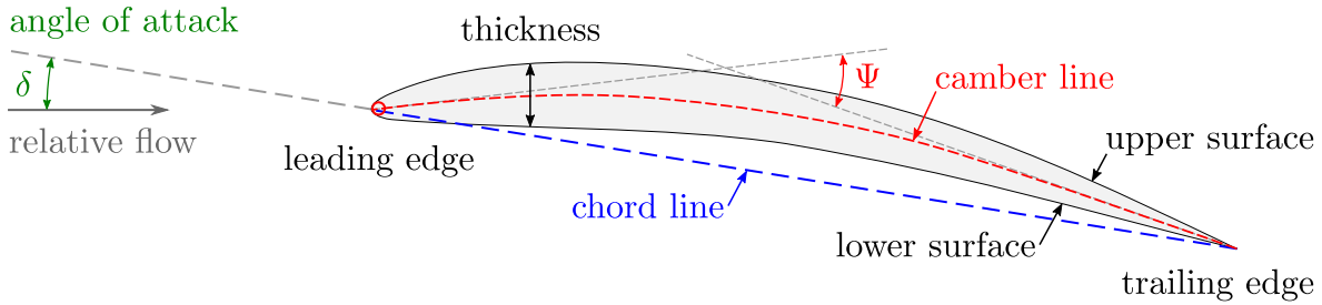
Figure 1.5: Definition of the vane profile.
