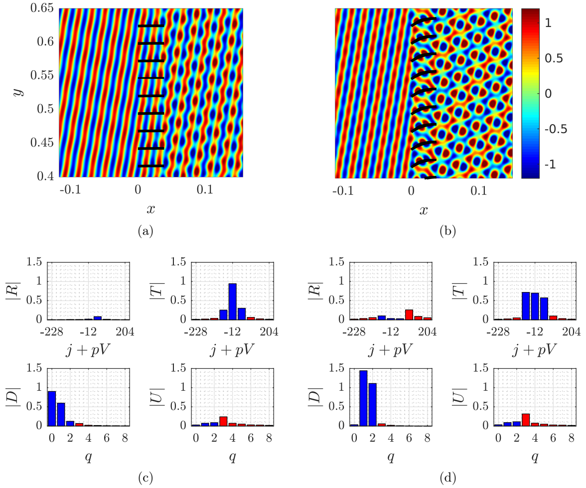
Figure 3.34: Pressure maps and corresponding modal contents without flow ( M_{-\infty} = 0 ), for an incident mode order j = -12 at kb/\pi = 2.7 , a solidity value l/b = 1.5 and a camber angle \Psi = 1^\circ (a,c) or \Psi = 34^\circ (b,d).
