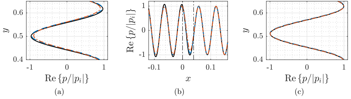
Figure 3.22: Instantaneous pressure profiles computed with FEM (—), MMBCW/Stagger (--) and MMBCW/Camber (-.-) for j = 6 at kb = 2.75 , extracted at x = -0.04 m (a), y = 0.013 m (b) and x = 0.08 m (c). The vertical dash-dotted lines in (b) represents the LE and TE interfaces.
