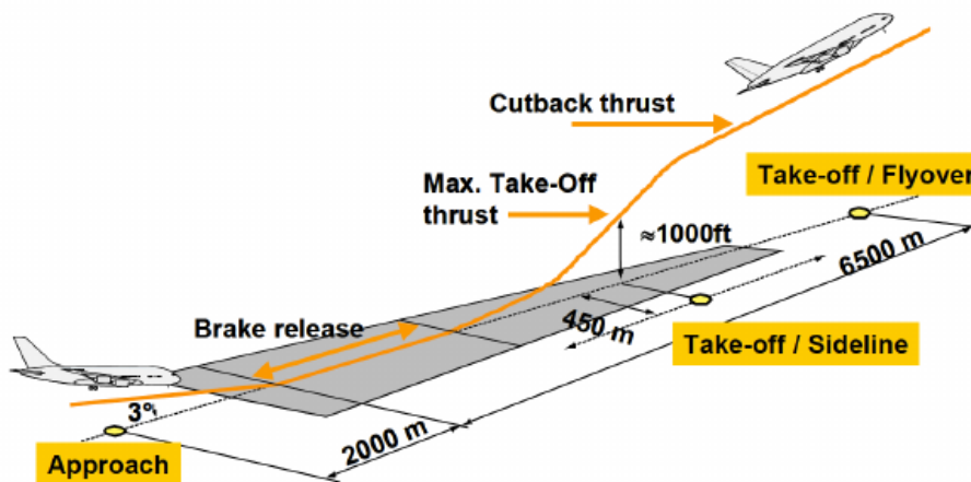
Figure 2: Noise certification flight paths and control points.
