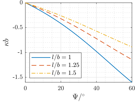
Figure 3.2: Evolution of the dimensionless curvature \kappa b against the camber angle \Psi for different solidity values l/b .
