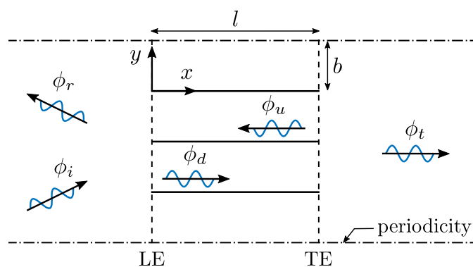
Figure 1.11: Scattering of an incident acoustic wave by a linear cascade of flat vanes.
