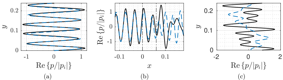
Figure 2.19: Instantaneous pressure profiles using FEM (—) and MMBW (--) for j = 5 at kb = 12.145 , at x = -0.01 m (a), y = 0.04 m (b) and x = 0.07 m (c). The vertical dash-dotted lines in (b) represents the LE and TE interfaces.
