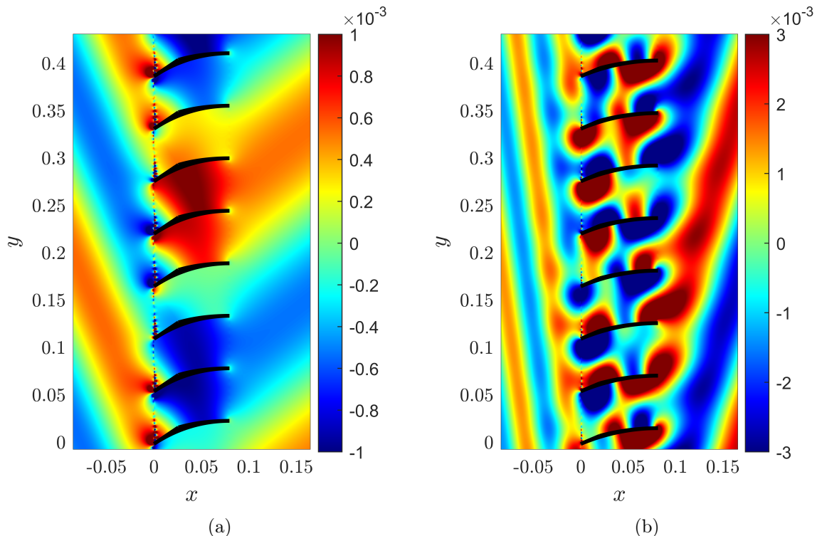
Figure 5.19: Instantaneous pressure field of the resonance (0,0) for \Psi = 34^\circ (a) and (1,1) for \Psi = 23^\circ (b).
