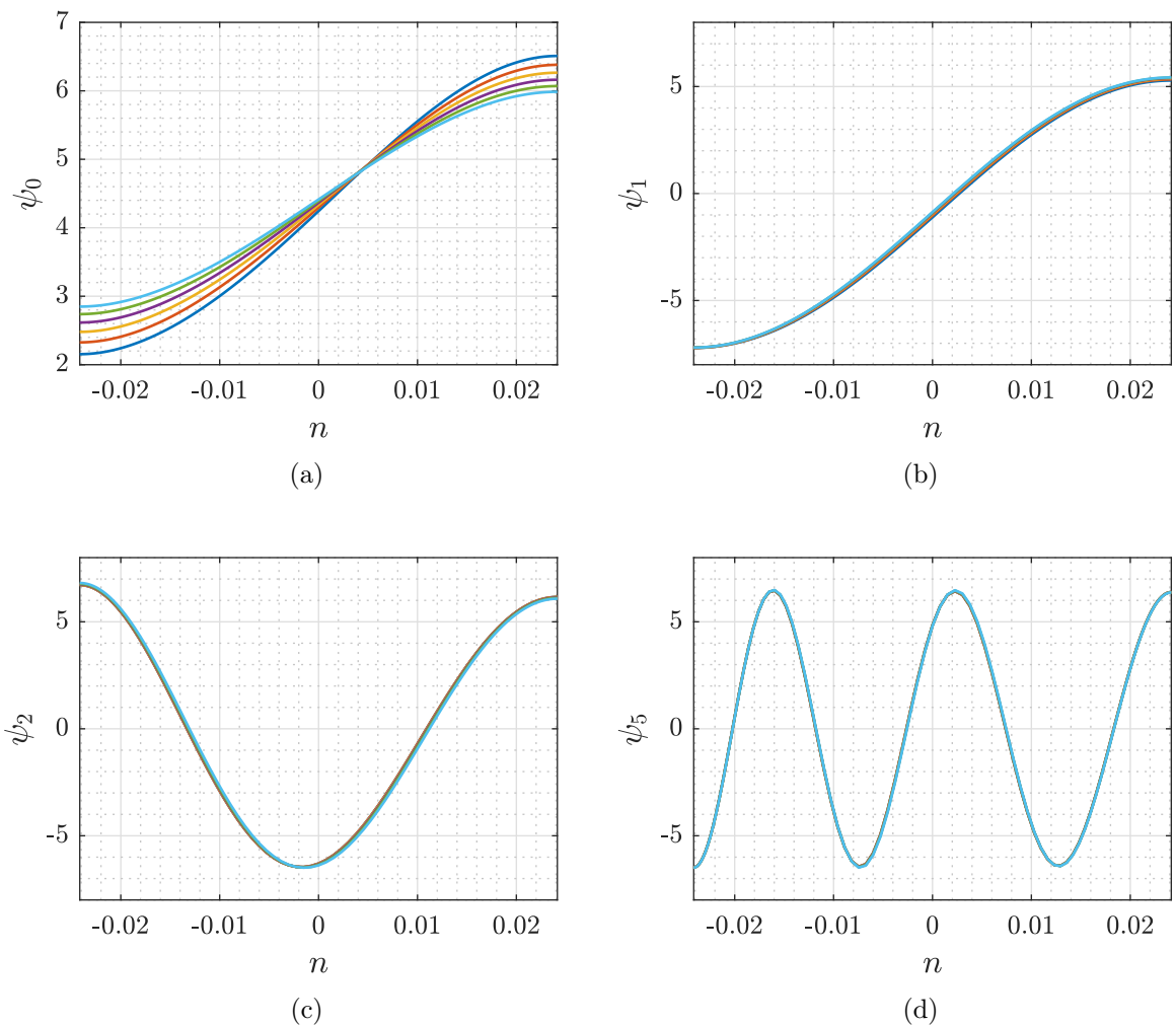
Figure 3.10: Eigenfunctions numerically computed for varying Mach numbers.
