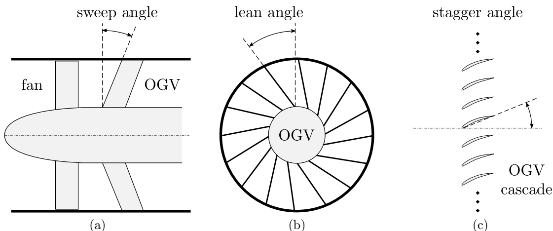
Figure 1.4: Definition of the sweep, lean and stagger angles. Stator in the meridian plane of the bypass duct (a), front view of the stator (b), and unwrapped stator at mid-span (c).
