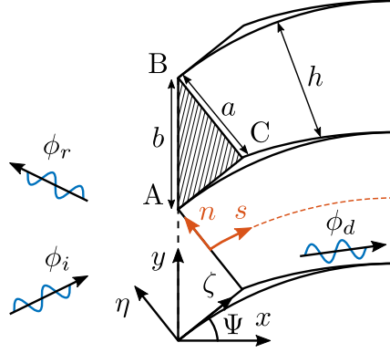
Figure 2.12: Scattering of an incident mode at the staggered leading-edge interface.
