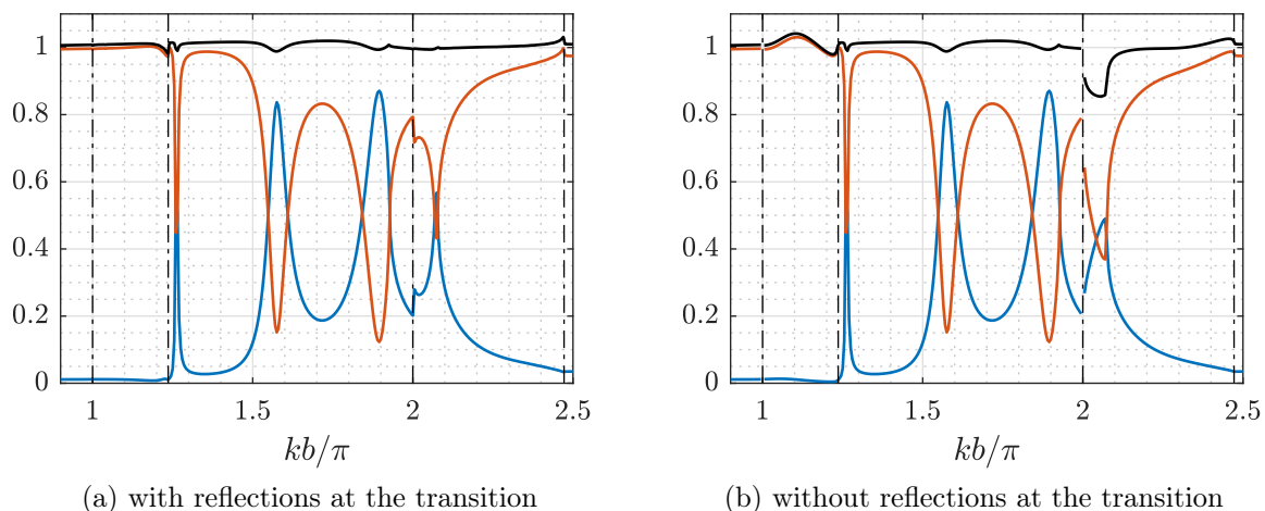
Figure 4.15: Reflected -\mathcal{P}_r/\mathcal{P}_i (—), transmitted \mathcal{P}_t/\mathcal{P}_i (—) and total (\mathcal{P}_t - \mathcal{P}_r)/\mathcal{P}_i powers evolution for j = 2 and \Psi = 36^\circ .
