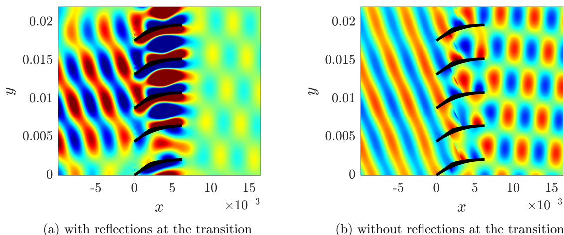
Figure 4.19: Instantaneous pressure maps at the (0,2) resonance for j = 22 and \Psi = 36^\circ .
