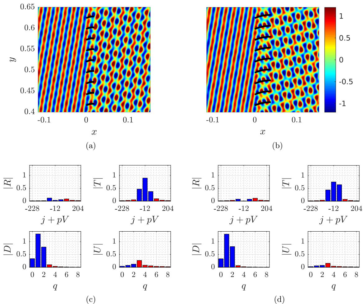
Figure 3.37: Pressure maps and corresponding modal contents without flow ( M_{-\infty} = 0 ), for an incident mode order j = -12 at kb/\pi = 2.7 , a camber angle \Psi = 23^\circ and a solidity value l/b = 0.75 (a,c) or l/b = 1.5 (b,d).
