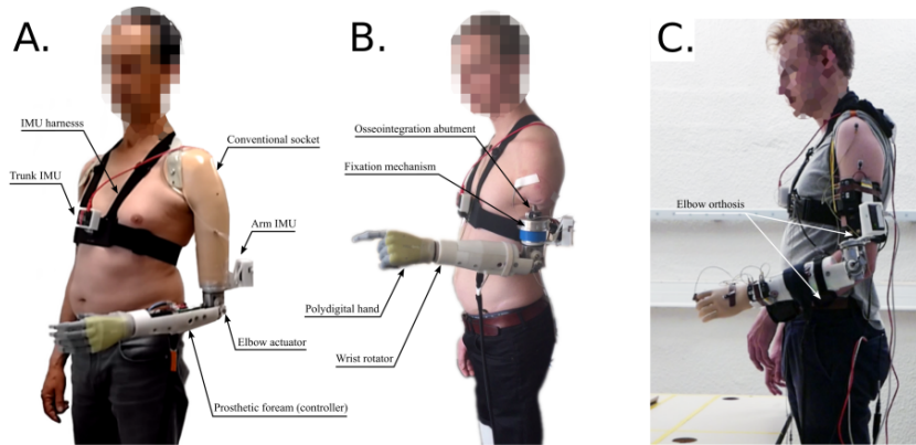
Figure 3.4: A. amputated participant wearing the prosthesis prototype with a conventional external socket. B: amputated participant with the prosthesis prototype plugged to an osseointegrated participant. C: non amputated participant wearing the prosthesis mounted on an elbow orthosis as a substitution arm.
