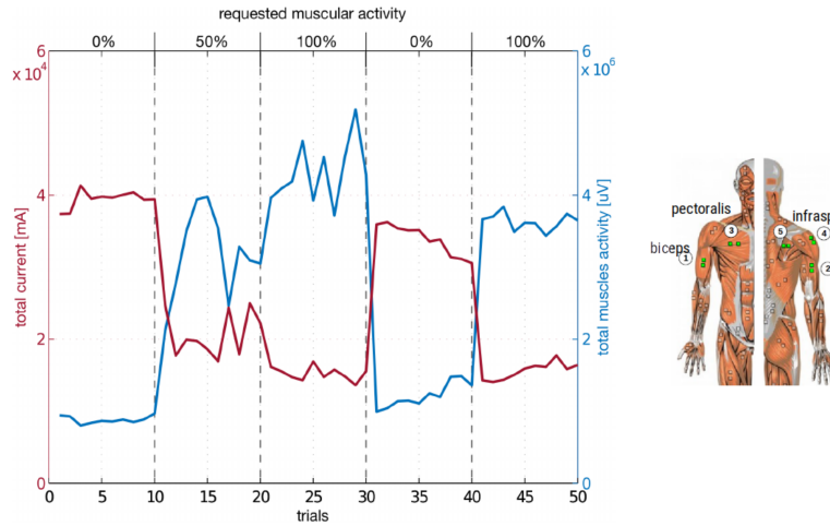
Figure 2.3: Robot adaptation with respect to the human performance. Total muscular activity (blue line) measured over the muscles indicated on the right, and total current from the adaptive PD controller (red line) over the 50 trials. On top of the figure, the percentage of participation (i.e. muscular activity) requested to the subject, trial-by-trial. Taken from [37].
