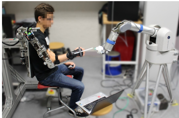
Figure 1.5: View of the experimental setup. On the left, a participant performing a repetitive task while a coordination constraint is applied by the ABLExoskeleton. On the right, the WAM manipulator with the push button represent the variable target to reach.
