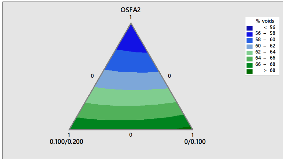
Figure 3-10 – Mixture contour plot analysis of the third round of optimisation which the response analysed is the intergranular porosity (%).
