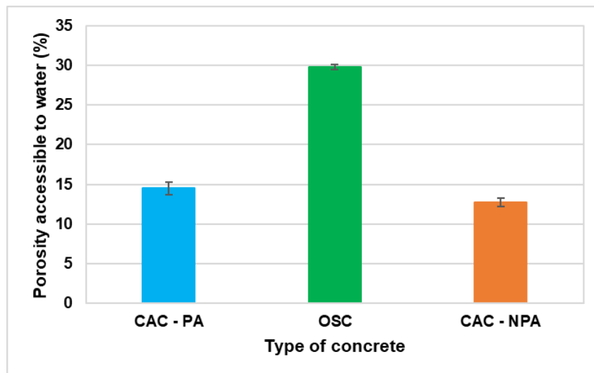
Figure 5-15 – Porosity accessible to water for CAC – PA, OSC and CAC – NPA measured at 90 days aged specimens.
