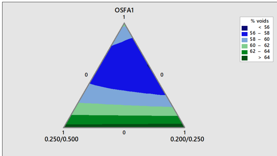
Figure 3-8 – Mixture contour plot analysis of the second round of optimisation which the response analysed is the intergranular porosity (%).
