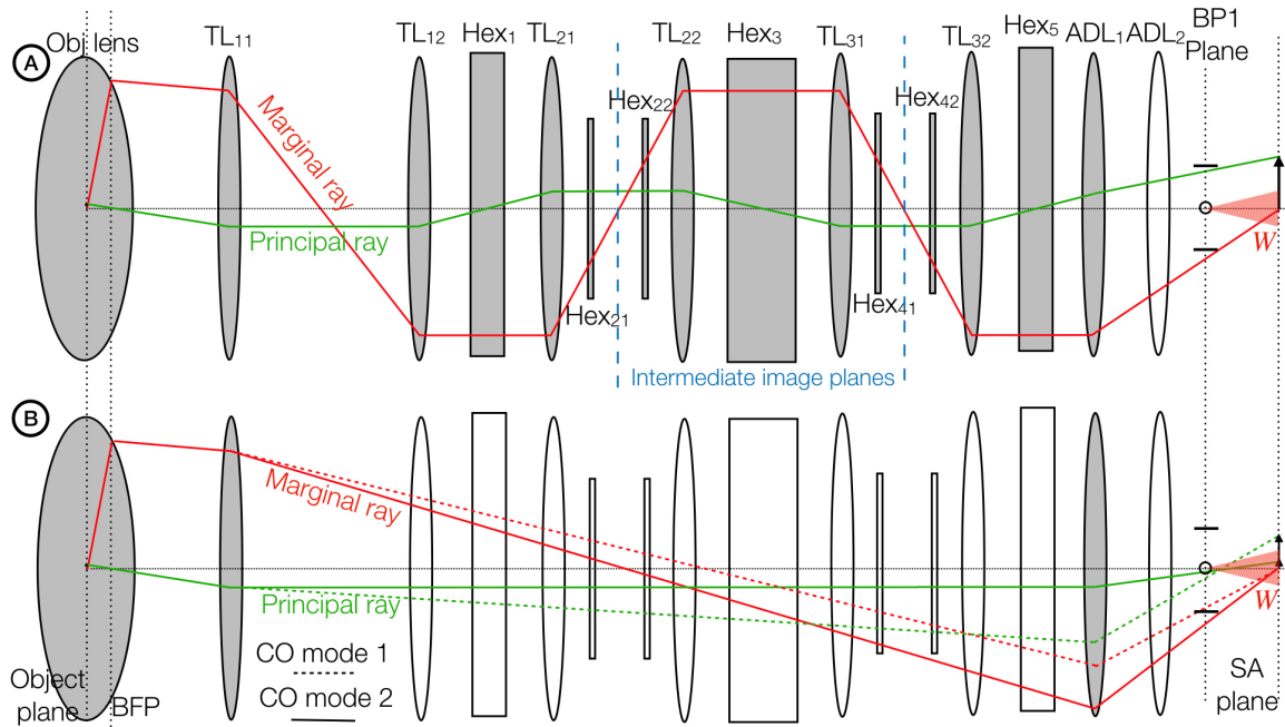
Figure 1.23 Paraxial fundamental rays (principal and marginal rays) inside the I2TEM B COR system. A- Standard aplanatic corrected mode B-Lorentz TL_{11} mode. Two cross-over (CO) modes are represented showing the influence of the B COR optic on the hologram field of view bringing higher flexibility compare to standard TL_{11} mode of a C COR.
