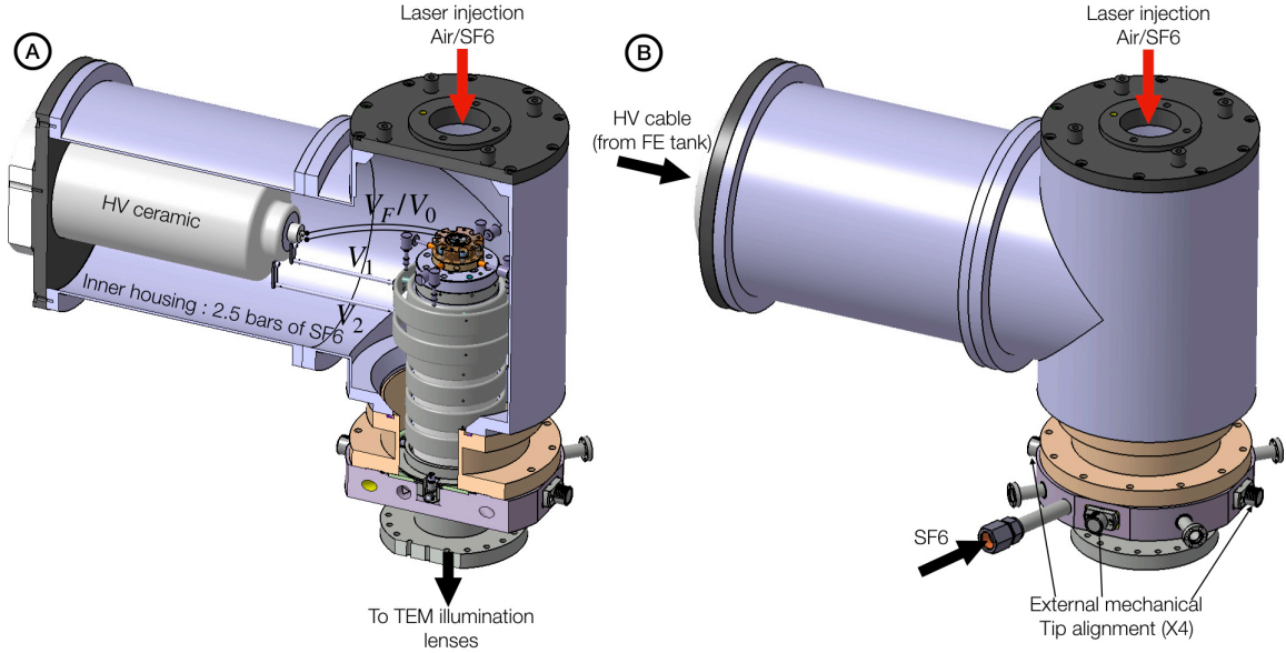
Figure 2.16 CAD drawing displaying the design of the new 200 kV metallic housing filled with 2.5 bars of SF6 gaz. The electric configuration inside the housing is outlined in A. The window located at the top of the housing is used to inject the laser pulse above the gun assembly from the outside to SF6 pressured area.
