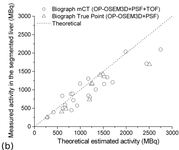
F . 12. For both the Biograph TruePoint and Biograph mCT, total activity in patients vs expected activity (a) and total activity in segmented liver vs expected activity (b), for all reconstruction methods.
