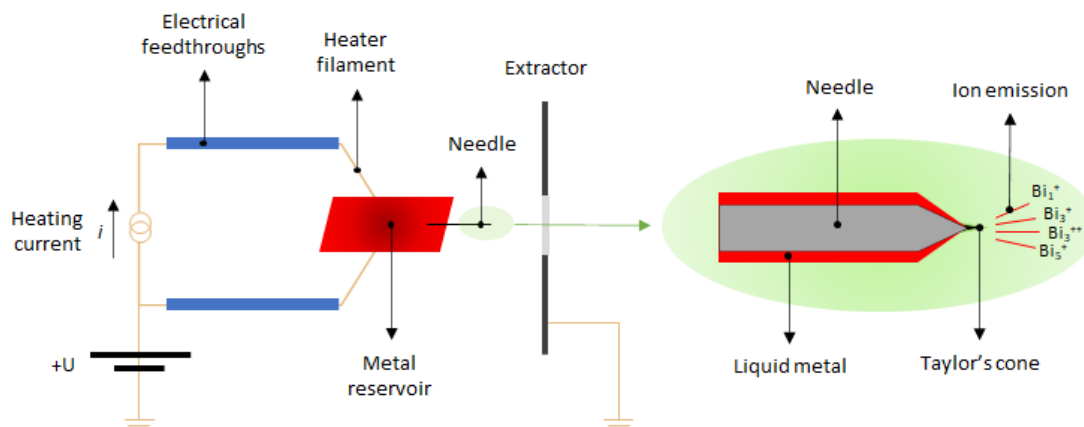
Figure 2.15. Schematic view of a LMIS emitter. [172]
