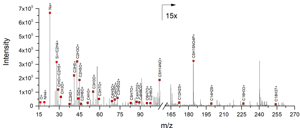
Figure 4.3. ToF-SIMS negative mass spectrum from the large 4 × 3 mm 2 area over the target system containing silicon substrate, biological tissue and the O.C.T. TM Compound.
