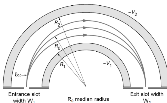
Figure 2.38. Scheme of a 180^{\circ} hemispherical analyser commonly used in XPS. [184]
