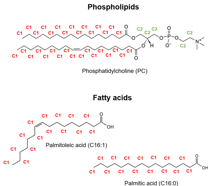
Figure 5.22. Chemical environments of carbon identified in some common phospholipids and fatty acids molecules found in the plasma membrane (PM)-rich region on the slice SA18.
