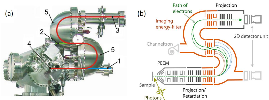
Figure 2.42. (a) Photo and (b) equivalent schematic layout of the NanoESCA Mk1 spectromicroscope (Scienta Omicron) instrument. Three operating modes are possible: (1) direct non-filtered photoelectron emission microscopy (PEEM) mode, (2) selected area spectroscopy or Channeltron mode, and (3) energy-filtered PEEM imaging mode. (4) Indicate the sample position and (5) the hemispherical analyser. Adapted from [192]
