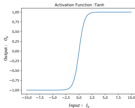
Figure 4.3.3: TanH activation function.
