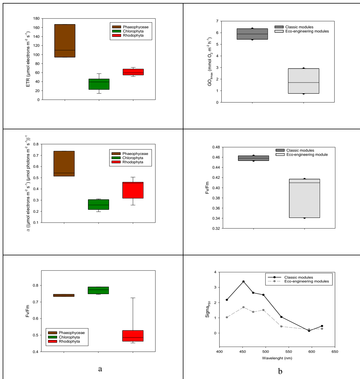
Figure 7. a: ETR, alpha and Fv/Fm measured under water by using Diving PAMII on the dykes modules on Chlorophyta (green algae), Rhodophyta (red algae) and Phaeophyceae (brown algae). b: GO I max , Fv/Fm, and Sigma PSII measured on microalgal biofilm by using LabSTAF. Measurements were performed in the Bay of Cherbourg in April 2021
