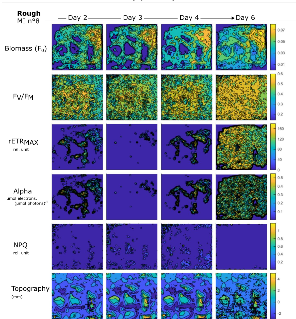
Figure 40 – Spatial distribution of biofilm biomass ( F_0 ) and selected photosynthetic indicators ( F_V/F_M , rETR_{MAX} (relative unit), Alpha ( \mu\text{mol electrons } (\mu\text{mol photons})^{-1} ) and NPQ (relative unit)) and microtopography (mm) on one rough BMI (n°8) during the monitoring period.
