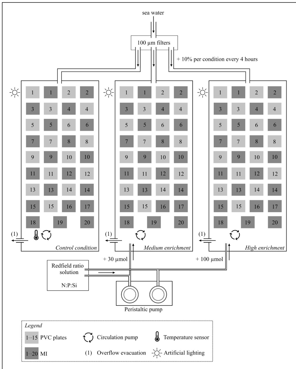
Figure 43 – Experimental setup
