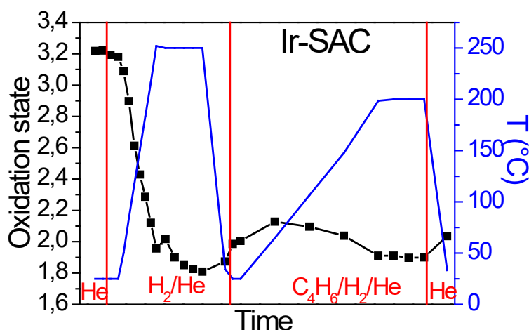
Figure 4. 18: Variation of Ir oxidation state in Ir-SAC in operando XAS conditions.
