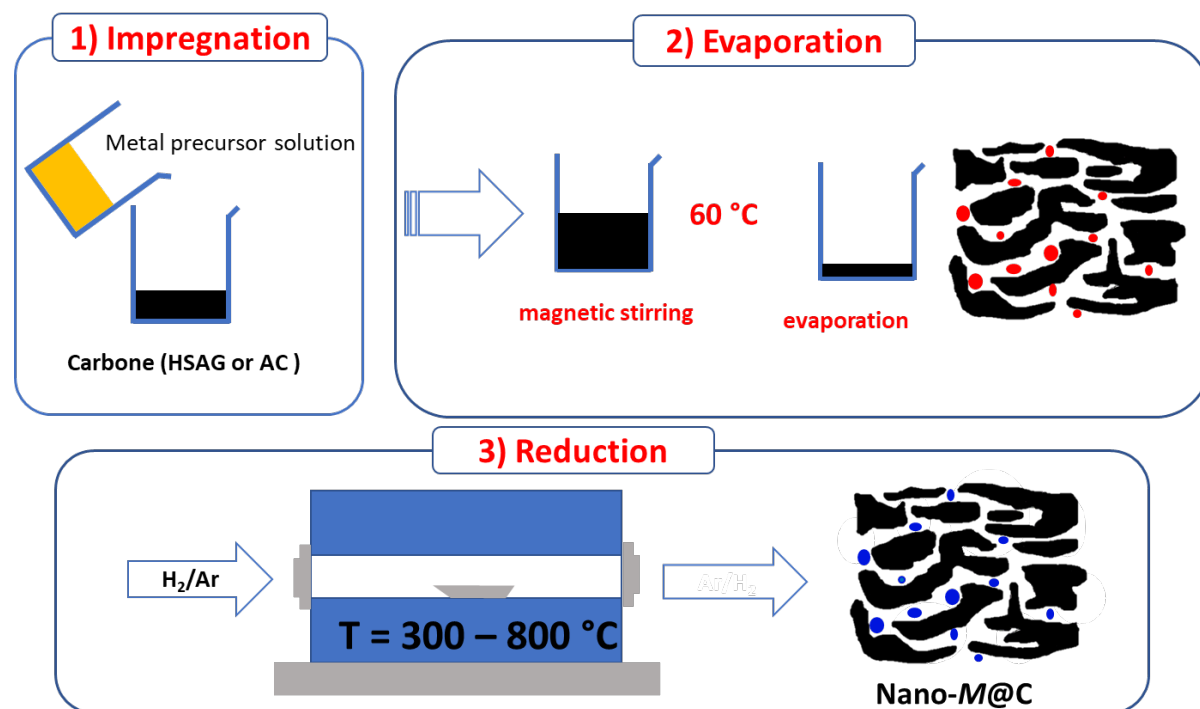
Figure 2. 1: Schematic illustration of the synthesis of metal nanoparticles supported on porous carbon materials.
