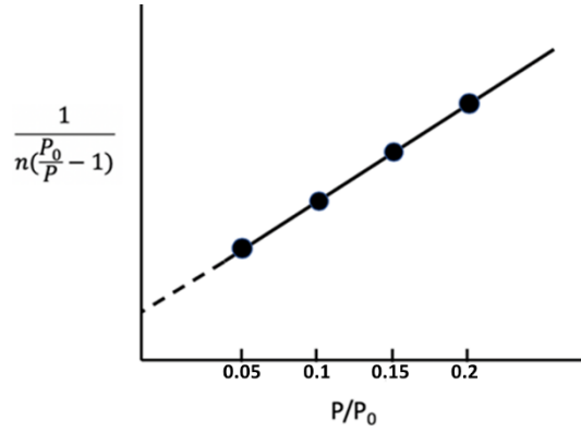
Figure 2. 8: Typical BET plot.
