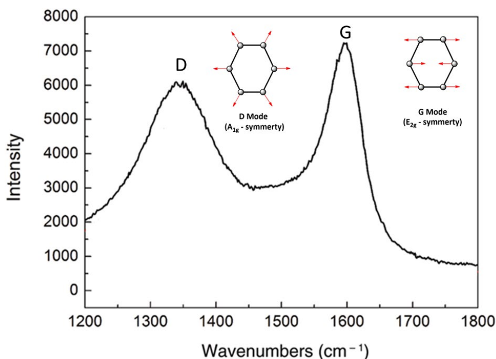
Figure 2. 9: Raman spectrum of activated carbon materials, collected with an excitation \lambda = 514\text{ nm} , and assignment of the main bands. The insets show a scheme of the vibrational modes associated with the two main bands. 5
