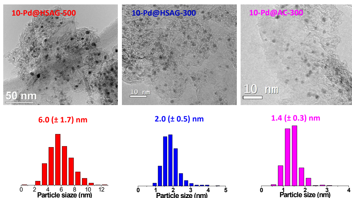
Figure 3. 3: TEM images of 10-Pd@HSAG-500, 10-Pd@HSAG-300 and 10-Pd@AC-300, together with the particle size distribution of Pd nanoparticles.
