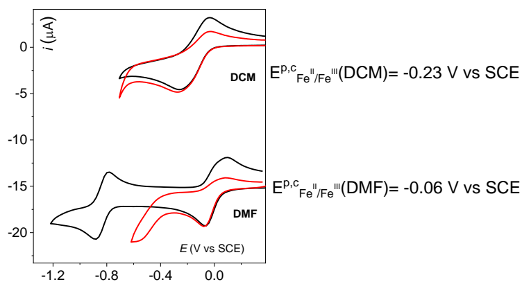
Figure 2.8: CVs of \text{Fe}^{\text{III}}(\text{F}_{20}\text{TPP})\text{Cl} in organic solution of 0.1 M TBAPF 6 at 0.1 V s -1 at a GC electrode (0.07 cm 2 ), T = 293 K; Under Ar (black trace) and air saturated (red trace), all in 0.5 mM porphyrin solutions. Up: CVs in DCM. Down: CVs in DMF.
