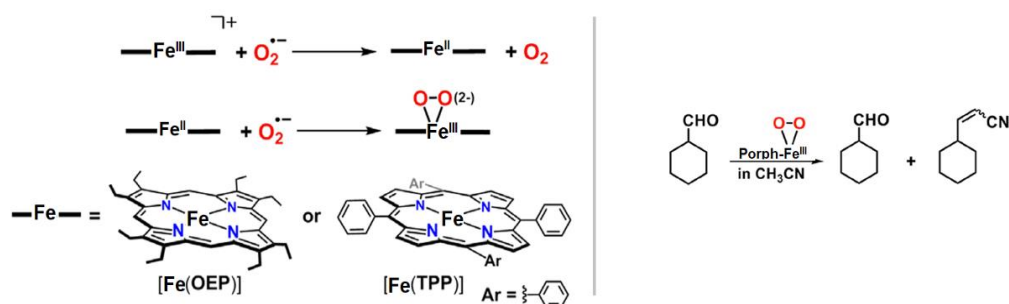
Figure 1.9: (Left) Generation of ferric porphyrinate peroxy species by Valentine 56 (Right) reactivity of ferric peroxy as reported by Watanabe. 59
