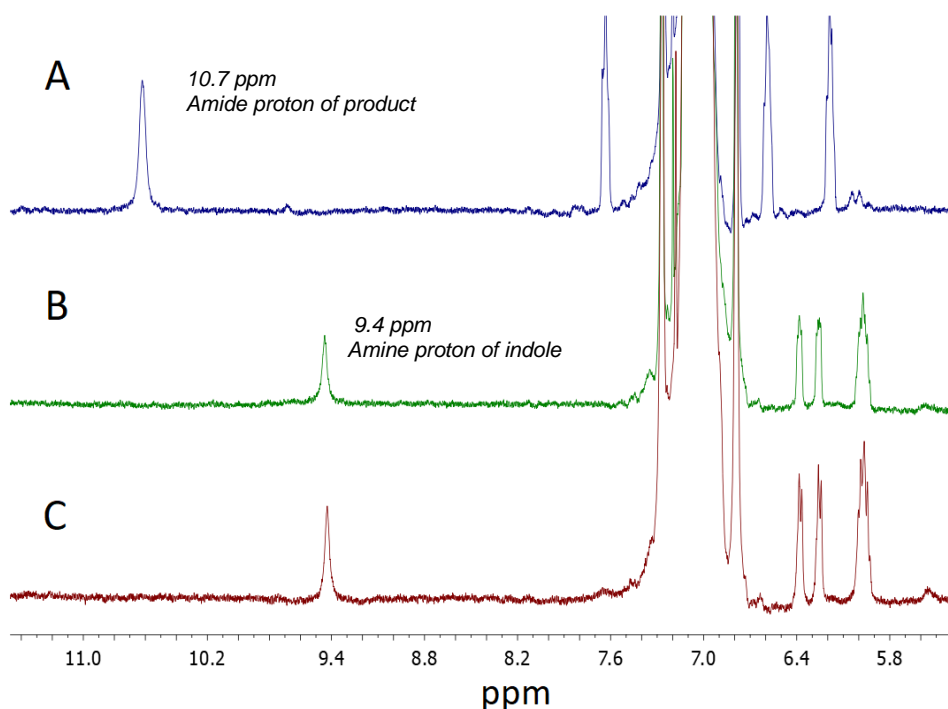
Figure 5.3 A: 1 H-NMR spectra of the synthesized N -2-(methylphenylacetamide) in a solution of 4:2 DMF/CDCl 3 . B: 1 H-NMR spectra of air saturated solution of Fe(TPP)Cl with 2,3-dimethylindole in presence of 0.1 M TBAPF 6 after electrolysis at -0.2 V vs SCE for 1h. C: Before electrolysis. For C and B 0.2 mL CDCl 3 were added in 0.4 mL of sample in DMF.
