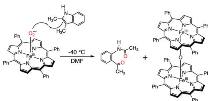
Figure 1.8: System developed by Goldberg et al. for dioxxygenation of 2,3-dimethylindole. 55
