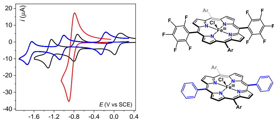
Figure 2.1:(Left) CV of an Ar saturated DMF solution of 1 mM Fe^{III}(F_{20}TPP)Cl (black trace), and CV of a DMF solution of 1 mM of Fe^{III}(TPP)Cl in the same conditions (blue trace). CV of 1 mM solution of O_2 (air saturated, red trace). All solutions contained 0.1 M TBAPF_6 , and CVs were recorded at a glassy carbon (GC) disk electrode (with an area of 0.071 \text{ cm}^2 ), at 0.1 \text{ V s}^{-1} and T = 293 \text{ K} . (Right) molecular structures of Fe^{III}(F_{20}TPP)Cl and Fe^{III}(TPP)Cl .
