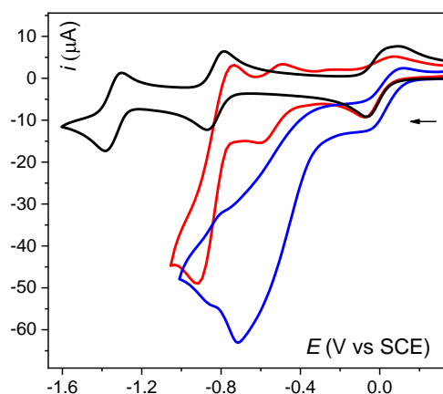
Figure 3.1: CVs at GC disk electrode (area 0.07 \text{ cm}^2 ) of 1 \text{ mM} solution of \text{Fe}^{\text{III}}(\text{F}_{20}\text{TPP})\text{Cl} in DMF with \text{TBAPF}_6 ( 0.1 \text{ M} ), \nu = 0.1 \text{ V s}^{-1} , T = 293 \text{ K} ; under Ar (black trace), under \text{O}_2 (air saturated, 1 \text{ mM} ) (red trace) and under \text{O}_2 with 10 \text{ mM HClO}_4 (blue trace).
