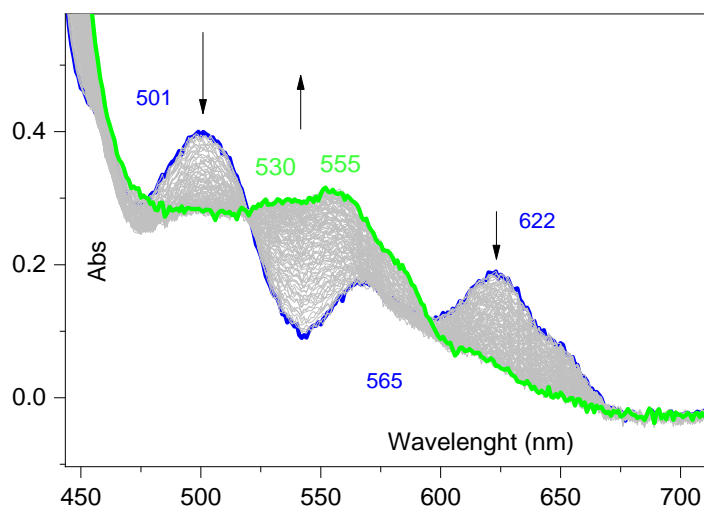
Figure 3.11: UV-Vis spectra of \text{Fe}^{\text{III}}(\text{F}_{20}\text{TPP})\text{Cl} (0.5 mM) in DMF with \text{TBAPF}_6 (0.2 M), T = 258 \text{ K} , under \text{O}_2 (air saturated) with \text{HClO}_4 (0.5 mM) at open circuit potential (blue trace) and at -0.20 \text{ V} vs. SCE after 5 min (green trace). Grey traces are intermediate spectra.
