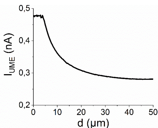
Figure 7.7: Approach curved obtained in a SECM set-up with a velocity of 1 \mu\text{m s}^{-1} , in a DMF solution with 0.1 M TBAPF6 and 0.25 mM of \text{Fe}^{\text{III}}(\text{F}_{20}\text{TPP})\text{Cl} under argon. A potential of -0.4 V vs Ag/AgCl is holded in the UME resulting in reduction of \text{Fe}^{\text{III}} to \text{Fe}^{\text{II}} while in the generator substrate a potential of -0.5 V vs Ag/AgCl is applied resulting in oxidation of \text{Fe}^{\text{II}} to \text{Fe}^{\text{III}} .
