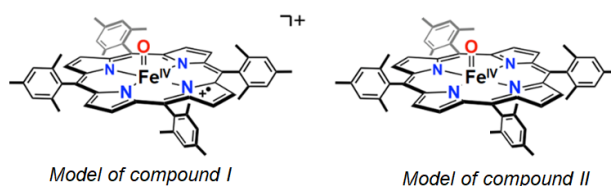
Figure 1.14: High valent species \text{Fe}^{\text{IV}}(\text{O}) \pi radical cation (left, Compound I) and \text{Fe}^{\text{IV}}(\text{O}) of the FeTMP porphyrin (right, Compound II).
