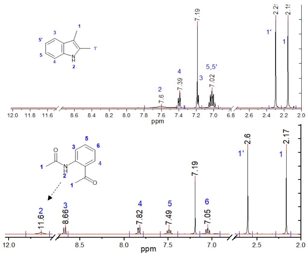
Figure 5.1 ^1\text{H-NMR} spectra of 2,3-dimethylindole (Up), and the N -2-(methylphenylacetamide) (Down). In the insets are shown the molecular structures of the two complexes. Peak at 7.19 ppm corresponds to the solvent, \text{CDCl}_3 . 1 and 1' numbers correspond to three methyl-protons.
