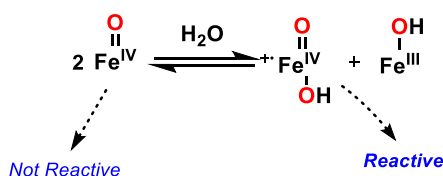
Figure 1.16: Disproportionation reaction that takes place between high valent Fe oxo species in non-dry solvents and in water, as described by Newcomb. 94
