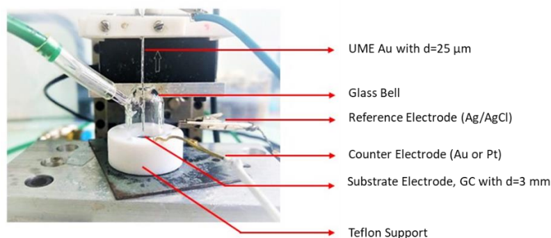
Figure 7.6: Set-up used for Scanning Electrochemical Microscopy Experiments.
