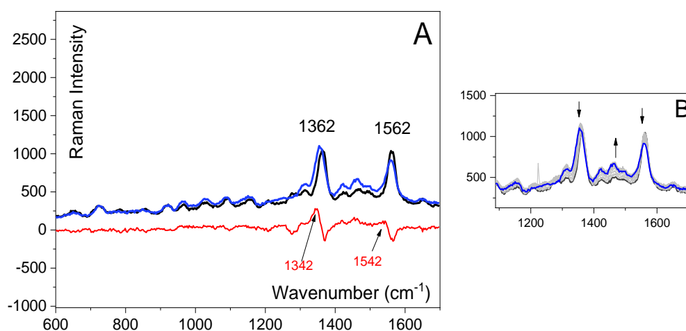
Figure 6.2: A: Resonance Raman spectrum of an acetonitrile solution of 0.1\text{ M} \text{TBAPF}_6 of 0.5\text{ mM} \text{Fe}(\text{F}_{20}\text{TPP})\text{Cl} before (black), and after (blue trace) the application of -0.3\text{ V} vs SCE under Ar. Red trace represents the different of the before and after spectra. Excitation at 406\text{ nm} . B: Marker band region of the spectra recorded during the electrolysis (blue and black traces are identical with (A)).
