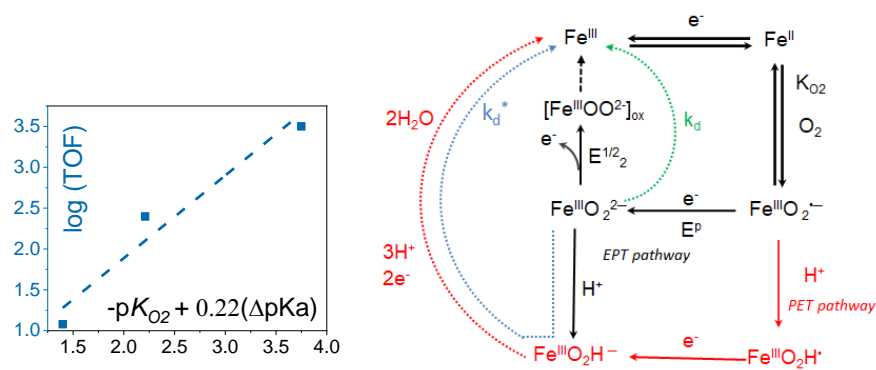
Figure 4.15 Left: Dependence of the TOF on a factor containing both K_{O_2} and pK_a of the peroxo based on the equation \log(\text{TOF}) = -pK_{O_2} + a pK_{a_{\text{Fe}^{\text{III}}\text{OO}^-}/\text{Fe}^{\text{III}}\text{OOH}} + B'' with B'' and a constant terms within the series. Right: Reaction scheme displaying different reaction pathways considered.
