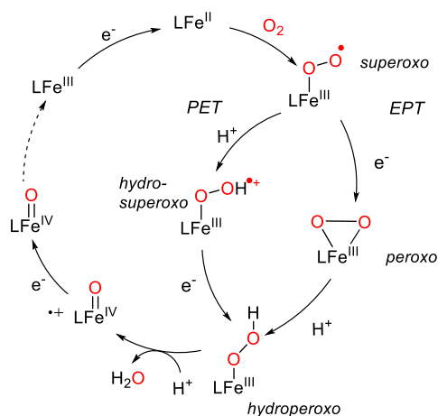
Scheme 3.1: Proposed catalytic cycle of \text{O}_2 reductive activation by \text{Fe}^{\text{III}}(\text{F}_{20}\text{TPP})\text{Cl} . Total charges of intermediates and axial ligands are omitted for clarity.
