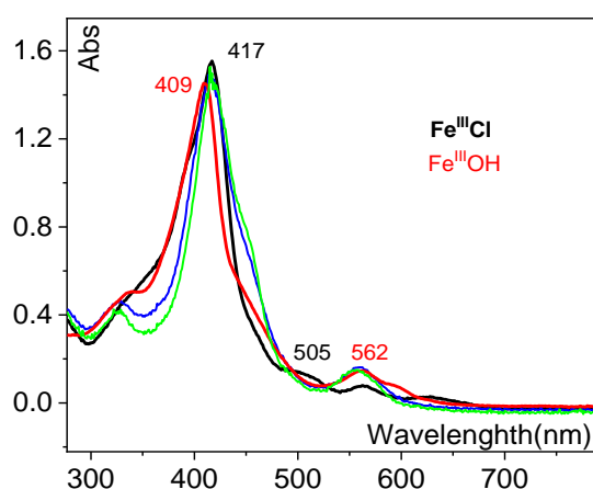
Figure 4.10: Spectra of a 0.2 mM Fe III (F 20 TPP)Cl at 253 K in an air saturated DMF solution with 0.2 M TBAPF 6 in the spectroelectrochemical cell before (black trace) and after electrochemical generation of the peroxo by applying -0.6 V vs SCE for 10 min, and subsequent decomposition in open circuit (blue trace). Second electrolysis of that solution at -0.6 V vs SCE and subsequent decomposition in open circuit leads to the green trace spectrum. A chemically prepared Fe III OH is also shown in the figure for comparison (red trace).
