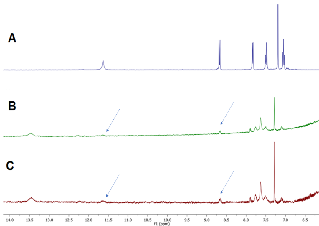
Figure 5.4: A: solution of the synthesized product N-2-(methylphenylacetamide) in 0.1 mL CDCl 3 in with 0.5 mL of DCM B: 1 H-NMR spectra of air saturated solution of Fe(TPP)Cl with 2,3-dimethylindole in presence of 0.1 M TBAPF 6 after 1h electrolysis at -0.35 V vs SCE. C: before electrolysis. For C and B 0.1 mL CDCl 3 is added in 0.5 mL of sample in DCM.
