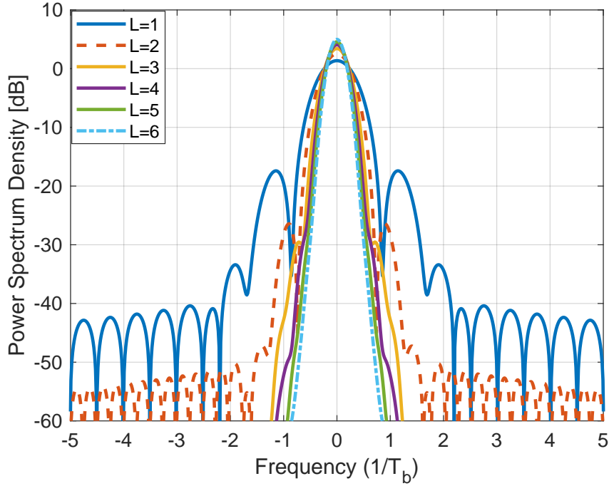
Figure 1.11 – Power spectral density of binary RC with h = 0.5 and for L = \{1, 2, 3, 4, 5, 6\} .
