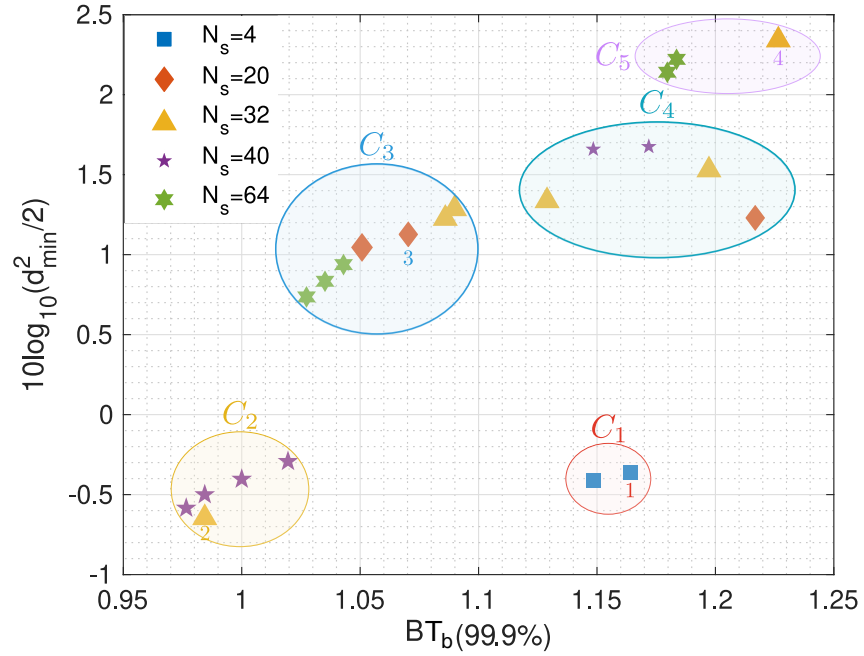
Figure 3.4 – Three Pareto optimum objective functions configurations for LSSB-FSK using B_{99} .
