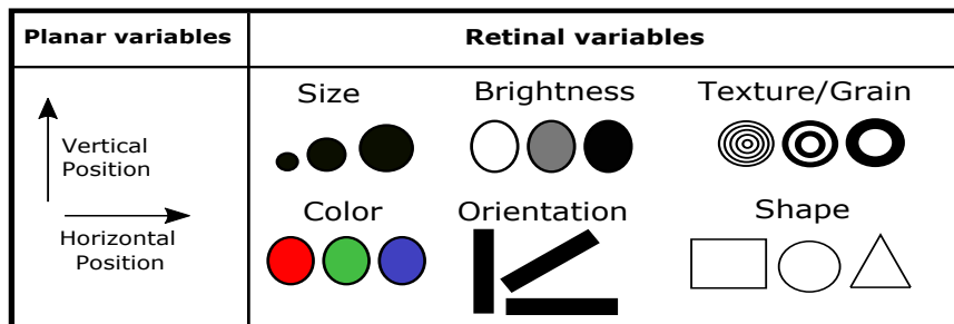
Figure 3.4: Visual variables
