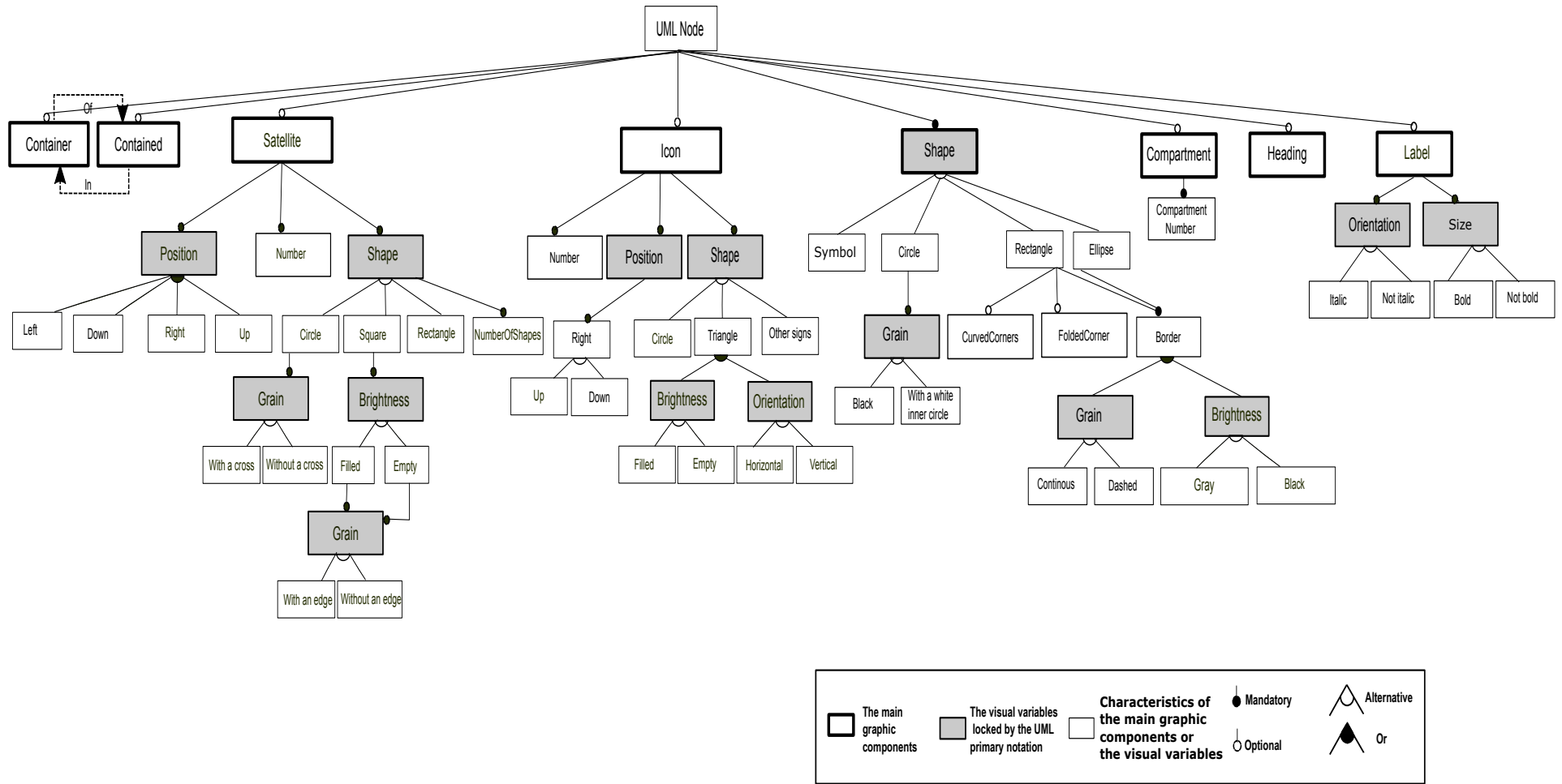
Figure 4.1: Cartography of the UML graphic nodes and the used visual variables.
