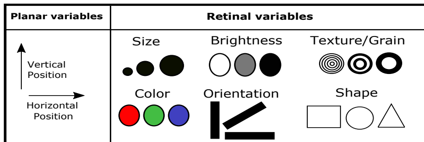
Figure 3.4: Visual variables
