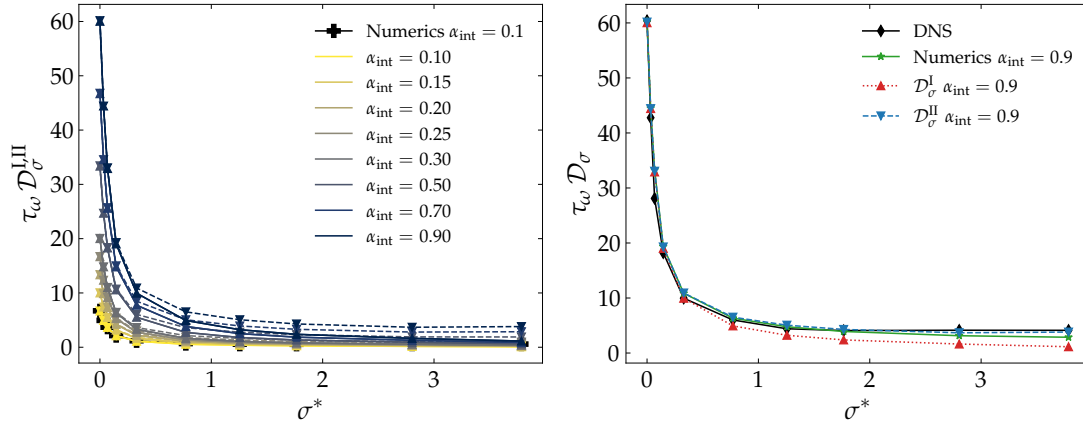
Figure 3.18: Left panel: Measurements of diffusion coefficient \mathcal{D}_\sigma^I in Eq.(3.81) (continuous line with upper triangular markers) and \mathcal{D}_\sigma^{II} in Eq.(3.84) (dotted line with lower triangular markers) for different values of the tuning parameter \alpha_{\text{int}} (as in legend). In black cross marked line corresponds to the model result by integrating numerically Eq. (3.44) for the tuning parameter \alpha_{\text{int}} = 0.1 . Right panel: Measurement of the diffusion coefficient \mathcal{D}_\sigma : in DNS (in black diamond line), in the model according to Eq. (3.81) (in red upper triangles marker dotted line), in the model according to Eq. (3.81) (in blue lower triangles marker dashed line), and in the model result by integrating numerically Eq. (3.44) (in green starred marker line), for the tuning parameter \alpha_{\text{int}} = 0.9 , as a function of \sigma^* . The numerical integration for the model has been performed using an Euler–Maruyama scheme with an integration time-step \Delta t = 5 \cdot 10^{-4} and with a final time T = 1000 .
