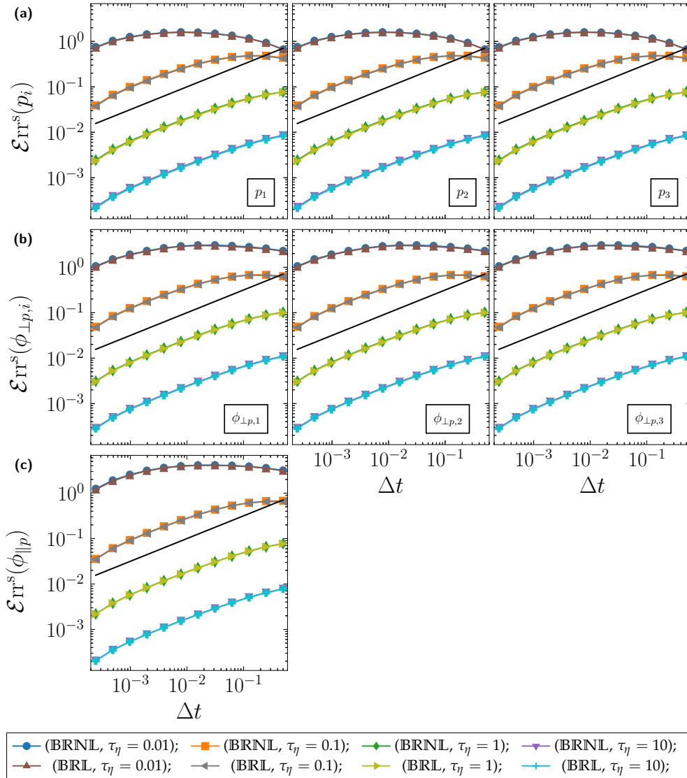
Figure B.6: Splitting scheme in HIT: Strong error ( \mathcal{E}_{rr^s} ) of the splitting algorithm Eq. (4.96) using the numerical scheme in Eq. (4.93) followed by Eq. (4.89) (BR – BSNL) and Eq. (4.95) followed by Eq. (4.89) (BR – BSL), against the time step \Delta t for different values of \tau_\eta . In (a) the three components of \mathbf{p} , (b) the first component \phi_{\perp p} of tumbling and (c) the spinning \phi_{\parallel p} . Black line indicates the slope 1/2; and the initial condition of particle orientation is \mathbf{p}_b^0 = (1, 1, 1)/\sqrt{3} .
