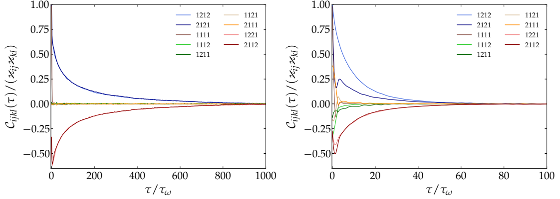
Figure 3.11: Correlations of the fluid velocity gradient tensor renormalised by their standard deviation \varkappa_{ij} = \langle A_{ij}^2(0) \rangle^{1/2} as a function of time-lag \tau . Left panel: \sigma^* = 0 . Right panel: \sigma^* = 2.8 .
