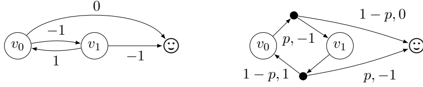
Figure 5.4 – On the left, a game with no negative cycles where \sigma_{\text{Min}}^p is optimal. On the right, the MC obtained when playing along \sigma_{\text{Min}}^p .
