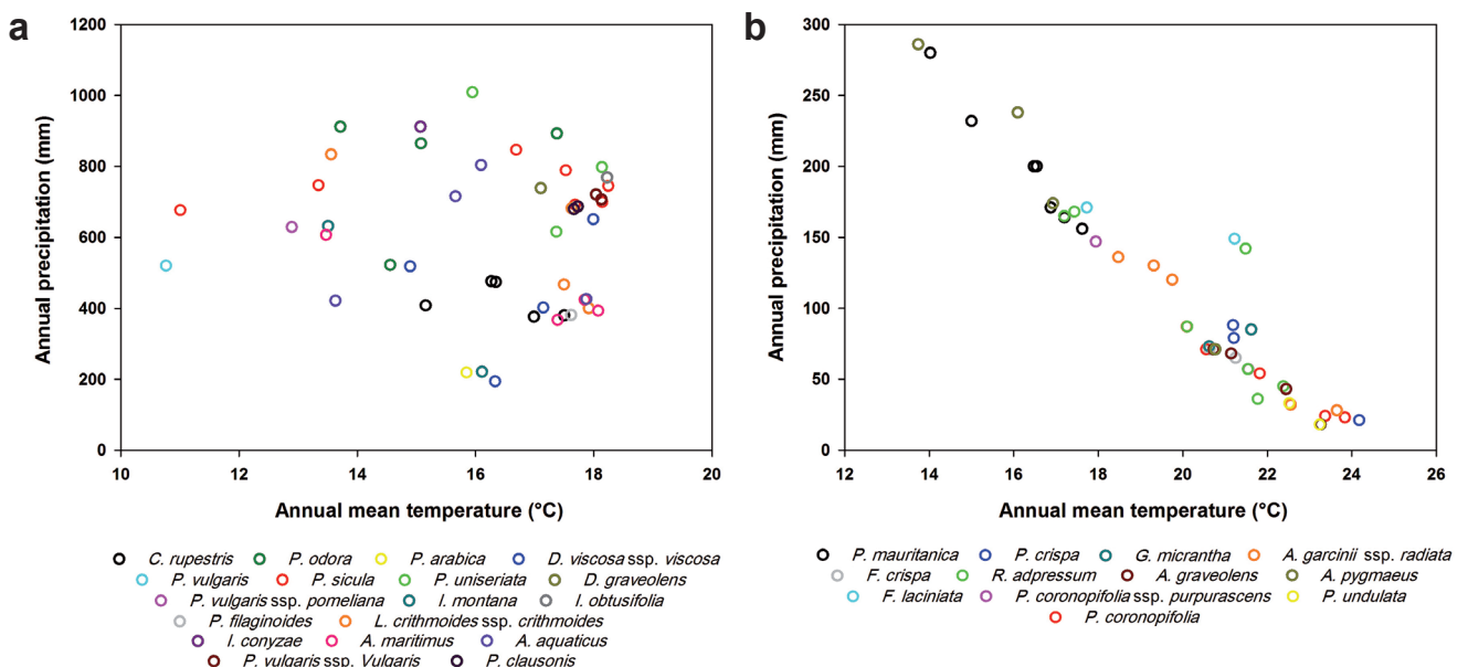
Fig. 2. Two-dimensional niches of various species of the Algerian tribe Inuleae Explanations: a – the Tell species, b – the Sahara species
