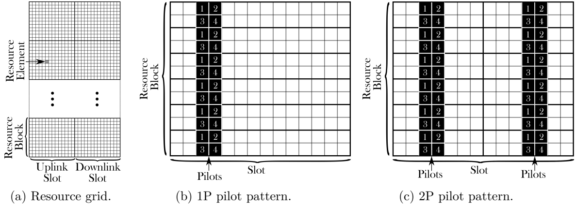
Figure 5.1: Pilots are arranged on the RG according to two different patterns, where each number corresponds to a different transmitter.
