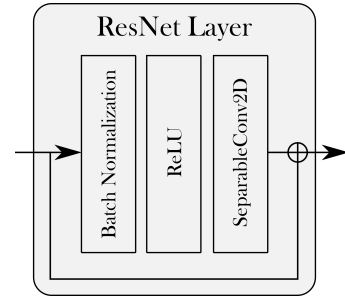
Figure 5.12: ResNet layer.
