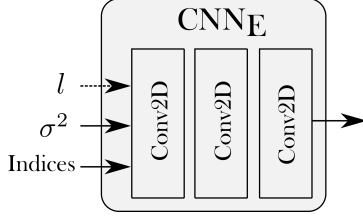
Figure 5.13: Architecture of \text{CNN}_{\mathbf{E}} .
