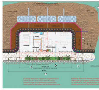
Global Model Earthship One Bedroom One Bathroom Construction Drawings
