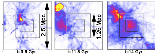
Fig. 13. X-ray weighted metal maps for model cluster B at different times. The movement of the metals with respect to the X-ray surface brightness centre (fixed at the image centre) due to several cluster mergers can easily be seen.
