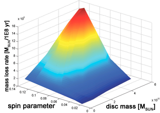
Fig. 4. The mass loss rate [ M_{\odot}/1 \times 10^8 \text{ yr} ] for simulated galaxies as a function of disk mass and spin parameter ( \lambda ). The halo mass for all galaxies is fixed to 3 \times 10^{11} M_{\odot} . It can clearly be seen that higher disk masses and spin parameter result in a higher mass loss rate. This is due to the fact that higher spin parameters cause a larger disk scale length and therefore a larger disk.
