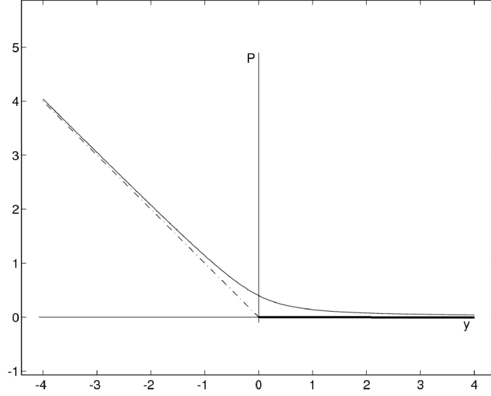
Figure 2.1: Hyperbolic Penalty
