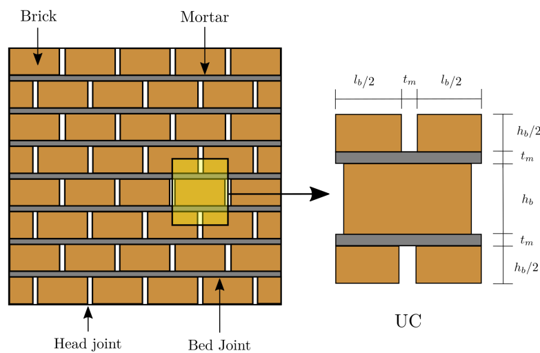
Figure 3.14: Schematic of periodic masonry structure with mortar joints in pattern HD and periodic unit cell selected from the structure and used for the nonlinear finite element based homogenization analysis.
