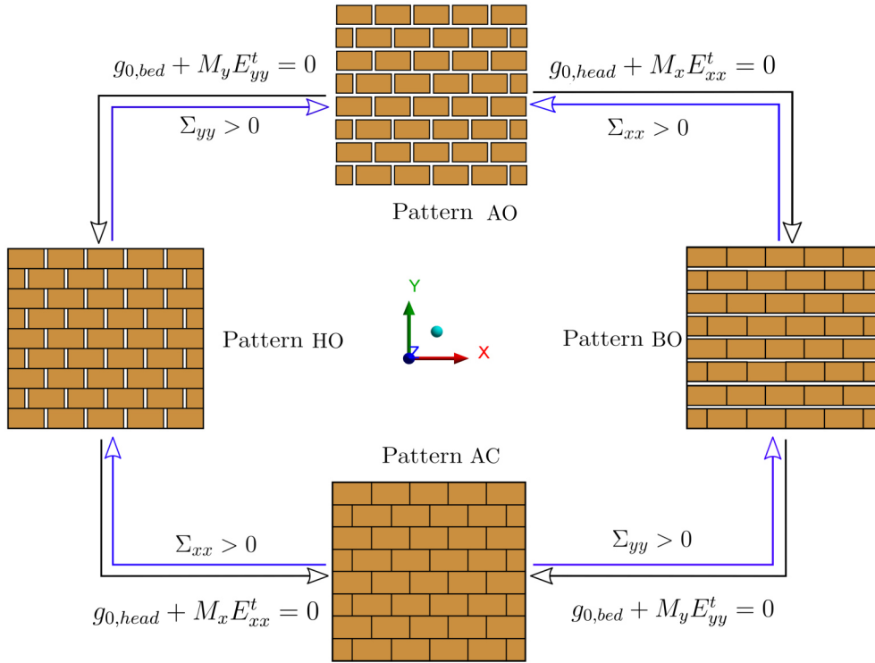
Figure 3.15: Schematics of all possible joint patterns of refractory masonry with dry joints and joints closure and reopening criteria.
