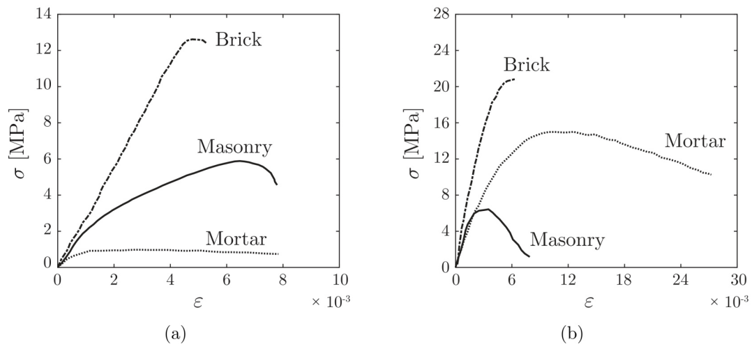
Figure 1.21: Stress-strain curves for mortar, brick, and masonry: (a) weak mortar [99] and (b) strong mortar [98].
