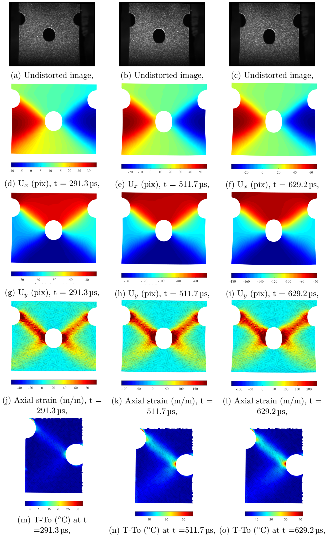
Figure E.1: Undistorted images, displacement fields and strain fields obtained during a dynamic tensile test, for different time steps. 227
