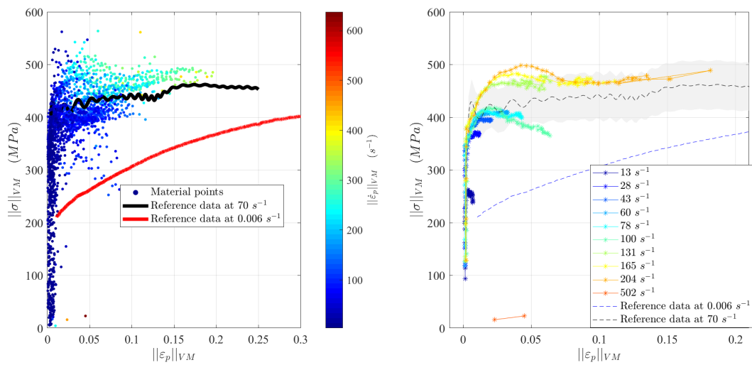
(a) Material states in (\|\boldsymbol{\varepsilon}_p\|_{VM}, \|\boldsymbol{\sigma}\|_{VM}) . The colour of the markers denote the strain-rates, while the lines denote the reference data from ONERA,
