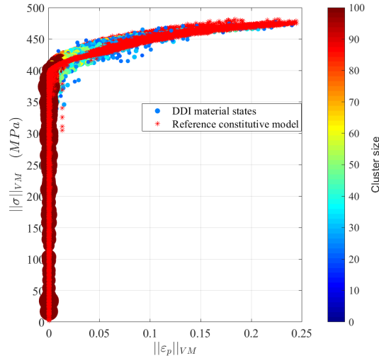
Figure 8.15: Comparison of the DDI material states versus the reference solution (in red) in one projection of the constitutive space ( \|\varepsilon_p\|_{VM} , \|\sigma\|_{VM} ). The marker size and colour for the DDI output are related to the size of the cluster. Only the selected clusters are represented.
