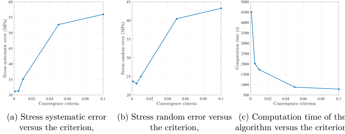
Figure 8.4: Stress errors and computation time evolution according to the criterion.
