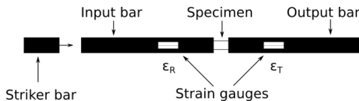
Figure 2.3: Schematic of a classical Split Hopkinson Pressure Bar test apparatus.
