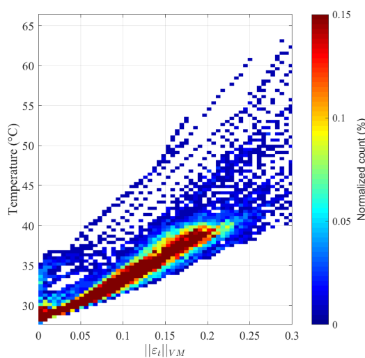
Figure 7.9: Temperature vs Von-Mises norm of the total strain distribution for elements in the main localization band before crack initiation.
