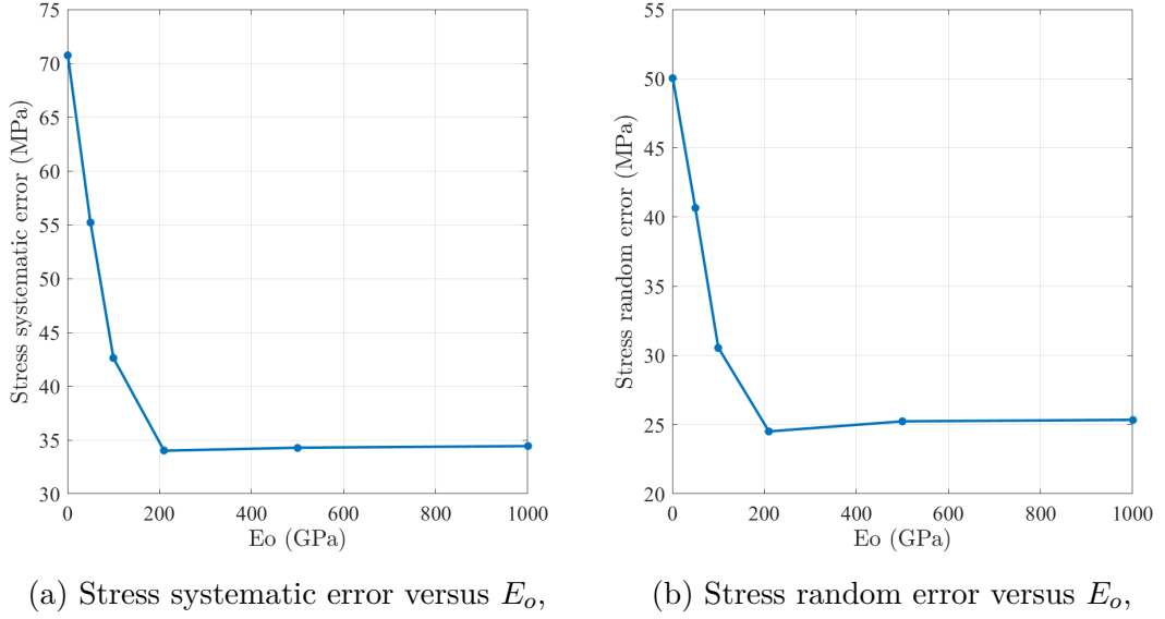
Figure 8.2: Stress errors evolution according to the value of E_o .
