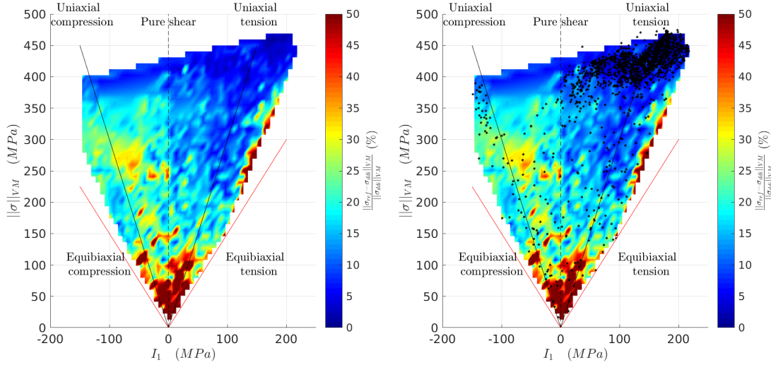
(a) Distribution of the DDI relative error in the space of the stress tensor invariants. (b) With the selected material states in black,
