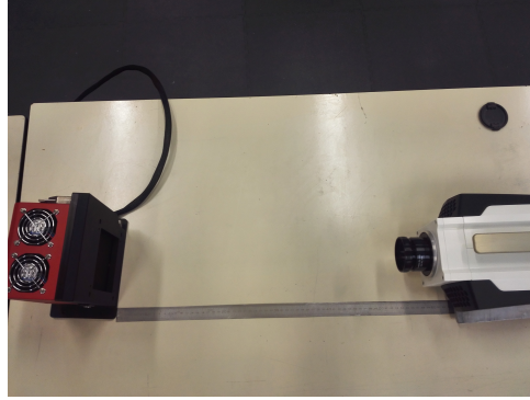
Figure 4.7: Experimental setup for the calibration of an IR camera.
