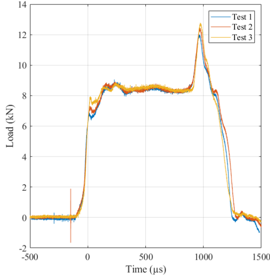
Figure 7.2: Loads evolution obtained for three different tests.
