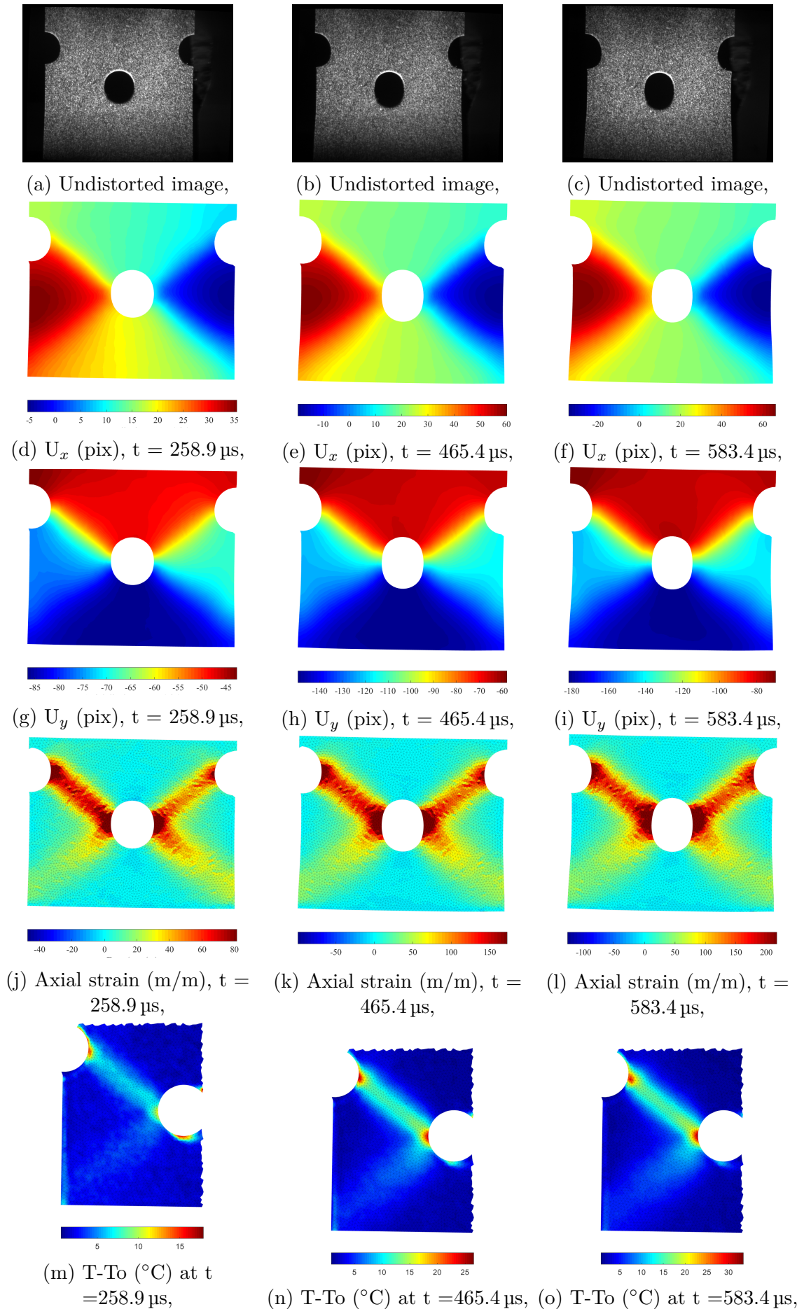
Figure D.1: Undistorted images, displacement fields and strain fields obtained during a dynamic tensile test, for different time steps. 221
