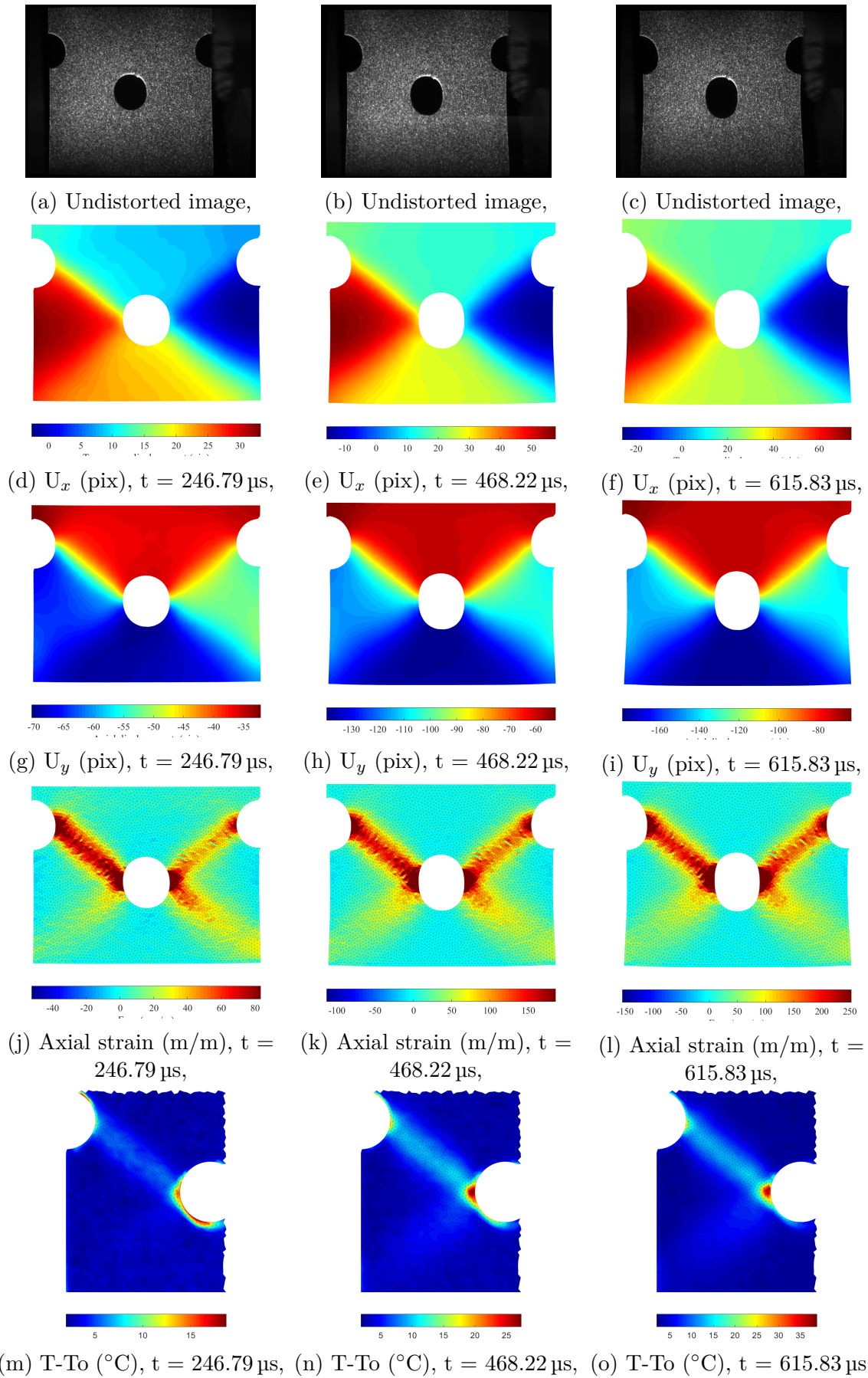
Figure 7.7: Undistorted images, displacement fields, strain fields as well as temperature fields obtained during a dynamic tensile test, for different time steps.
