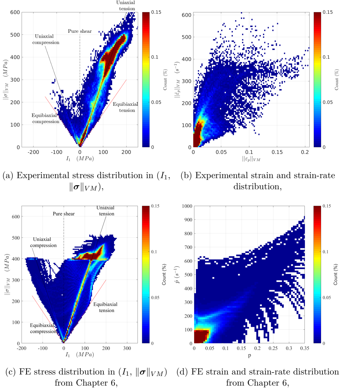
Figure 9.3: Comparison between the stress distribution, strain and strain-rate distributions during the experiment and the ones predicted in Chapter 6.
