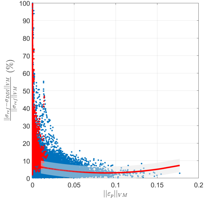
Figure 8.11: Relative error of the stress estimation for the selected mechanical states as a function of the Von-Mises norm of the plastic strains. The red line is the quadratic fit of the data presented for \|\varepsilon_p\|_{VM} \geq 0.01 and the grey area represents one standard deviation of the fit. The red points represent the mechanical states under compression ( I_1 \leq 0 ) and the blue points represent the states under tension ( I_1 \geq 0 ).
