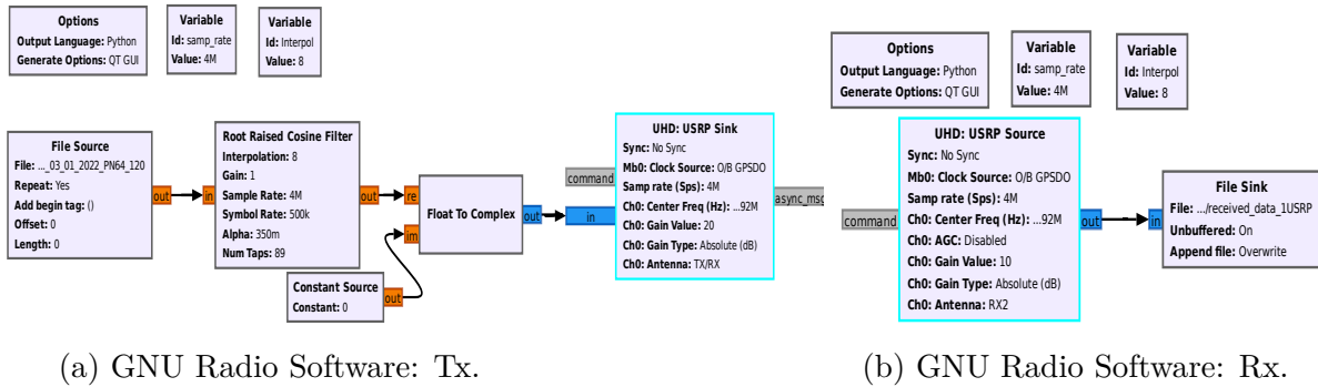
Figure 6.8 – Tx and Rx communication chain in GNU radio software.
