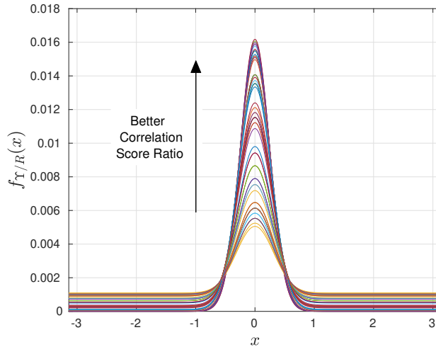
Figure 5.23 – f_{\xi/R} depending on the CCSK ratio R at SNR = -10 dB.
