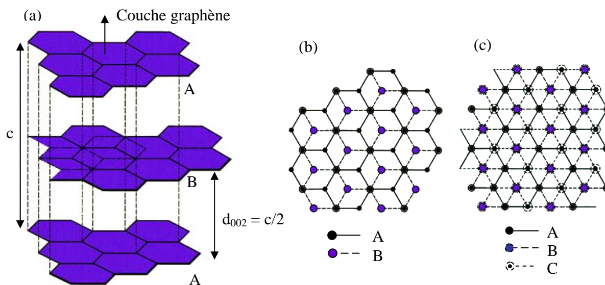
Figure I.5: Structures du graphite
