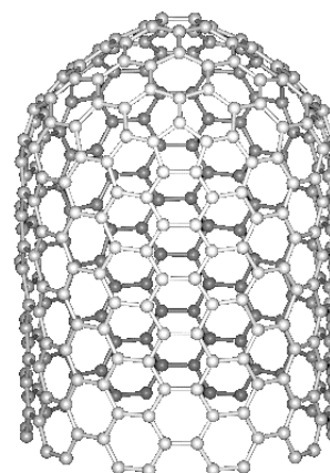
Figure I.4: Nanotube
