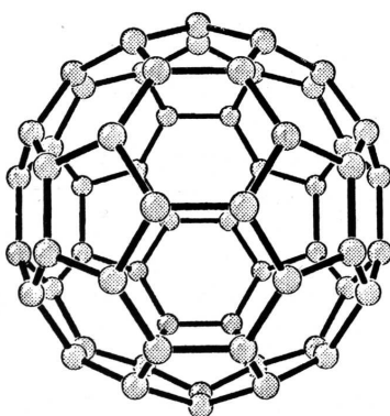
(a) Fullerène C_{60}
