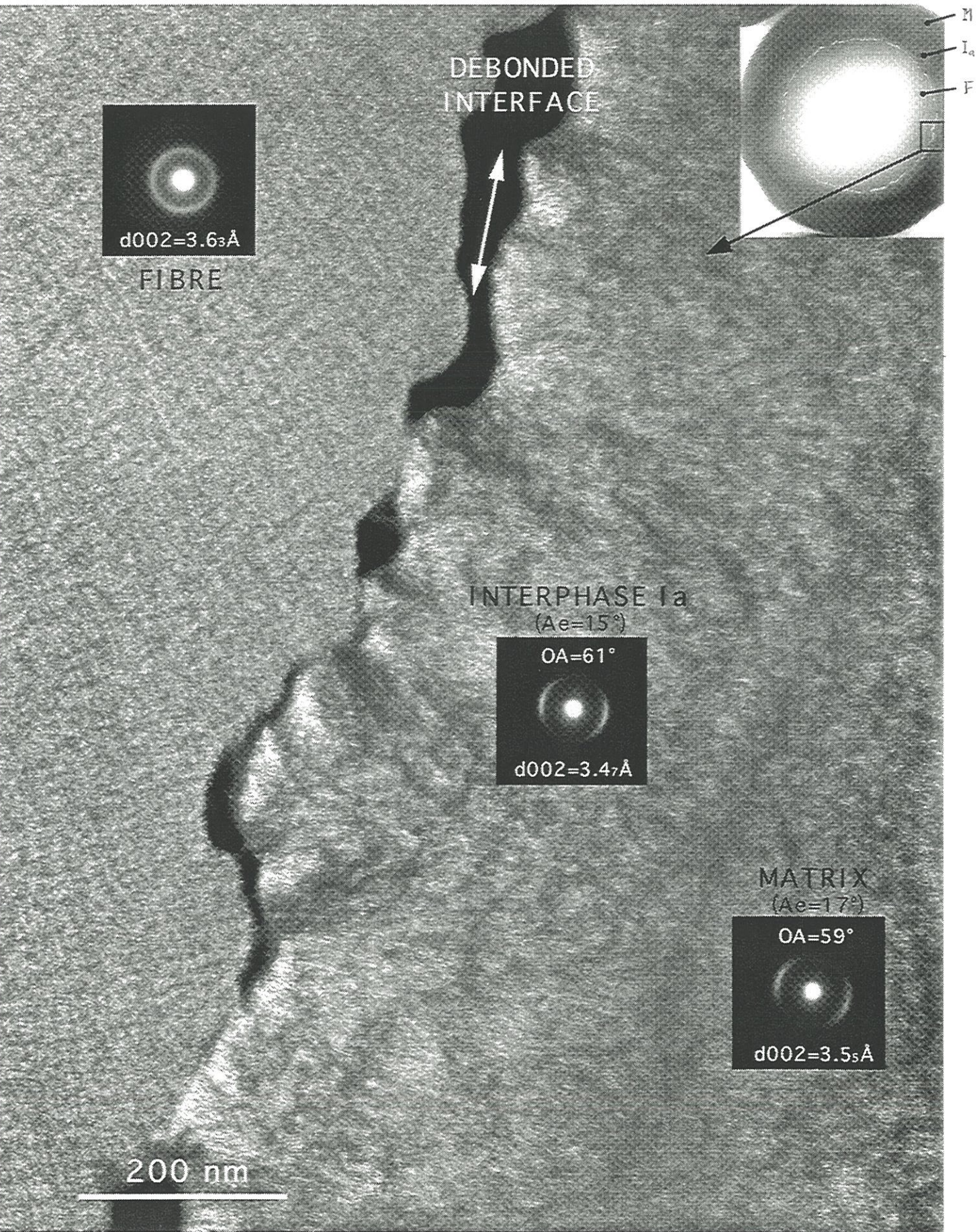
Figure 12: Microcomposite with interface Ia. Inset is a low magnification of the microcomposite
