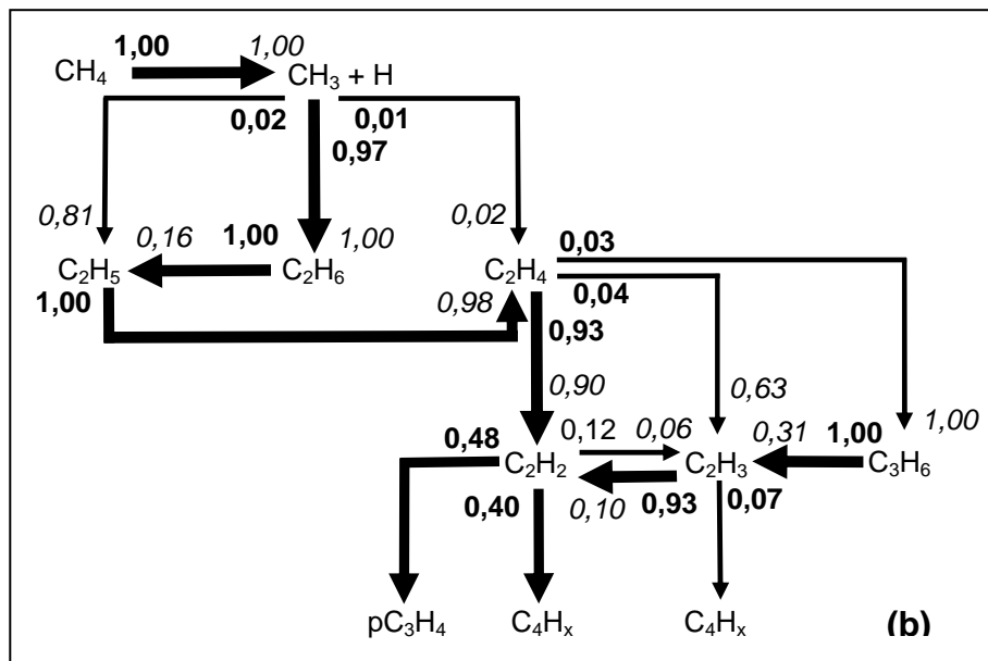
Figure 7: Reactions fluxes for: (a) propane ( T=1223\text{K} and P=2\text{kPa} ) and (b) methane ( T=1373\text{K} , P=10\text{kPa} and P_{\text{total}} = 100\text{kPa} )
