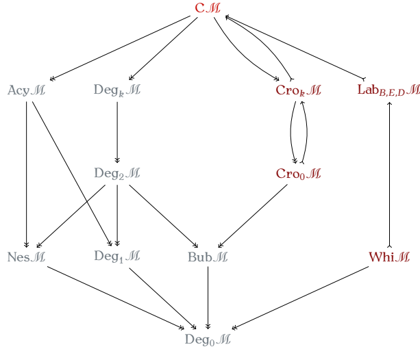
FIGURE 7.2. The diagram of the main suboperads and quotients of C\mathcal{M} . Arrows \hookrightarrow (resp. \twoheadrightarrow ) are injective (resp. surjective) operad morphisms. Here, \mathcal{M} is a unitary magma without nontrivial unit divisors, k is a positive integer, and B , E , and D are subsets of \mathcal{M} such that 1_{\mathcal{M}} \in B , 1_{\mathcal{M}} \in E , and E \star B \subseteq D .
