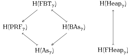
FIGURE 9.2. Diagram of combinatorial Hopf bialgebras where arrows \hookrightarrow (resp. \rightarrow ) are injective (resp. surjective) Hopf bialgebras morphisms. The parameter \gamma is a positive integer. When \gamma = 0 , H(\text{PRF}_0) = H(\text{As}_0) = H(\text{Heap}_0) = H(\text{FHeap}_0) and H(\text{FBT}_0) = H(\text{BAs}_0) .
