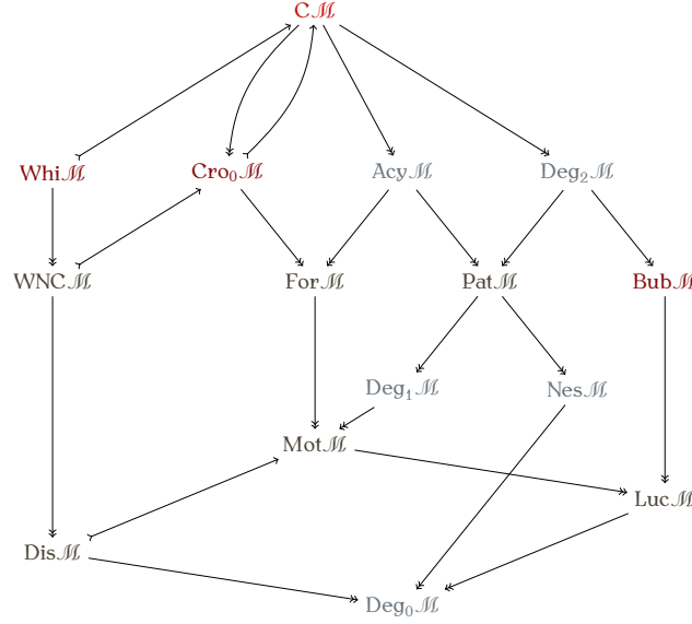
FIGURE 7.3. The diagram of the secondary suboperads and quotients of \mathcal{CM} together with some of their related main suboperads and quotients of \mathcal{CM} . Arrows \hookrightarrow (resp. \twoheadrightarrow ) are injective (resp. surjective) operad morphisms. Here, \mathcal{M} is a unitary magma without nontrivial unit divisors.
