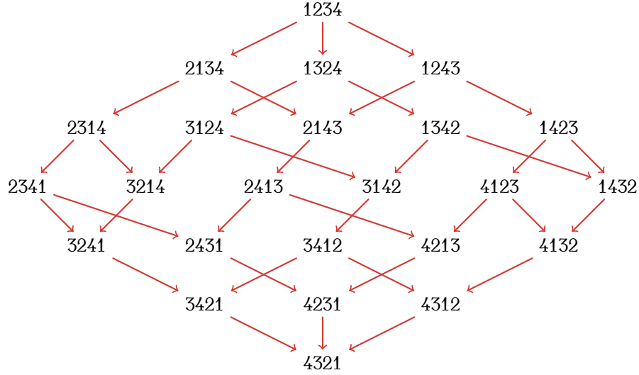
FIGURE 1.3. The Hasse diagram of the right weak poset of permutations of size 4.
