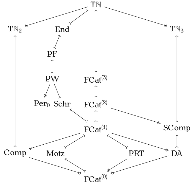
FIGURE 4.1. The diagram of ns suboperads and quotients of \text{TN} . Arrows \hookrightarrow (resp. \twoheadrightarrow ) are injective (resp. surjective) ns operad morphisms.
