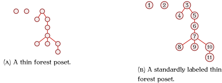
FIGURE 6.1. Hasse diagrams of a thin forest poset and a standardly labeled version.
