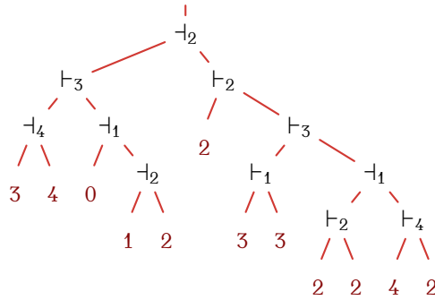
FIGURE 5.1. A \mathfrak{G}_{\text{Dias}_\gamma} -syntax tree t where the images of its leaves are shown. This tree satisfies \text{ev}(t) = 340122332242 .
