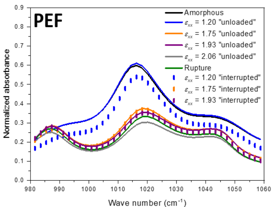
Annex 8: FT-IR spectra from 980 to 1060 \text{cm}^{-1} of amorphous, stretched up to the rupture, stretched and interrupted and stretched and unloaded PEF.
