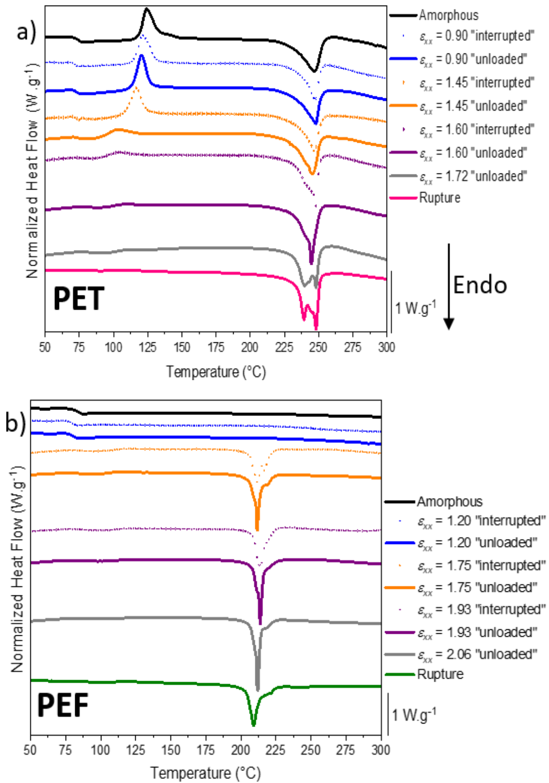
Figure 43. Thermal behaviour of (a) PET and (b) PEF, measured by DSC at a heating rate of 10^{\circ}\text{C}/\text{min} from 50^{\circ}\text{C} to 300^{\circ}\text{C} . Comparison is made between amorphous, “unloaded” samples (lines) and “interrupted” samples (dots). Endothermic phenomena are top-down [116].
