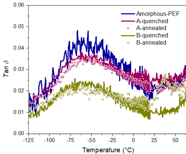
Annex 2. Viscoelastic measurement in the low temperature region of A and B tests (quenched and annealed), measured by DMTA at 1 Hz and 1 ^{\circ}\text{C}/\text{min} .
