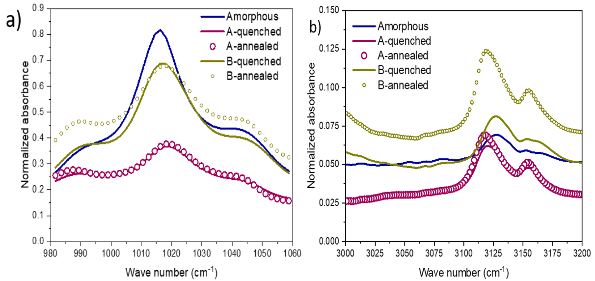
Annex 1. FT-IR measurement of amorphous, quenched (lines) and annealed (dots) PEF from (a) 980 \text{cm}^{-1} to 1060 \text{cm}^{-1} and (b) 3000 \text{cm}^{-1} to 3200 \text{cm}^{-1} .
