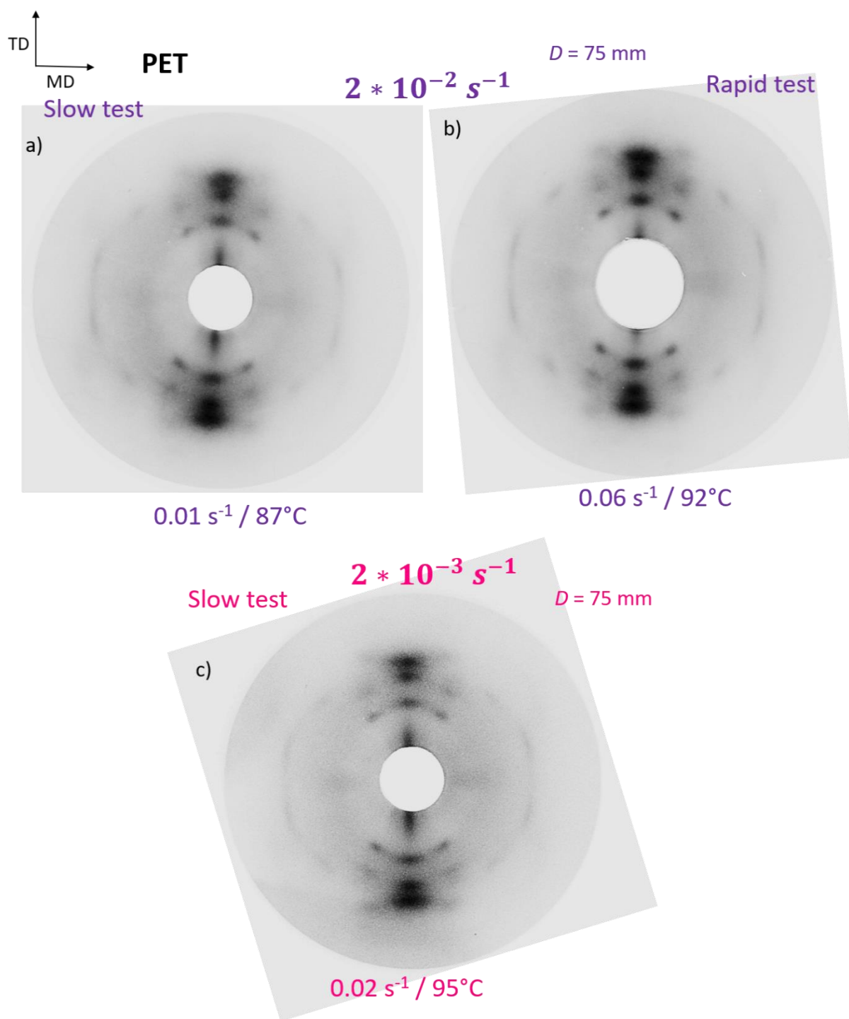
Annex 3. Debye-Scherrer patterns of stretched PET, (a) “slow” and (b) “rapid” strain rates at an equivalent strain rate of 2 * 10^{-2} \text{ s}^{-1} (purple); and (c) “slow” test of an equivalent strain rate of 2 * 10^{-3} \text{ s}^{-1} (pink) defined at the reference temperature of 90^{\circ}\text{C} .
