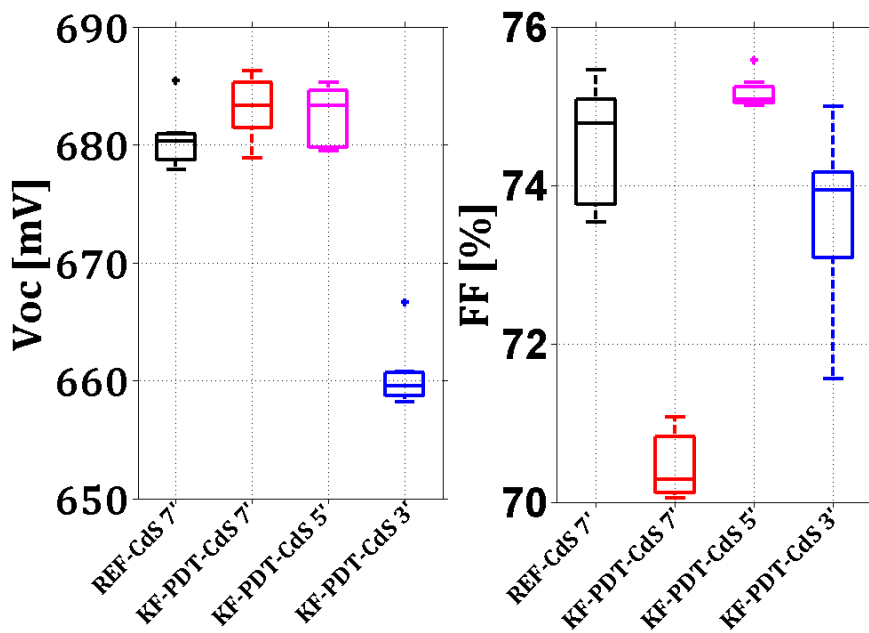
Figure 5-8 -- Voc (left) and FF (right) statistical results of solar cells with an absorber subjected to KF-PDT (red, magenta or blue) or not (black) and dipped into the CdS chemical bath for 3 (blue), 5 (magenta) and 7 minutes (red and black). Each box gives statistical results on 18 cells. The box has lines at the lower quartile, median and upper quartile values. Lines extending from each end of the box show the extent of the rest of the data
