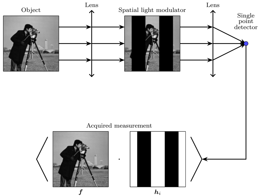
FIGURE 1.1 – The principle of the single-pixel camera. The measurements acquired are the inner product between the object to be acquired and the user-defined patterns on the spatial light modulator.
