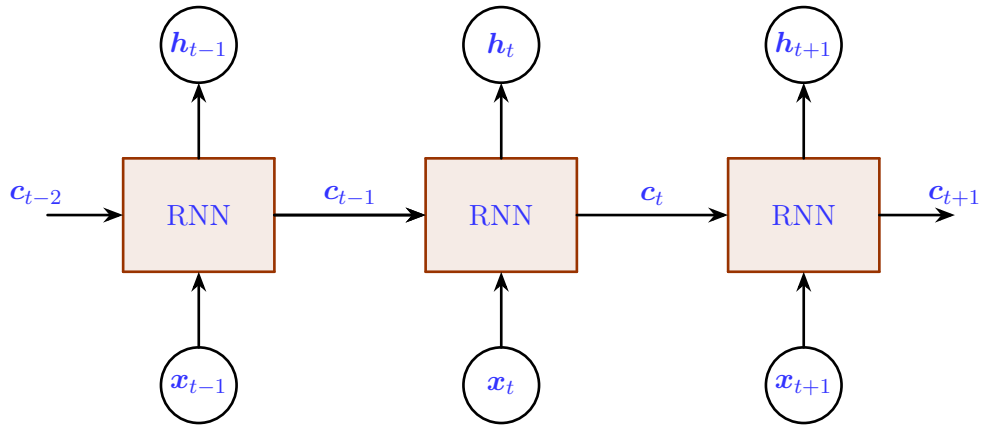
FIGURE 3.7 – Recurrent cell: The weights of the RNN are shared at all times. The recurrent cell takes as an input the cell state in the previous iteration \mathbf{c}_{t-1} , and the current inputs \mathbf{x}_t , and outputs a new cell state \mathbf{c}_t and the output \mathbf{h}_t .
