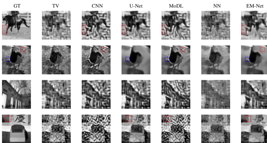
FIGURE 7.2 – Reconstructions of the simulated images using the different methods. Top row: STL-10 horse image with M = 512 and \alpha = 3 ph. Second row: STL-10 duck with M = 1,024 and \alpha = 30 ph. Third row: ImageNet hall with M = 512 and \alpha = 2 ph. Fourth row: ImageNet couch with M = 1,024 and \alpha = 5 ph. The images were reconstructed from simulated measurements from the ground-truth (GT) image. The following columns show reconstructions using total variation (TV), the ConvNet reconstructor presented in Fig. 7.1b (CNN), a U-Net reconstructor (Ronneberger et al., 2015) (U-net), a model-based reconstruction with deep learned priors (Aggarwal, Mani, and Jacob, 2019) (MoDL), and the proposed method (EM-Net).
