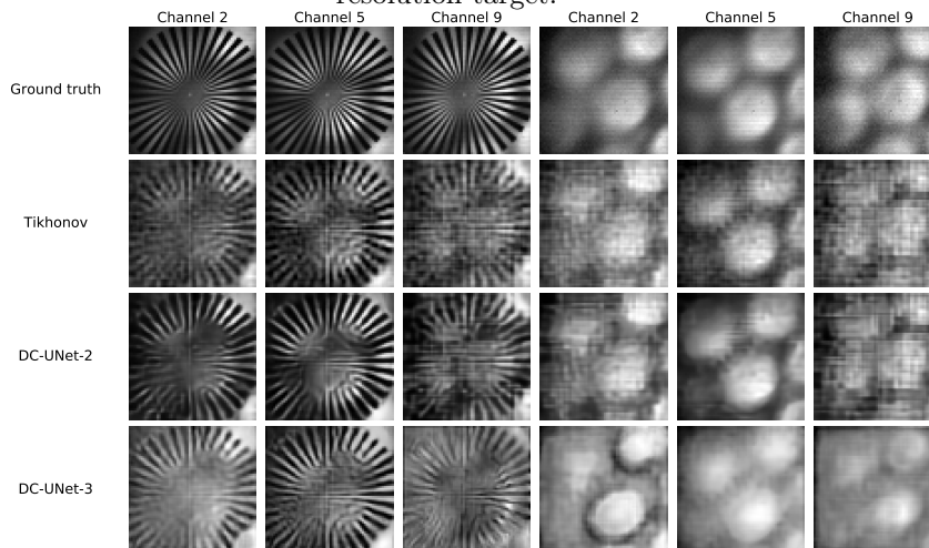
(b) Reconstruction of two experimental images - centered Siemens star target and LED lamp.
