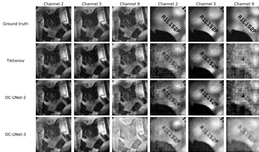
(a) Reconstruction of two experimental images - STL-10 cat and off-centered Siemens star resolution target.
