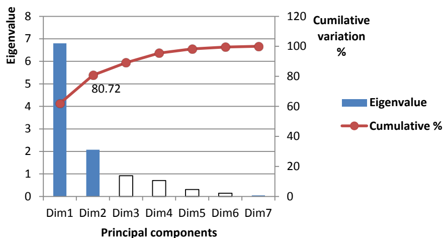
Figure 2. Scree plot.
