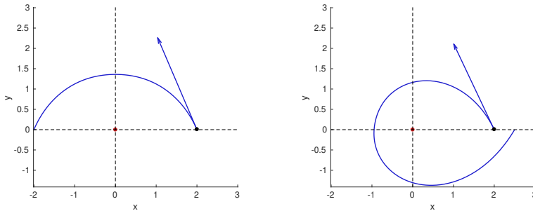
FIGURE 8.11 – Geodesic with a strong drift at the initial point : \mu = 2 \|q_0\| . (Left) q_0 = (2, 0) , q_f = (-2, 0) and the final time is t_f \approx 1.641 . (Right) q_0 = (2, 0) , q_f = (2.5, 0) and the final time is t_f \approx 2.821 .
