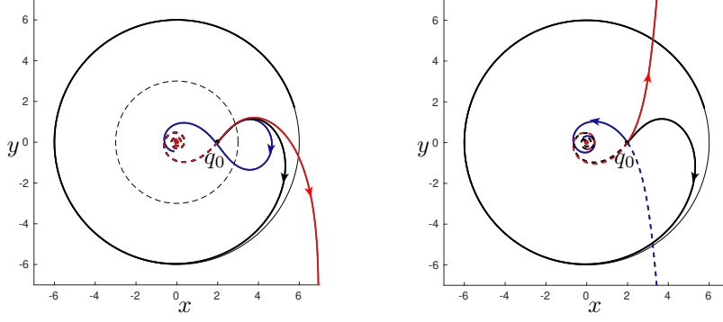
FIGURE 8.13 – (Left) Behavior of the trajectories around the separatrix (black). The geodesics below the separatrix (blue), i.e. parametrized by p_\theta < p_\theta^* ( p_\theta^* parametrizing the separatrix), converge towards the vortex and those above the separatrix (red) go to infinity. However, in the neighborhood of the separatrix the geodesics all come from the vortex. (Right) Illustration of the two pseudo-meridians represented in red and blue. The orbits of these do not coincide because of the drift. In dotted line the trajectories are traversed in negative time.
