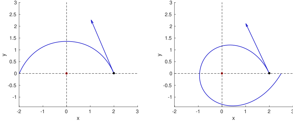
FIGURE 6.4 – Example 1 and 2. Geodesic with a strong drift at the initial point : \mu = 2 \|x_0\| . (Left : example 1) x_0 = (2, 0) , x_f = (-2, 0) and the final time is T \approx 1.641 . (Right : example 2) x_0 = (2, 0) , x_f = (2.5, 0) and the final time is T \approx 2.821 .
