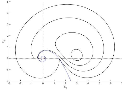
FIGURE 6.20 – Spheres \mathbb{S}(x_0, t) at times t \in \{0.5, 1.5, 2.5, 3.5\} in black together with the cut locus \Sigma_1 in blue. The cut locus should go to the vortex but to gain in clarity, it is represented up to a distance of 0.12 to the vortex. The vortex being represented by a red dot while the initial condition is represented by a black dot.
