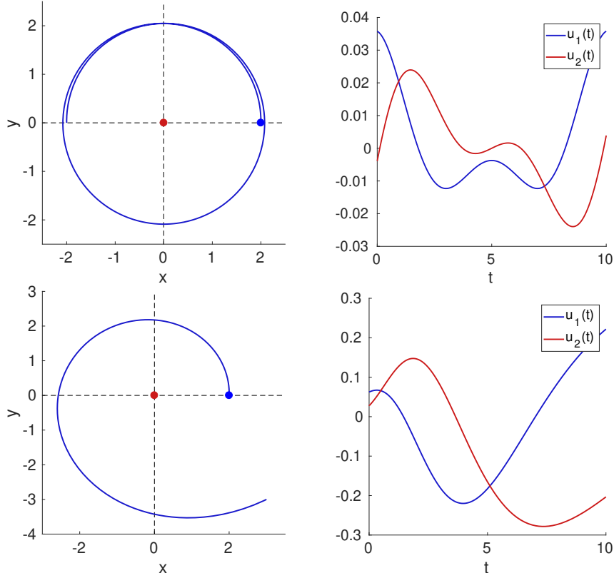
FIGURE 9.1 – One vortex. (Top) q_f = (-2, 0) and the cost is J \approx 4.2675e-3 . (Bottom) q_f = (3, -3) and the cost is J \approx 5.5177e-1 . In both cases, the shooting equation S = 0 is solved with a good accuracy of order 1e-12 . On the left, we have the trajectory (in blue), the point vortex is represented by a red dot, the initial condition by a blue dot. The two control components are given on the right.
