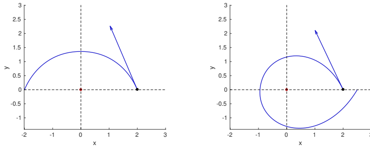
FIGURE 8.11 – Geodesic with a strong drift at the initial point : \mu = 2 \|q_0\| . (Left) q_0 = (2, 0) , q_f = (-2, 0) and the final time is t_f \approx 1.641 . (Right) q_0 = (2, 0) , q_f = (2.5, 0) and the final time is t_f \approx 2.821 .
