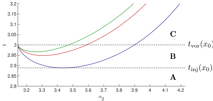
FIGURE 6.16 – Graph of the function t(\alpha_2) along \Sigma_1 (blue), \Sigma_2 (red) and \Sigma_3 (green) for times t \leq 3.2 . The balls are of three types : A, B and C. See the description detailed in the step 3.
