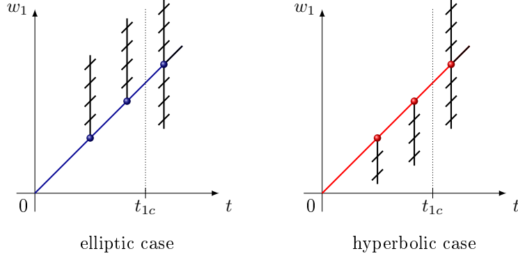
FIGURE 8.1 – Projection of the fixed time accessibility set on the w_1 -coordinate; t_{1c} being the first conjugate time.
