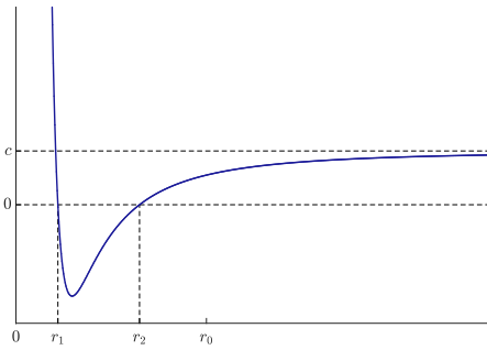
FIGURE 6.9 – Case \Delta > 0 and p_\theta > 0 . Graph of r \mapsto P(1/r^2) . Setting : \mu = 2 , r_0 = 3\mu , p_\theta = r_0/2 .
