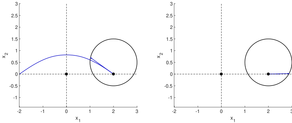
FIGURE 6.5 – Example 3 and 4. Geodesic with a weak drift at the initial point : \mu = 0.5 \|x_0\| . (Left : example 3) x_0 = (2, 0) , x_f = (-2, 0) and the final time is T \approx 2.826 . (Right : example 4) x_0 = (2, 0) , x_f = (2.5, 0) and the final time is T \approx 0.56 . Compare this to Figure 6.4.
