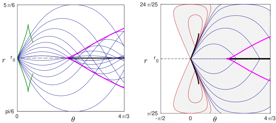
FIGURE 8.8 – (Left) Hyperbolic flow, conjugate and cut loci. (Right) Optimal synthesis in minimal time in an adapted neighborhood R = \{\pi/25 \leq r \leq 24\pi/25; -\pi/2 \leq \theta \leq 4\pi/3\} . The pseudo-meridians (separatrices) are portrayed in black while the hyperbolic geodesics to the left and right of the separatrices are in red and blue. The abnormal geodesics are in green. Conjugate and cut loci are in magenta and black. The gray sector represents, in the considered adapted neighborhood, the reachable domain. The white domain is not reachable in the neighborhood. We take \lambda = 4/5 and v = 0.9 .
