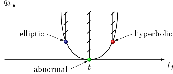
FIGURE 7.2 – Projection of the accessibility sets on the q_3 -coordinate in the abnormal case.
