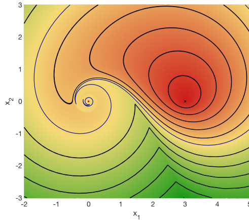
FIGURE 6.21 – Optimal synthesis. The black curves represent the spheres of types A and C. The two blue curves is a single sphere of type B. Since the balls of type B are not simply connected and have one hole, the corresponding spheres have two connected components.
