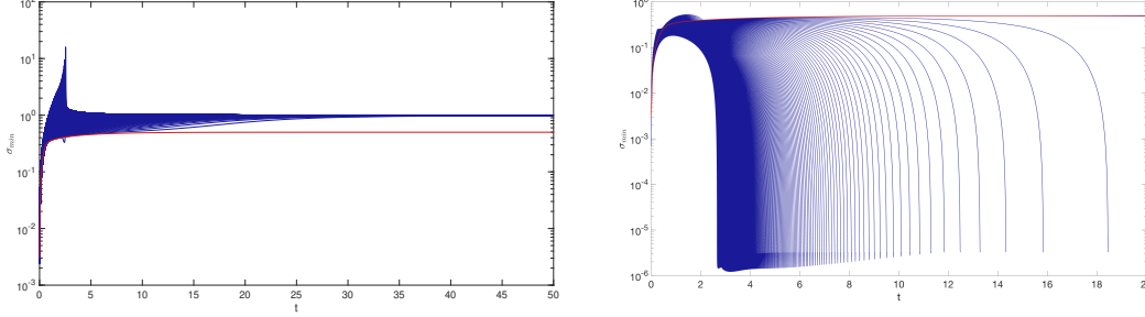
FIGURE 6.6 – Smallest singular value with respect to time. Setting : \theta_0 = 0 , \mu = 2.0 , r_0 = 4\mu/3 (weak drift at the initial point). The set of parameters [0, 2\pi[ is uniformly discretized in N := 1000 sub-intervals and we define 0 =: \alpha_1 < \dots < \alpha_N < 2\pi the associated parameters. Each blue curve is the graph of the smallest singular value \sigma_{\min}(t) for one \alpha \in \Theta(r_0, \mu) \cap \cup_{i=1}^N \{\alpha_i\} and for t \in [0, 50] on the left subgraph, and for one \alpha \in \Lambda(r_0, \mu) \cap \cup_{i=1}^N \{\alpha_i\} on the right subgraph. In this case, we stop the numerical integration when r(t) \leq 10^{-3} which explains why the minimal value of \sigma_{\min} is between 10^{-5} and 10^{-6} . The red curve on each plot corresponds to the separatrix.
