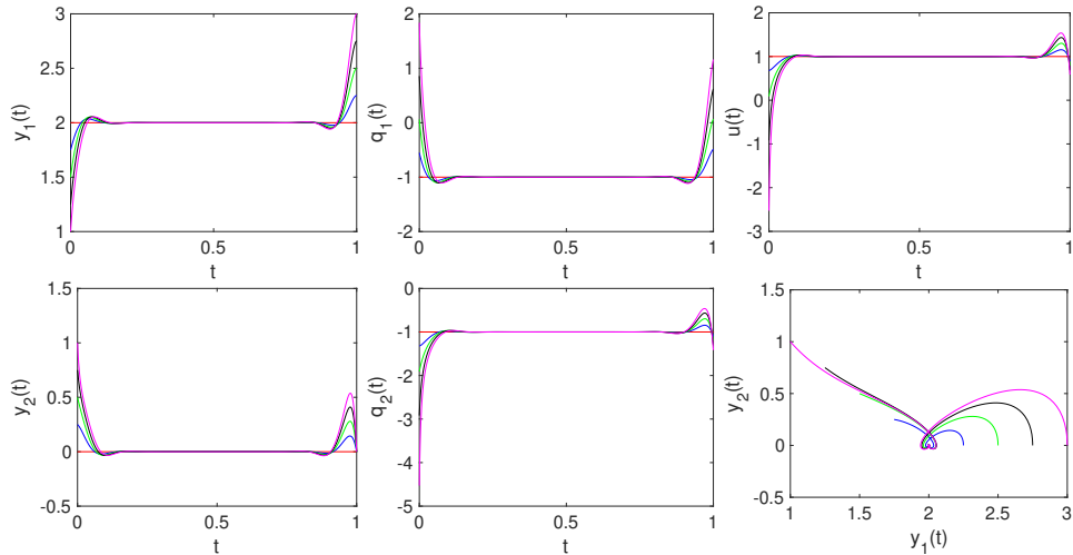
FIGURE 10.1 – Second step (homotopy on \lambda ). Graphs of state, co-state and optimal control during the first homotopy, with T = 40 , for \lambda \in \{0, 0.25, 0.5, 0.75, 1\} .
