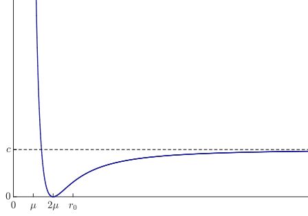
FIGURE 6.8 – Case \Delta = 0 . Graph of r \mapsto P(1/r^2) . Setting : \mu = 2 , r_0 = 3\mu , p_\theta = p_\theta^* .
