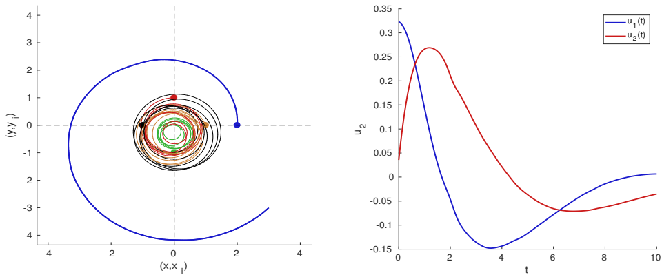
FIGURE 9.4 – Four vortices. Trajectory and control in the four vortices case. The initial adjoint vector is p_0 = (0.17, -0.0015, 0.041, -0.18, -0.025, -0.26, 0.11, 0.11, -0.18, 0.22) (see Table 9.1 for details).
