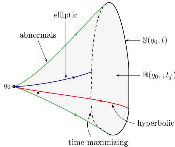
FIGURE 7.4 – Small sphere (plain black line) and ball (delimited by the abnormal geodesics and the sphere) for the strong current case. Note that the elliptic geodesics do not play a role in the construction of the time minimal sphere. But the part of the wavefront formed by the elliptic geodesics is represented (dashed line), together with an elliptic geodesic, to emphasize the difference with the weak case and represent the accessibility set in time t_f which is the interior of the wavefront.
