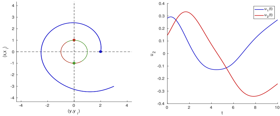
FIGURE 9.2 – Two vortices. Trajectory and control in the two vortices case. The initial adjoint vector being p_0 = (0.28, 0.15, 0.097, -0.47, -0.11, 0.088) (see Table 9.1 for details).
