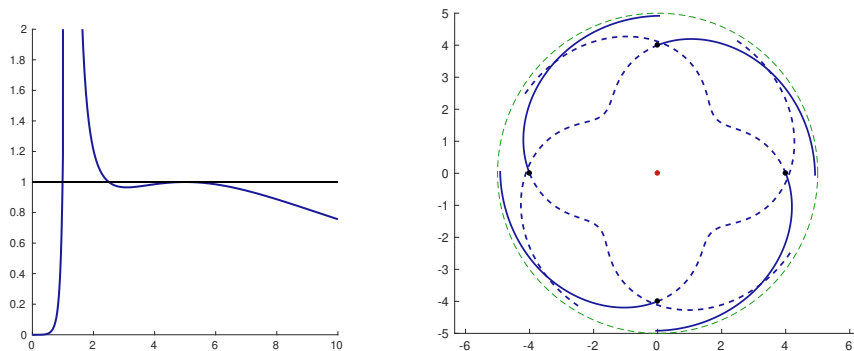
FIGURE 8.20 – Case 2-(c). Homocline separatrix parameterized by p_\theta^3 . The green circle represents the equator associated to r_3 .
