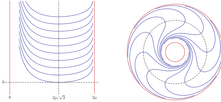
FIGURE 6.12 – (Left) Graphs of r \in ]0, 2\mu[ \mapsto -\ln(f(r)) + c , c \in \mathbb{R} , with f defined by eq. (6.25). The minimum is attained at r = 2\mu/\sqrt{3} where f'(r) = 0 . (Right) Generalized 2-dimensional compact Reeb component of the annulus given by the function F(r, \theta) = f(r) e^\theta . The intermediate dashed circle of radius 2\mu/\sqrt{3} is orthogonal to all the non compact leaves in blue. The two compact leaves are the two red circles.
