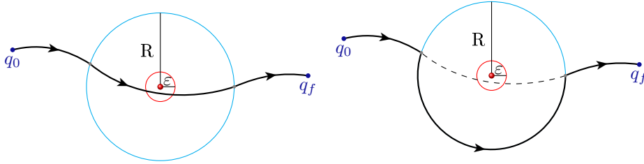
FIGURE 8.10 – Illustration of the construction of a strictly better admissible trajectory. The vortex is represented by a red ball, while the trajectories are the solid black lines. One can see on the left, a trajectory crossing the ball of radius \varepsilon . This trajectory is replaced on the right sub-graph by a strictly better admissible trajectory.
