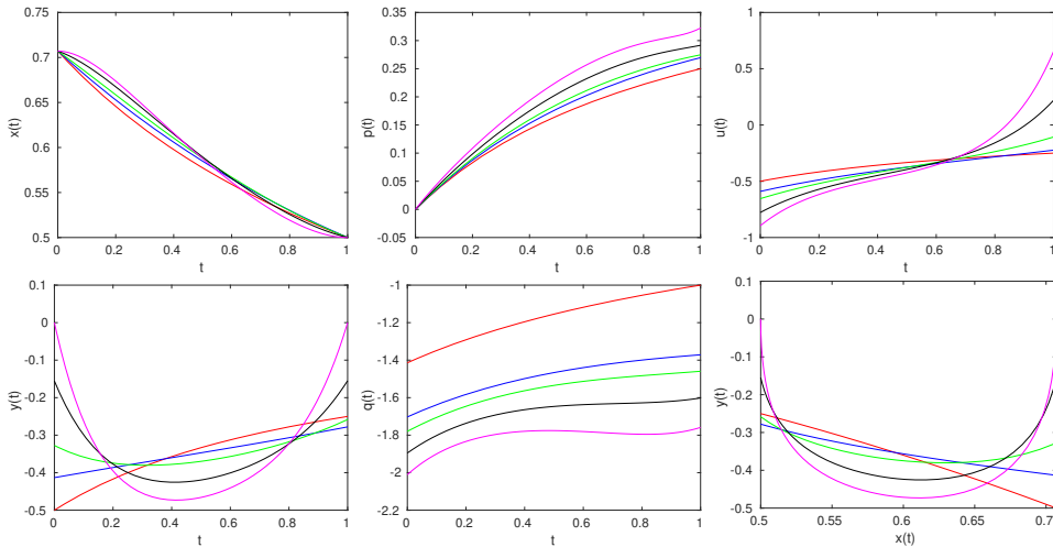
FIGURE 10.3 – Second step (homotopy on \lambda ). Graphs of state, co-state and optimal control for \lambda \in \{0.0, 0.3, 0.5, 0.8, 1.0\} , with \varepsilon = 0.25 .
