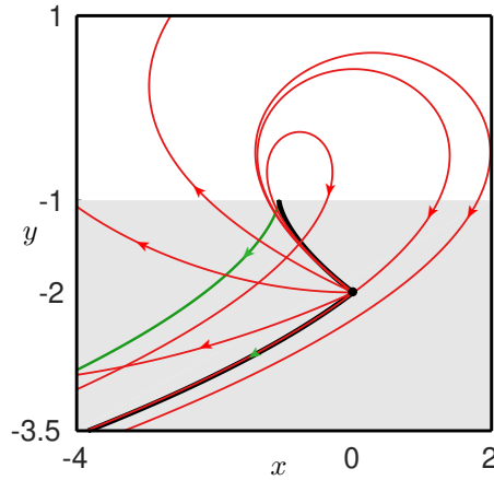
FIGURE 8.6 – Minimal time optimal synthesis in an adapted rectangle neighborhood containing the limit loop. The initial point is q_0 = (0, -2) . The abnormal geodesics are represented in green and in red are represented hyperbolic geodesics. The cut locus, formed by the abnormal geodesics, is represented in black.
