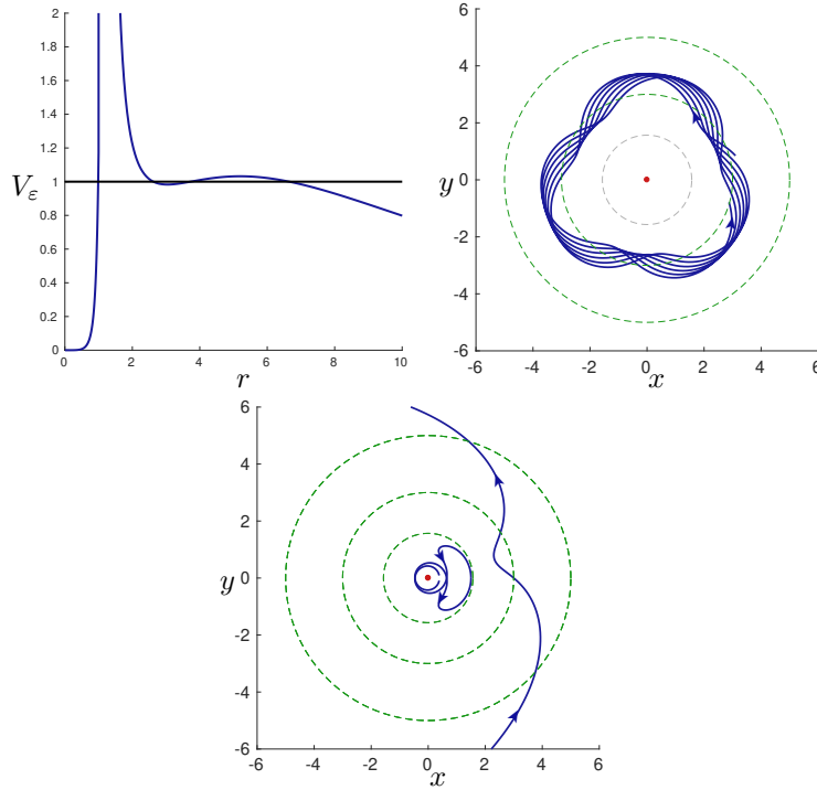
FIGURE 8.17 – Case 2-(b). We deduce from the potentials (left) that trajectories starting between the minimum and the maximum remain contained in an annulus, that those coming from the vortex return to it and that those starting from a large r_0 go to infinity. On the middle graph we represent a compact trajectory and in the right graph we represent the two other situations. On the right-hand graph is represented a trajectory for which the associated potential has its local maximum strictly less than 1 : we can see it oscillating around the r_2 L-elliptic equator.
