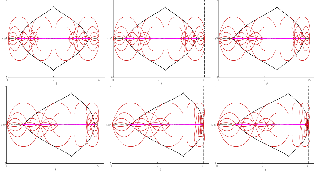
FIGURE 8.9 – Illustration of the deformation of the geodesic flow and conjugate locus in the weak current case. Taking \lambda = 4/5 and v = 0.0, 0.1, 0.2, 0.3, 0.4, 0.42 respectively from above left to below right. Hyperbolic geodesics are represented in red, conjugate and cut loci are respectively represented in black and orange.
