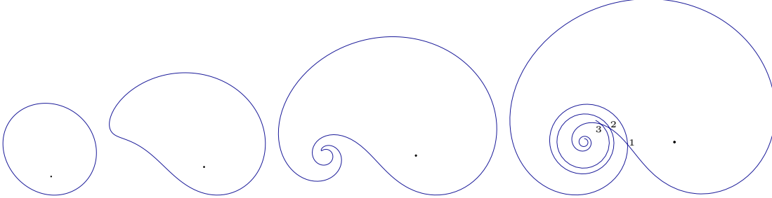
FIGURE 6.15 – Four wavefronts with different scaling at times t \in \{0.5, 2, 2.8, 3.5\} . The black dot is x_0 . For t = 3.5 , the wavefront has at least three self-intersections labelled 1, 2 and 3.
