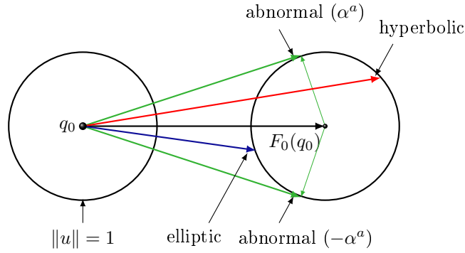
FIGURE 7.3 – Strong current case : ball of directions.
