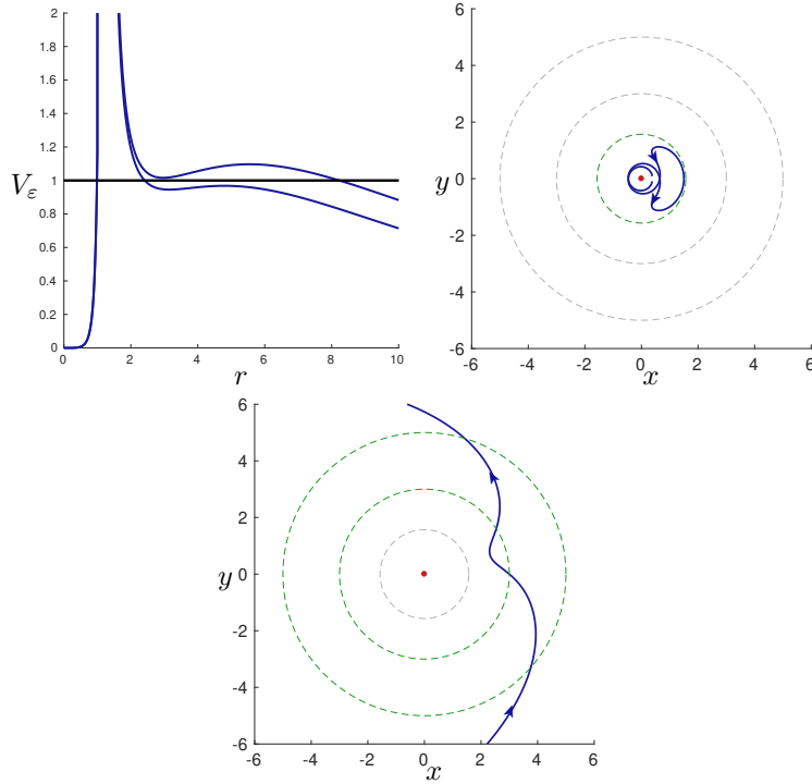
FIGURE 8.16 – Case 2-(a). We deduce from the potential (left) that the trajectories coming from the vortex return to it and that those starting from a quite large r_0 go to infinity.
