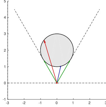
FIGURE 6.3 – The vortex is placed at the origin and marked by a black dot, as the initial point x_0 := (2, 0) in cartesian coordinates. The drift is strong at the initial point since \mu = 2r_0 . The black circle represents the set of initial directions x_0 + \mathcal{F}(x_0, \mu) and the blue vector is the initial hyperbolic direction associated to the initial control u(0) := (\cos \alpha, \sin \alpha) , with \alpha = 7\pi/8 . The direction in green is elliptic while the two red directions are the abnormal directions located at the boundary of the cone of admissible directions.
