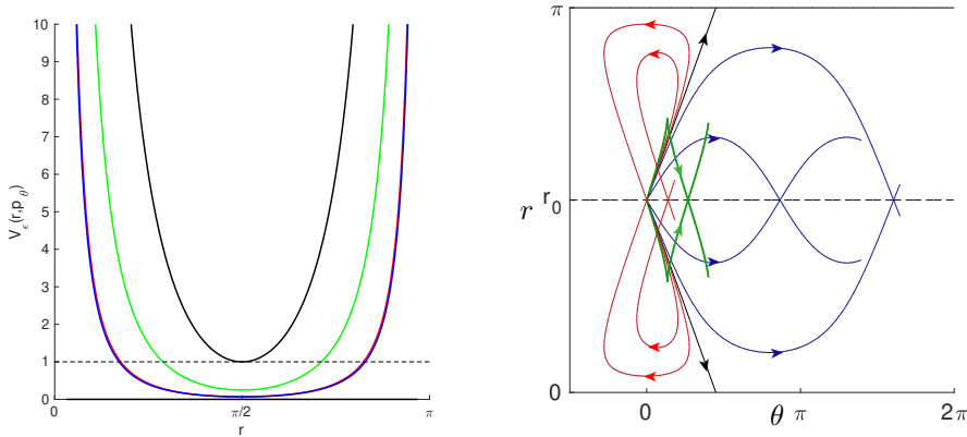
FIGURE 8.7 – (Left) We represent the potential for the different classes of geodesics in order to highlight the periodicity of the solutions. (Right) Illustration of different types of hyperbolic geodesics in the strong drift case. The meridians and the equator are represented in black while hyperbolic geodesics with a loop (resp. without loop) are represented in red (resp. in blue). Abnormal geodesics are represented in green. In this representation, we take \lambda = 4/5 and v = 0.9 .
