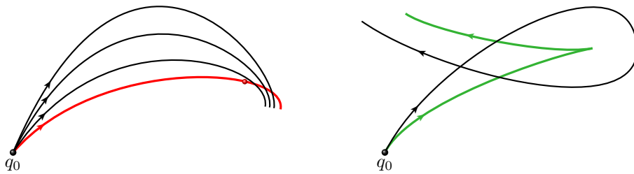
FIGURE 8.4 – Conjugate points in the 2D-space in normal (left) and abnormal (right) cases.
