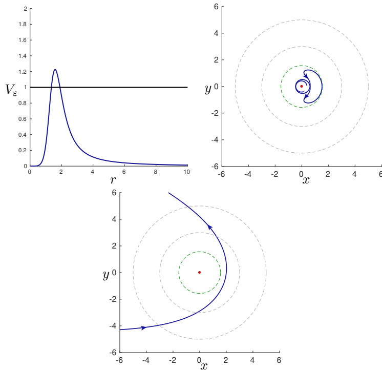
FIGURE 8.15 – Case 1-(b). We deduce from the potential (left) that the trajectories coming from the vortex go back to the vortex, and that the ones starting from a quite large r_0 go to infinity.
