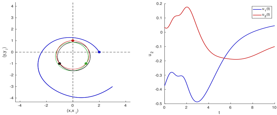
FIGURE 9.3 – Three vortices. Trajectory and control in the three vortices case. The initial adjoint vector being p_0 = (-0.37, -0.037, 0.088, 0.34, 0.69, -0.48, -0.36, -0.026) (see Table 9.1 for details).
