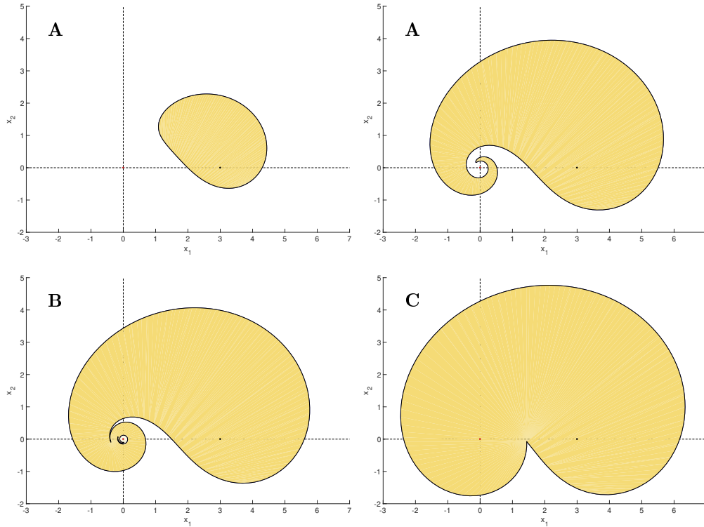
FIGURE 6.18 – Four balls in the (x_1, x_2) -plane at times t \in \{1.5, 2.8, 2.9, 3.5\} with the initial condition x_0 represented by a black dot and the vortex by a red dot. The balls \mathbb{B}(x_0, 1.5) and \mathbb{B}(x_0, 2.8) on top are of type A. The ball \mathbb{B}(x_0, 2.9) (Bottom-Left) is of type B while \mathbb{B}(x_0, 3.5) (Bottom-Right) is of type C.
