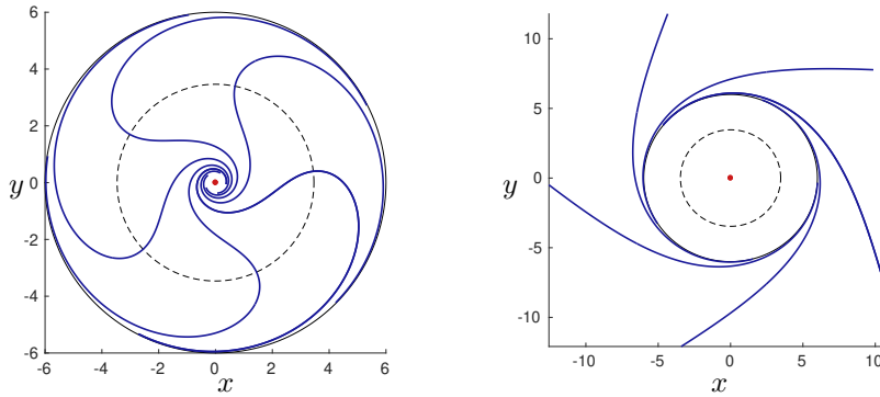
FIGURE 8.12 – (Left) Reeb's foliation formed by the separatrices in the perforated disk of radius 2k in the (x, y) plane. (Right) Foliation formed by the separatrices outside the disk of radius 2k . The vortex is placed at the origin and represented by a red point. The circles in black correspond to circles of radius 2k/\sqrt{3} (where \dot{\theta} vanishing along the separatrix) and of radius 2k .
