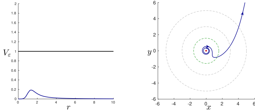
FIGURE 8.14 – Case 1-(a). We can deduce from the potential represented on the left graph that trajectories necessarily come from the vortex and go to infinity, the orientation of trajectories being taken according to the positive direction of integration that we have chosen.
