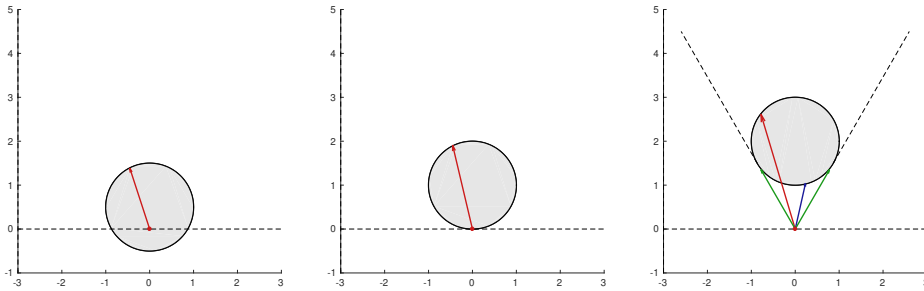
FIGURE 6.2 – The vortex is placed at the origin and marked by a black dot, as the initial point x_0 := (2, 0) in cartesian coordinates. The black circle corresponds to the set of initial directions x_0 + \mathcal{F}(x_0, \mu) and the thick blue vector is the initial direction associated to the initial control u(0) := (\cos \alpha, \sin \alpha) , with \alpha = 7\pi/8 . It is decomposed as the sum of the drift (oriented vertically) and the control field. On the left, we have a weak drift ( \mu = 0.5 r_0 ), in the middle we have a moderate drift ( \mu = r_0 ) and on the right a strong drift ( \mu = 2 r_0 ).
