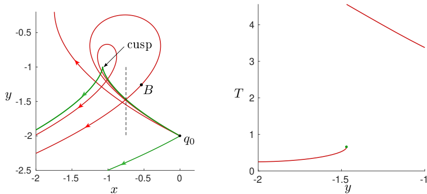
FIGURE 8.3 – (Left) The initial point is q_0 = (0, -2) . The abnormal geodesic with the cusp singularity is in green while the others geodesics in red are hyperbolic. We can see that the cusp singularity is the limit of self-intersecting hyperbolic geodesics. Besides, to reach the point B from q_0 , one has to use a hyperbolic self-intersecting geodesic. When this hyperbolic geodesic intersects the abnormal, the time is longer along the hyperbolic than the abnormal. At this intersection, the hyperbolic geodesic ceases to be optimal. (Right) The time minimal value function along the dashed segment geodesic from the left sub-graph. The discontinuity occurs at the intersection between the hyperbolic and abnormal geodesics. It is represented by the green dot, which is the time along the abnormal geodesic.
