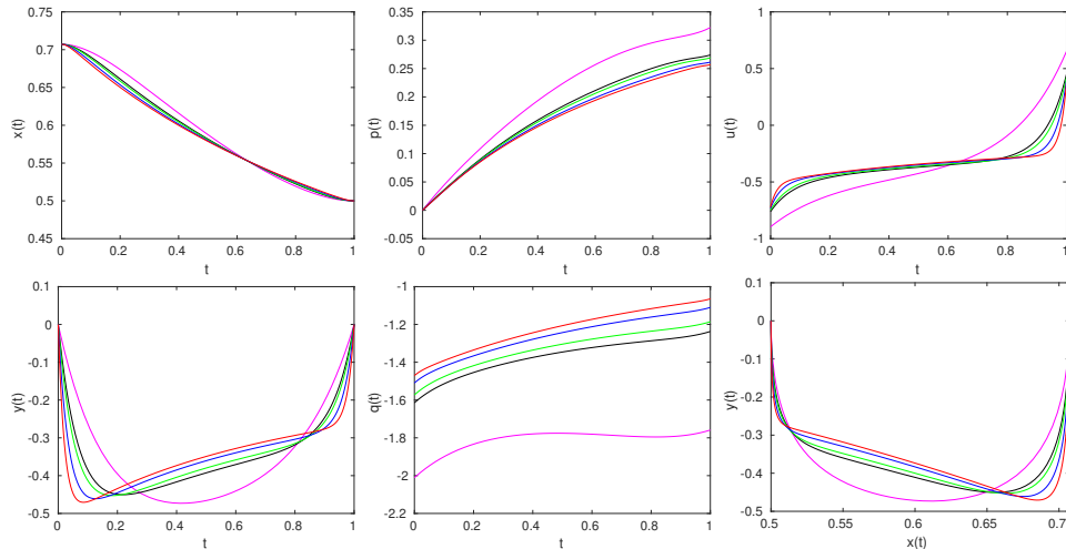
FIGURE 10.4 – Third step (homotopy on \varepsilon ). Graphs of state, co-state and optimal control for \varepsilon \in \{0.025, 0.05, 0.08, 0.1, 0.25\} , with \lambda = 1 .
