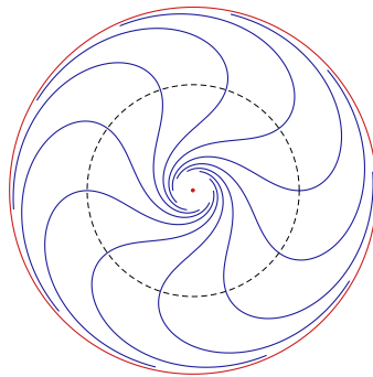
FIGURE 6.13 – Separating geodesics in the punctured disk of radius 2\mu in the (x_1, x_2) -plane. The vortex is placed at the origin and represented by a red dot. The red circle is the Reeb circle of radius 2\mu while the black and dashed circle is the circle of radius 2\mu/\sqrt{3} where \dot{\theta} = 0 along the separating geodesics.
