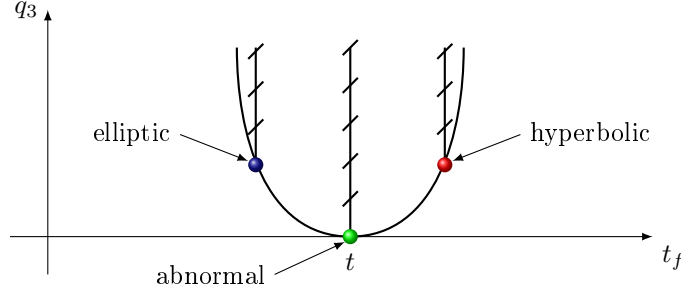
FIGURE 8.2 – Projection of the accessibility sets on the q_3 -coordinate in the abnormal case.
