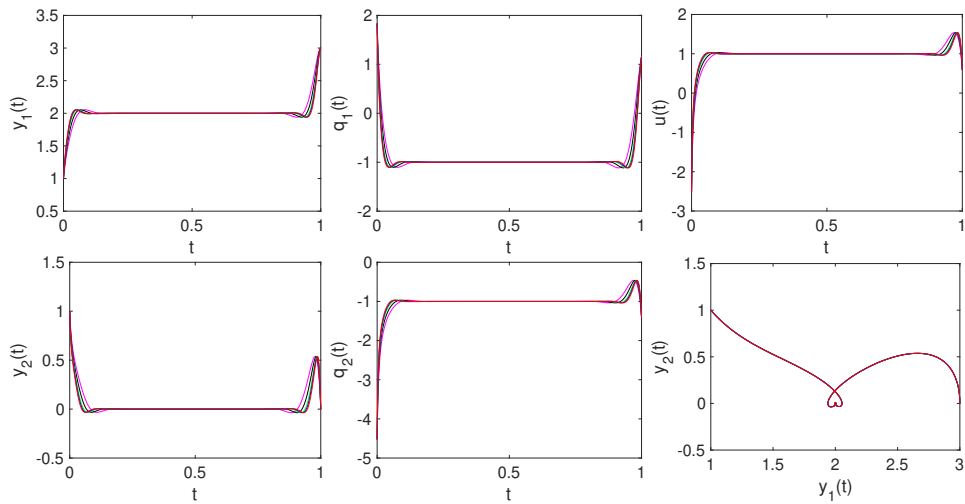
FIGURE 10.2 – Third step (homotopy on \varepsilon ). Graphs of state, co-state and optimal control during the homotopy on \varepsilon = 1/T , for T \in \{40, 50, 60, 65, 70\} .
