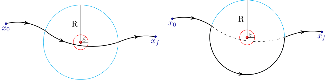
FIGURE 6.1 – Illustration of the construction of a strictly better admissible trajectory. The vortex is represented by a red ball, while the trajectories are the solid black lines. One can see on the left, a trajectory crossing the ball of radius \varepsilon . This trajectory is replaced on the right subgraph by a strictly better admissible trajectory.
