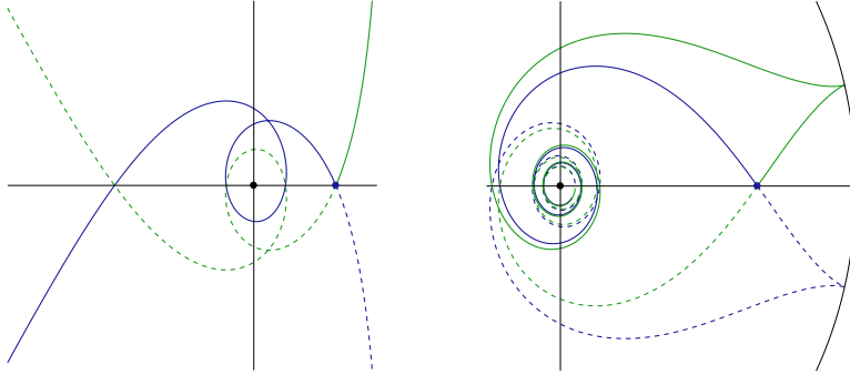
FIGURE 6.14 – Geodesics in the state space in the (x_1, x_2) -plane. The vortex is placed at the origin and represented by a black dot. The initial point, denoted x_0 , is the black dot at an intersection of both geodesics. The geodesic in green is obtained by a reflection of axis \mathbb{R}x_0 from the blue geodesic and vice-versa. Assuming that the initial point is given at time t = 0 , then the plain lines are obtained for times t > 0 while the dashed parts are for negative times. On the left subgraph is represented a normal geodesic with both extremities going to infinity while on the right subgraph is represented the two abnormal (in the case of a strong drift) with a cusp at r = |\mu| . Both extremities of the abnormal geodesics go the vortex.
