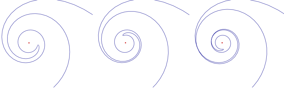
FIGURE 6.17 – Three wavefronts with the same scaling and a zoom around the vortex (red dot) for t \in \{2.86, 2.88, 2.9\} . For t = 2.9 > t_{\text{inj}}(x_0) \approx 2.889 , the wavefront has two self-intersections.
