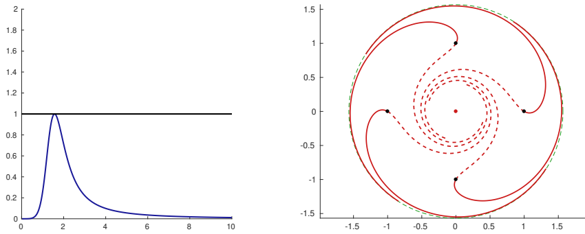
FIGURE 8.18 – Case 1-(c). Reeb's foliation formed by the separatrix parameterized by p_\theta^1 . In continuous line the trajectories are crossed in positive time and in dashed line they are crossed in negative time. The vortex is represented by the red dot and the different initial points by the black dots. The green circle represents the equator associated to r_1 .
