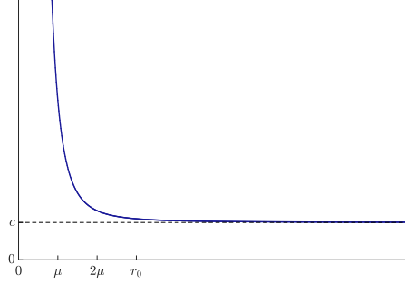
FIGURE 6.7 – Case \Delta < 0 . Graph of r \mapsto P(1/r^2) . Setting : \mu = 2 , r_0 = 3\mu , p_\theta = p_\theta^*/2 \in ]p_\theta^*, 0[ .
