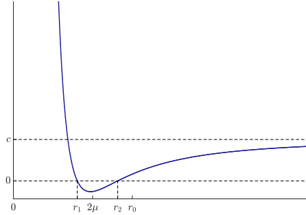
FIGURE 6.10 – Case \Delta > 0 and p_\theta < p_\theta^* : r \mapsto P(1/r^2) . Setting : \mu = 2 , r_0 = 3\mu , p_\theta = (p_\theta^* - r_0)/2 .
