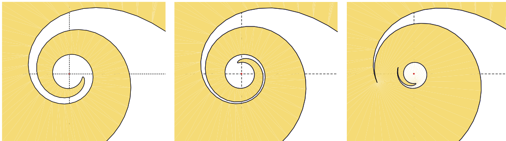
FIGURE 6.19 – Three balls with a zoom around the vortex (red dot) at times t \in \{2.86, 2.88, 2.9\} . Compare to Figure 6.17. For t = 2.9 the ball \mathbb{B}(x_0, t) is of type C and has a small hole with a fetus shape.
