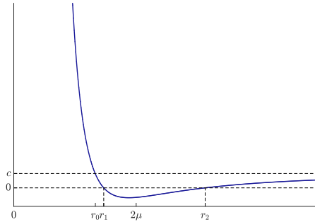
FIGURE 6.11 – Case \Delta > 0 and p_\theta < p_\theta^* : r \mapsto P(1/r^2) . Setting : \mu = 2 , r_0 = 4\mu/3 , p_\theta = (p_\theta^* - r_0)/2 .
