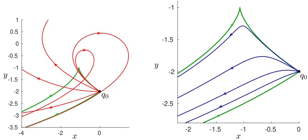
FIGURE 8.5 – Geodesic flow in hyperbolic case (Left) and elliptic case (Right) in the whole conic neighborhood delimited by the two abnormal geodesics. Hyperbolic geodesics are represented in red, elliptic geodesics are represented in blue and abnormal geodesics are represented in green. Initial point is taken at q_0 = (0, -2) .
