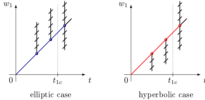
FIGURE 7.1 – Projection of the fixed time accessibility set on the w_1 -coordinate.
