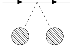
FIGURE 5.2: Feynman diagram corresponding to the insertion of a disformal vertex with any other arbitrary vertices
