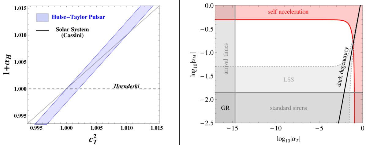
Figure 41: Left : Figure in 2 [232]. Hulse-Taylor Pulsar and Cassini constraints on \alpha_H and c_T^2 are shown. Right : Figure 4 in [261]. The prospective constraints on \alpha_M and \alpha_T with gravitational wave detectors measuring the decay of the wave amplitude with standard sirens and the arrival time with respect to the electromagnetic emission from a cosmological event. The shaded regions correspond to the allowed regions and the red region corresponds to where self-accelerating models lie.
