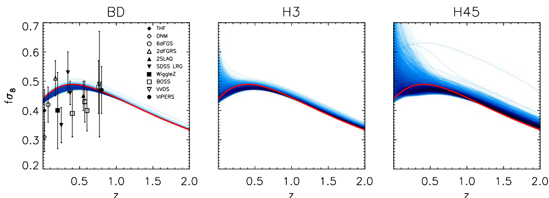
Figure 19: The redshift evolution of f\sigma_8 expected in 10^4 viable EFT models is shown and compared to data. The error bars represent 1\sigma standard deviation. The evolution predicted by the best Planck fit is shown in red.
