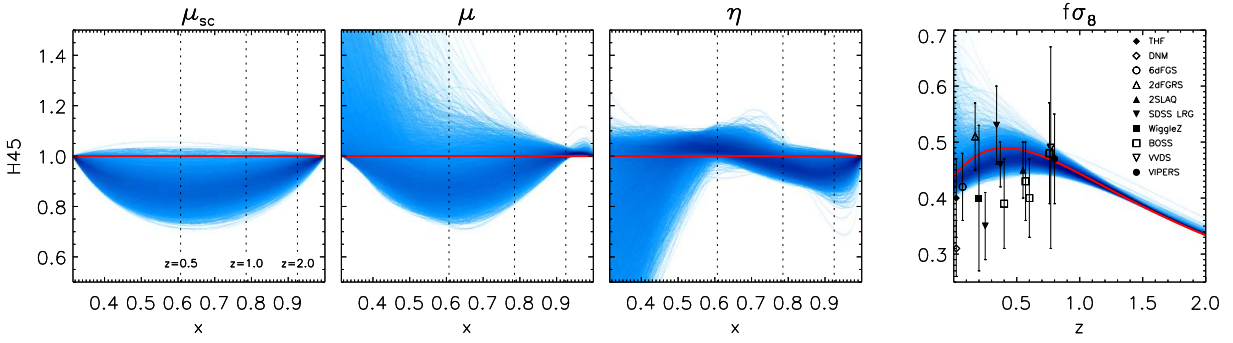
Figure 22: The amplitude of \mu_{\text{sc}} , \mu , \eta as a function of the reduced matter density x and f\sigma_8 as a function of the redshift z for 10^4 viable EFT models where \mu_2^2 is switched on. The expected values of both these functions in a \Lambda CDM cosmology are shown in red. The vertical dotted lines correspond from left to right to z = 0.5 , z = 1 and z = 2 .
