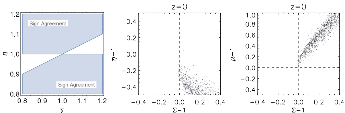
Figure 35: The regions allowing a sign agreement between \mu - 1 and \Sigma - 1 in the (\eta, \Sigma) plane according to (319) is shown in the left panel . In the middle and right panels, the correlations between the LDE models with \mu_2^2 = 0 , c_s < 1 and c_T < 1 are shown in the \mu - 1, \Sigma - 1 and \eta planes at z = 0 .
