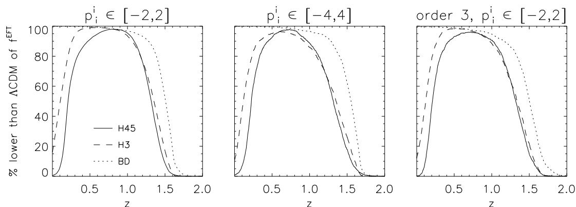
Figure 18: Percentage of randomly generated EFT models with growth rate f lower than that predicted by \Lambda CDM Planck-cosmology as a function of the redshift z . We have checked the robustness of our analysis by changing the interval of the randomly generated expansion coefficients (center) and by augmenting the order of the expansion (right).
