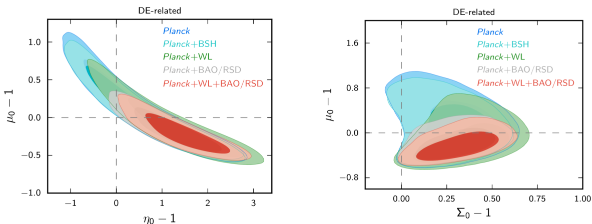
Figure 39: Figures 14 and 15 in [80]. Constraints on the present time value of \mu , \eta and \Sigma parametrised as (338) based on several combination of cosmological probes is shown.
