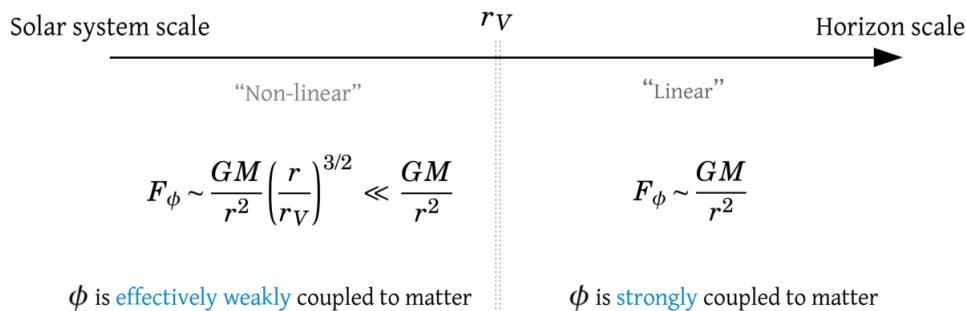
Figure 13: Schematic diagram of the evolution of the screening strength depending on the scale.
